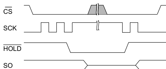
Figure 22. HOLD Operation
