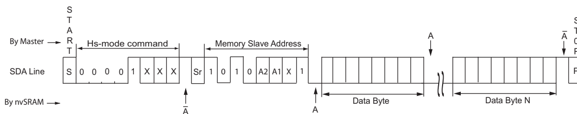
Figure 17. Current Location Multi-Byte nvSRAM Read (Hs-mode)
