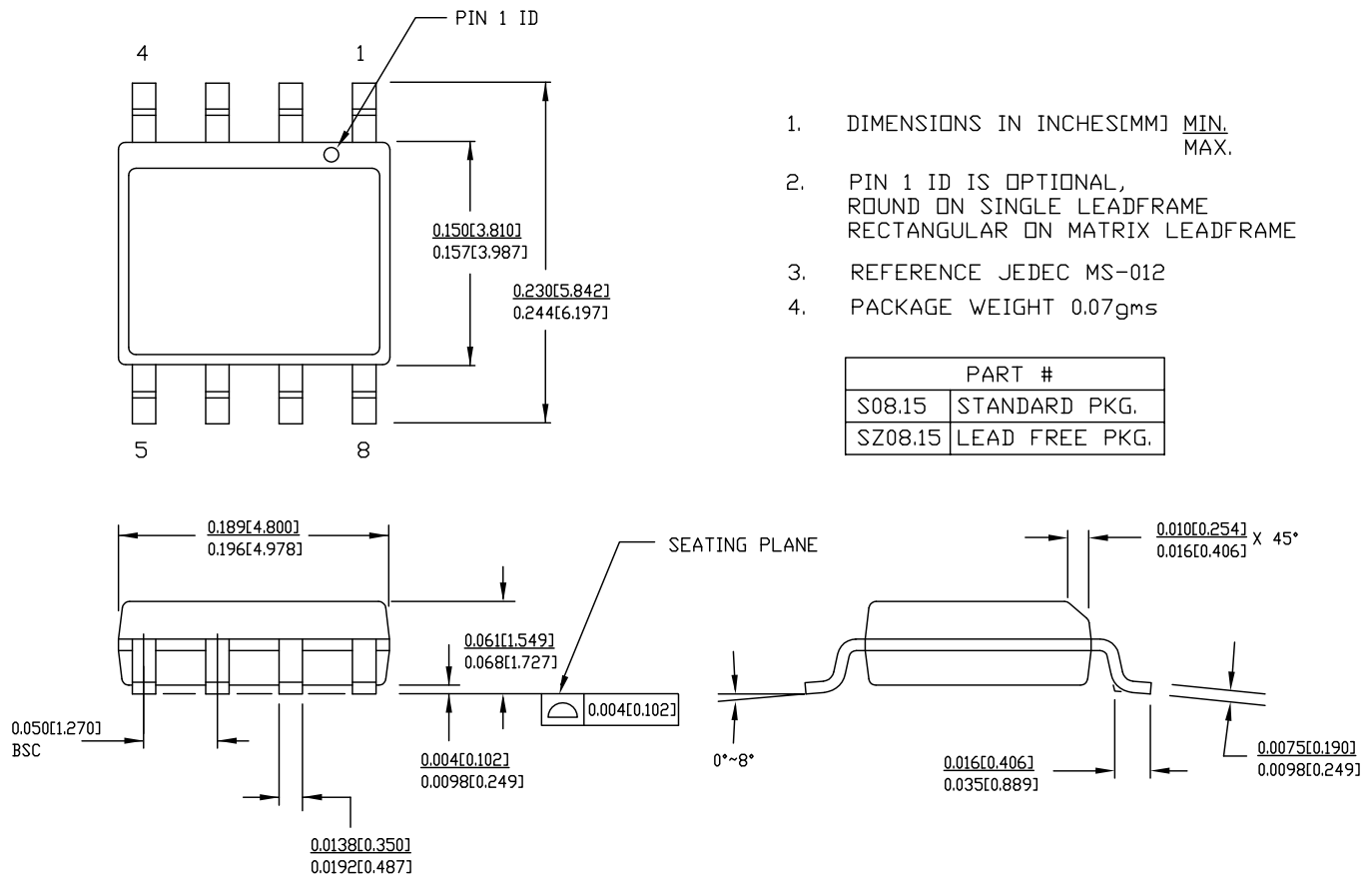
Figure 34. 8-pin SOIC (150 mils) Package Outline, 51-85066
