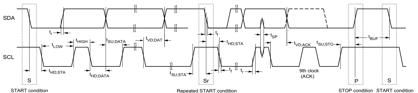
Figure 30. Timing Diagram
