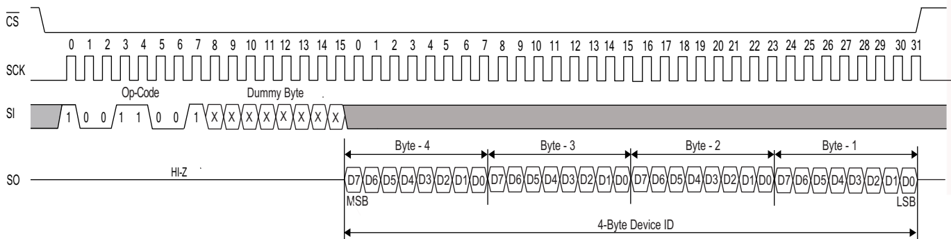
Figure 26. FAST_RDID instruction
