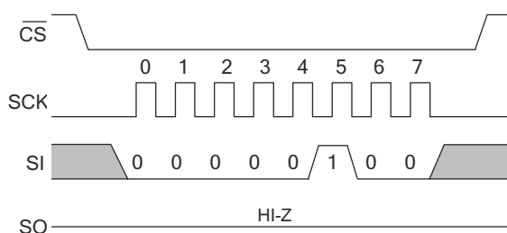
Figure 11. WRDI Instruction
