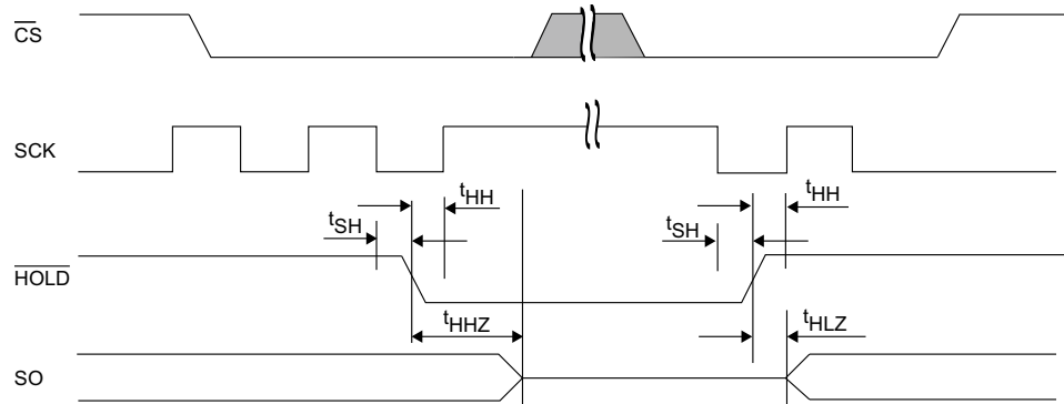
Figure 30. HOLD Timing
