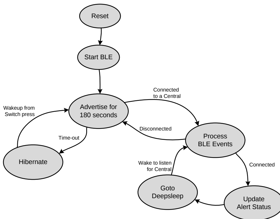
Figure 8. Firmware Flow
