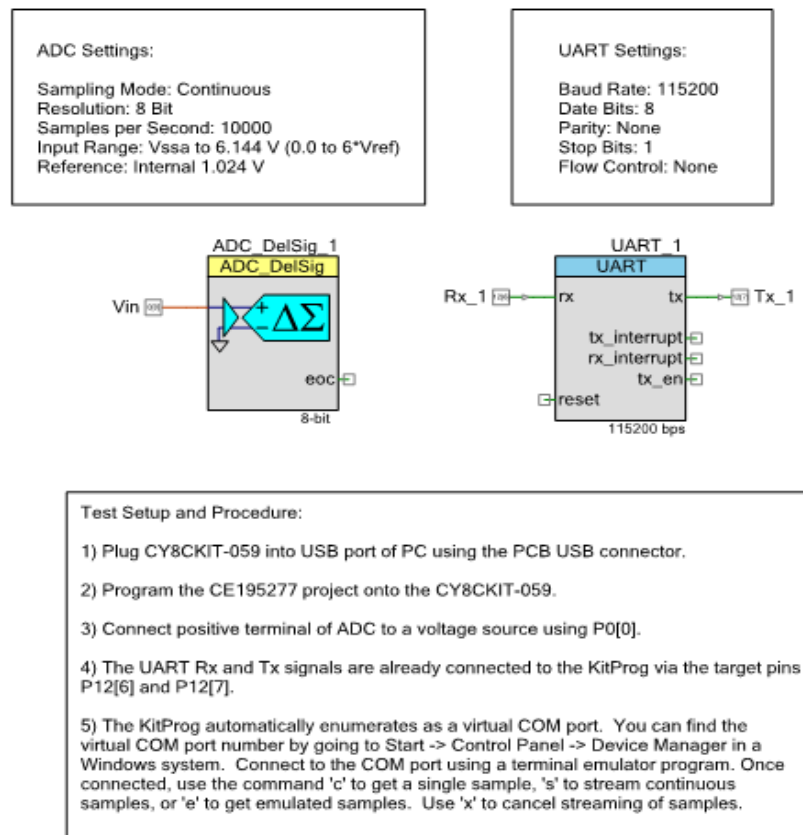
Figure 1. PSoC Creator Schematic of Code Example
