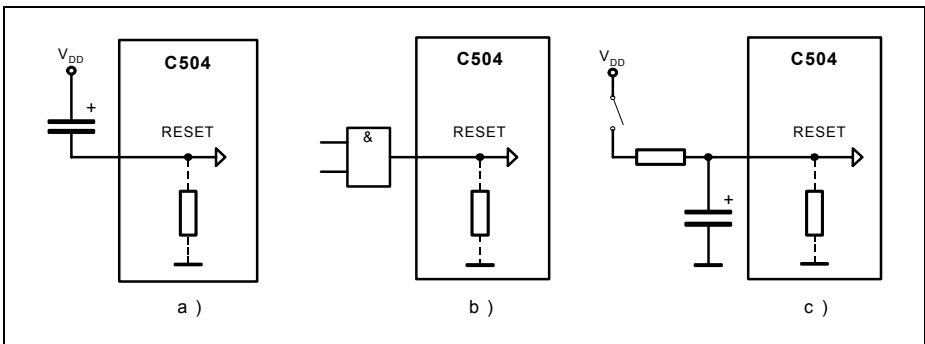
Figure 1 Reset Circuitries
