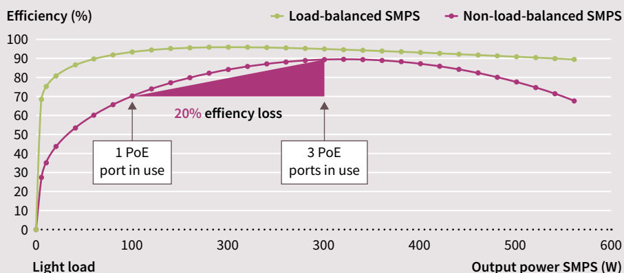
SMPS power sourcing equipment efficiency importance for 802.3bt type 4
