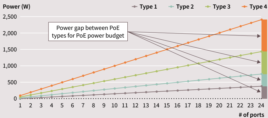
Relative power increase per port and PoE type
