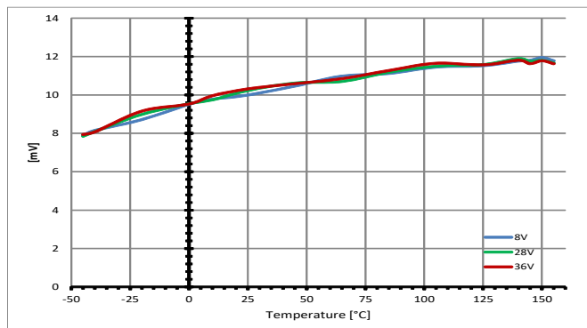
Output Voltage Drop Limitation at Low Load Current V_{DS(NL)} = f(T_J; V_S)
