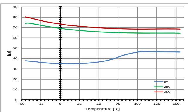
Turn OFF t_{OFF} = f(T_J; V_S), R_L = 4 \Omega
