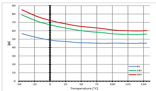
Turn ON t_{ON} = f(T_J; V_S), R_L = 4 \Omega
