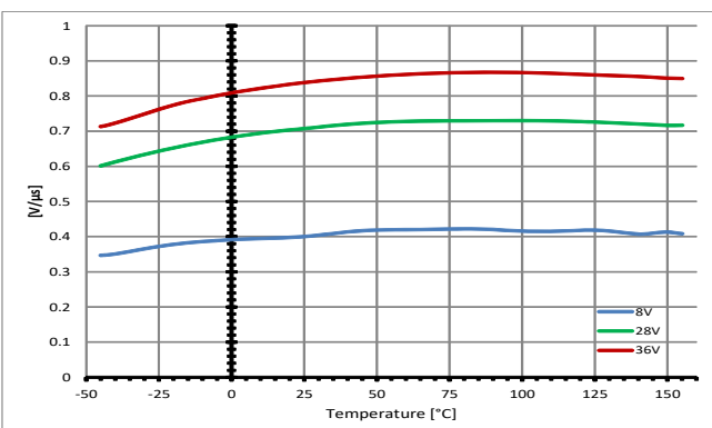
Slew Rate at Turn OFF -dV/dt_{OFF} = f(T_J; V_S), R_L = 4 \Omega
