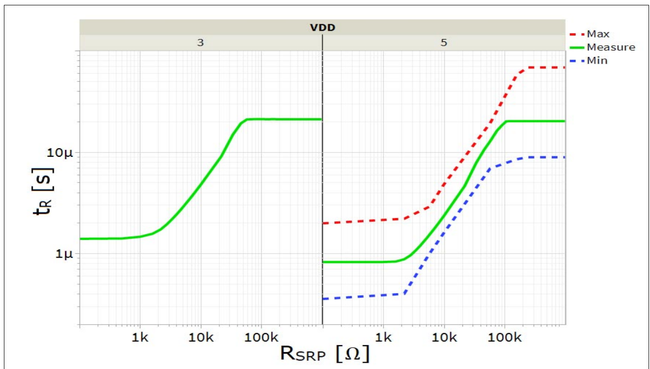
Figure 22 Typical t_R vs. R_{SRP} @ V_{IN}=5V ; V_{DD}=3V, 5V ; V_{BAT}=28V ; R_L=4.7\Omega ; T_J=[-40 \dots 150^{\circ}C]
