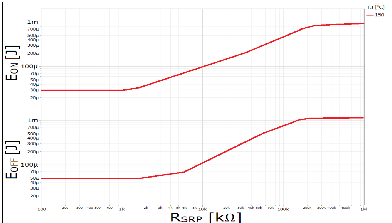
Figure 21 Typical E_{ON} & E_{OFF} vs. SRP @ T_{J(0)}=150^{\circ}C , V_{DD}=5.5V & V_{DD}=3V ; V_{BAT}=28V ; I_N=5V ; STATUS=pulled-up\ to\ V_{DD} ; I_L=I_{L(NOM)}
