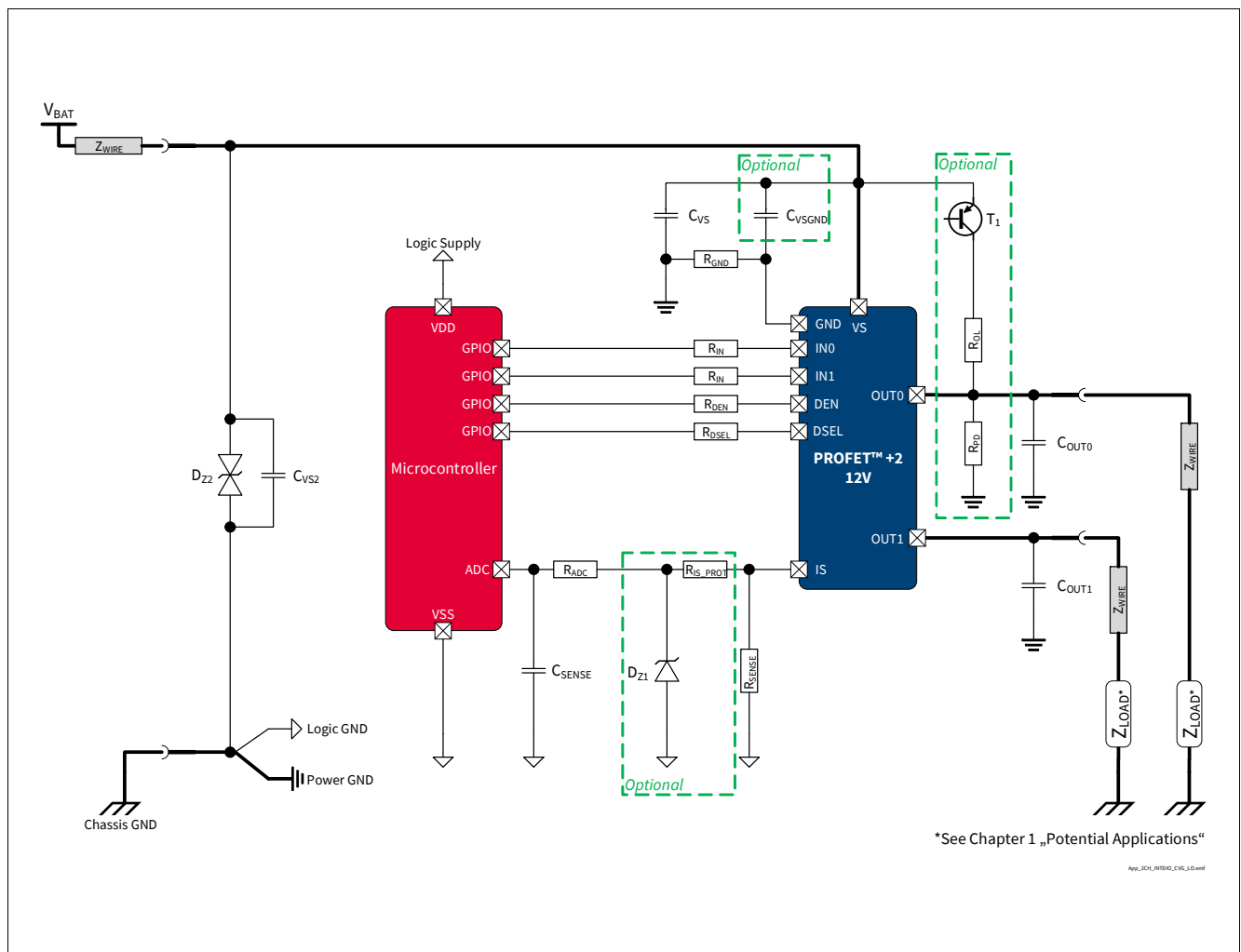
Figure 43 BTS7012-2EPG Application Diagram
