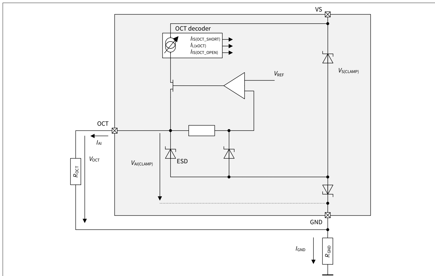
The device recognizes an OCT pin short if the current between the OCT pin and GND is higher than I_{OCT\_SHORT} . In this case the overcurrent threshold is internally set to the highest configurable overcurrent threshold I_{L(HOCT)} . Additionally, a sense current of I_{S(OCT\_SHORT)} is sent out at the IS pin when the sequential diagnosis address #4 is selected.
