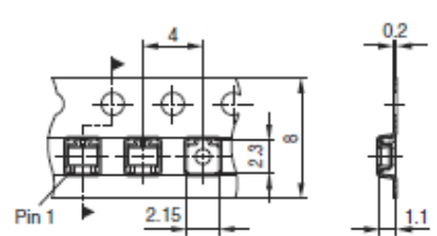
Figure 1 Outline PG-SOT323, dimensions in mm
