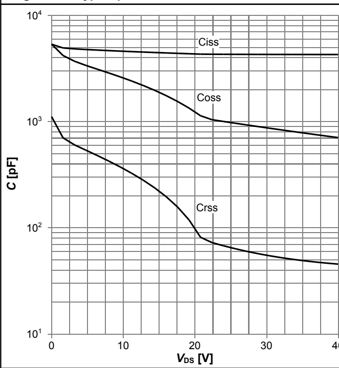
Diagram 11: Typ. capacitances
