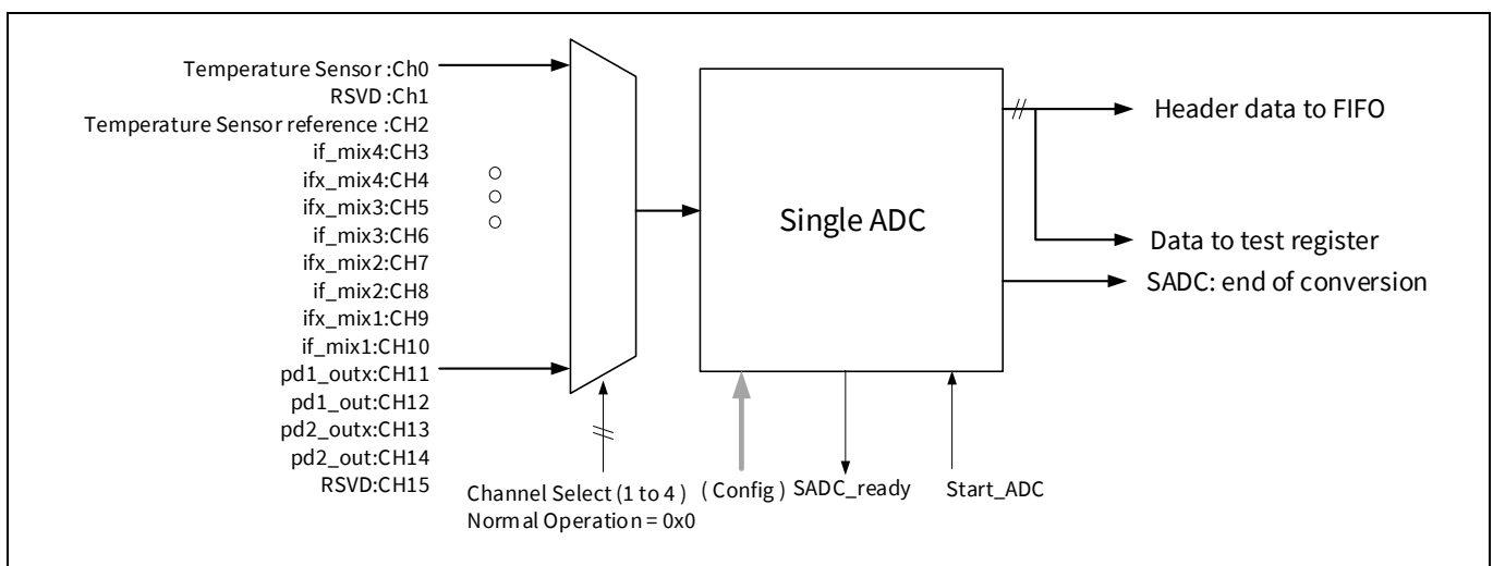
Figure 79 SADC Integration
