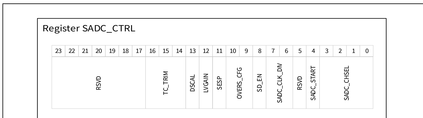
Figure 27 SADC_CTRL registers
