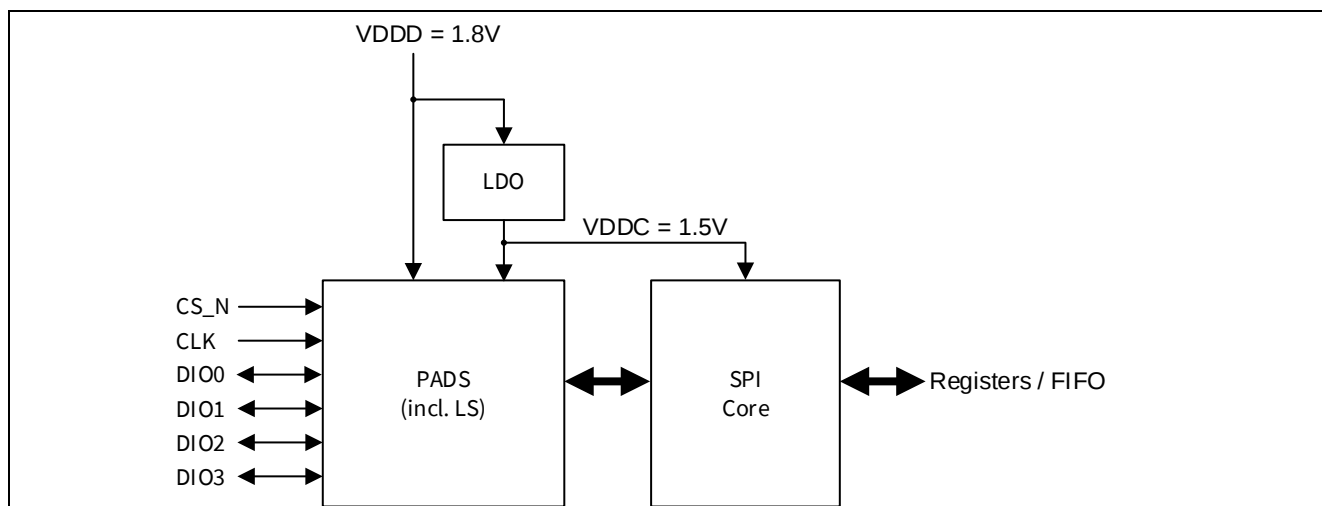
Figure 48 SPI module
