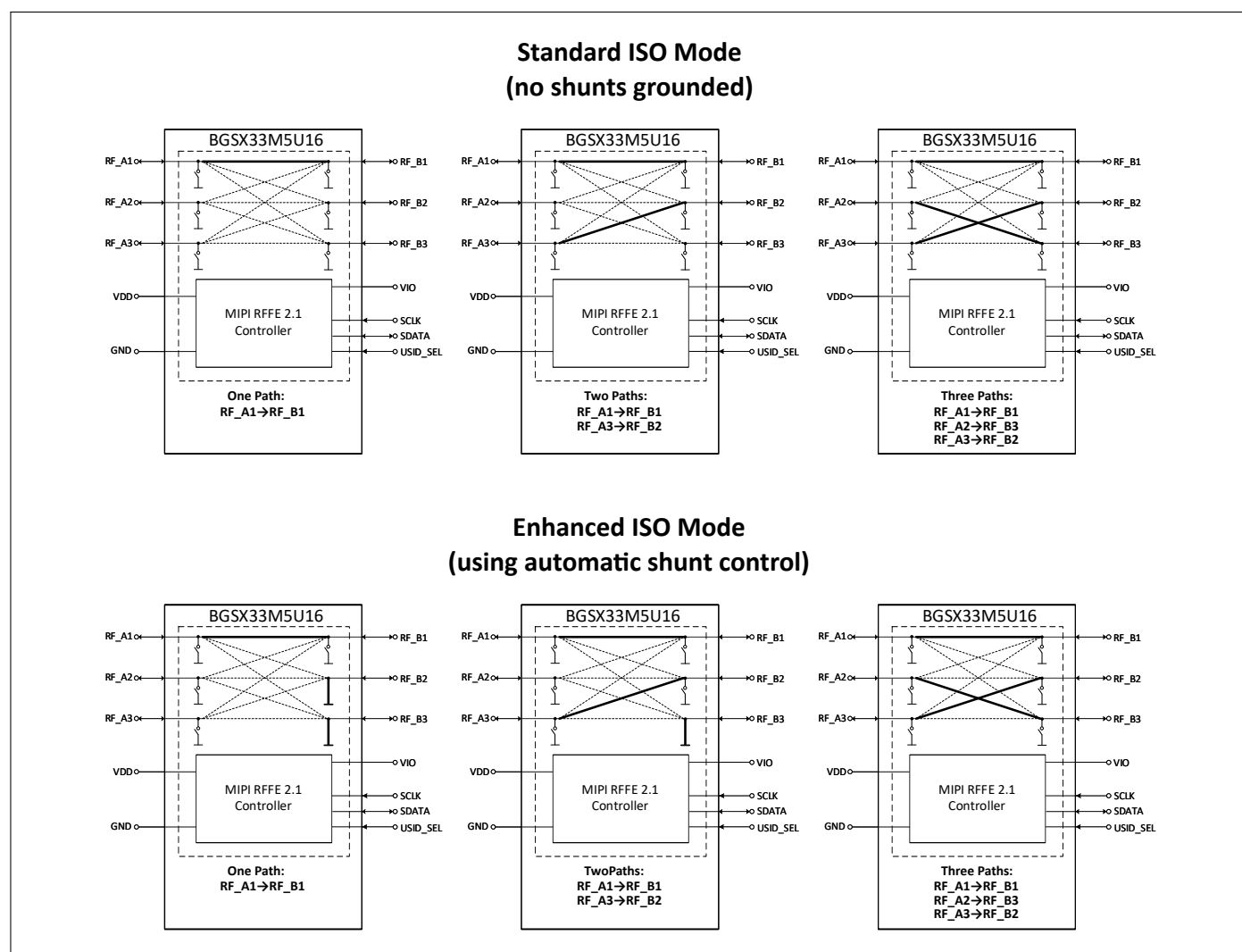
Figure 2: Examples for standard vs. enhanced isolation modes
