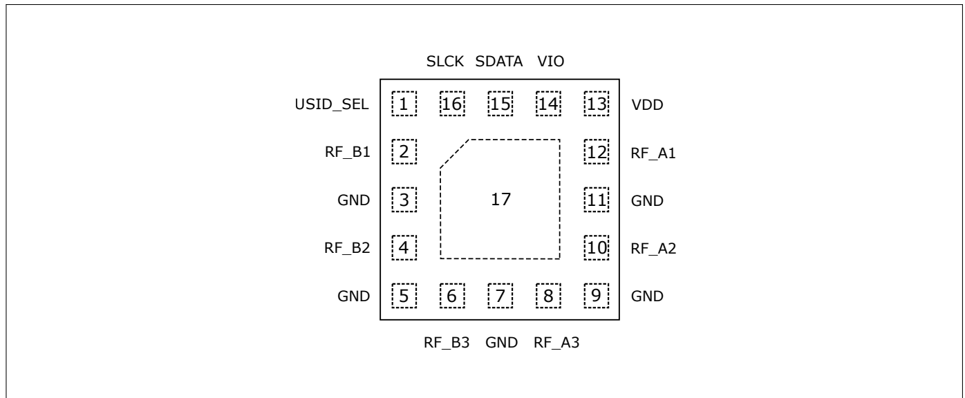
Figure 3: Footprint (top view)
