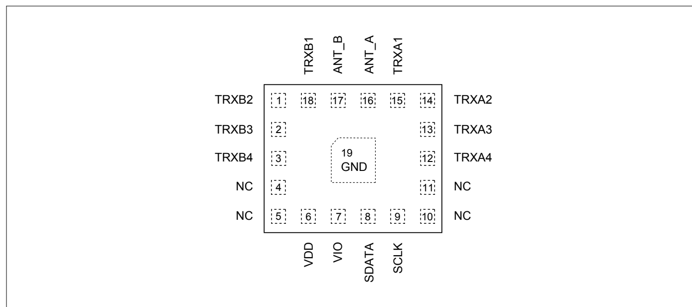
Figure 3: BGSX28MA18 Pin Configuration (top view)
