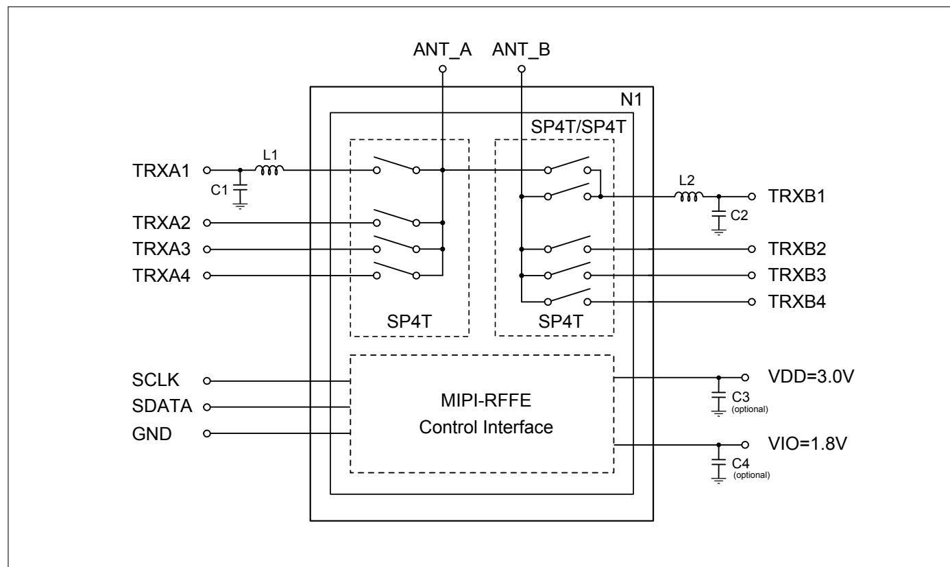
Figure 2: BGSX28MA18 Application Schematic
