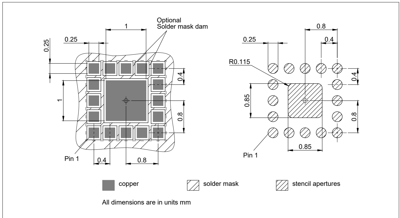
Figure 5: Footprint Recommendation
