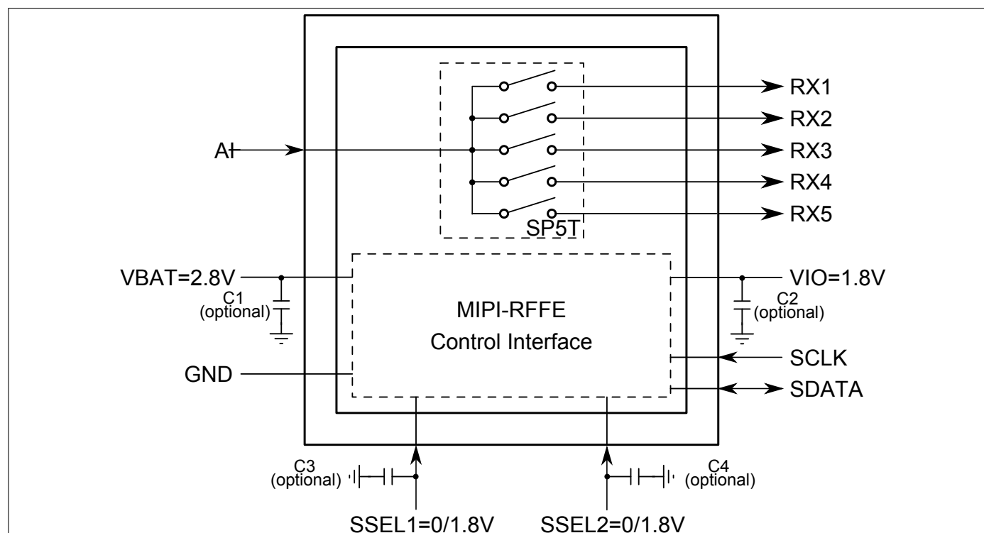
Figure 10: BGS15MA12 Application Schematic
