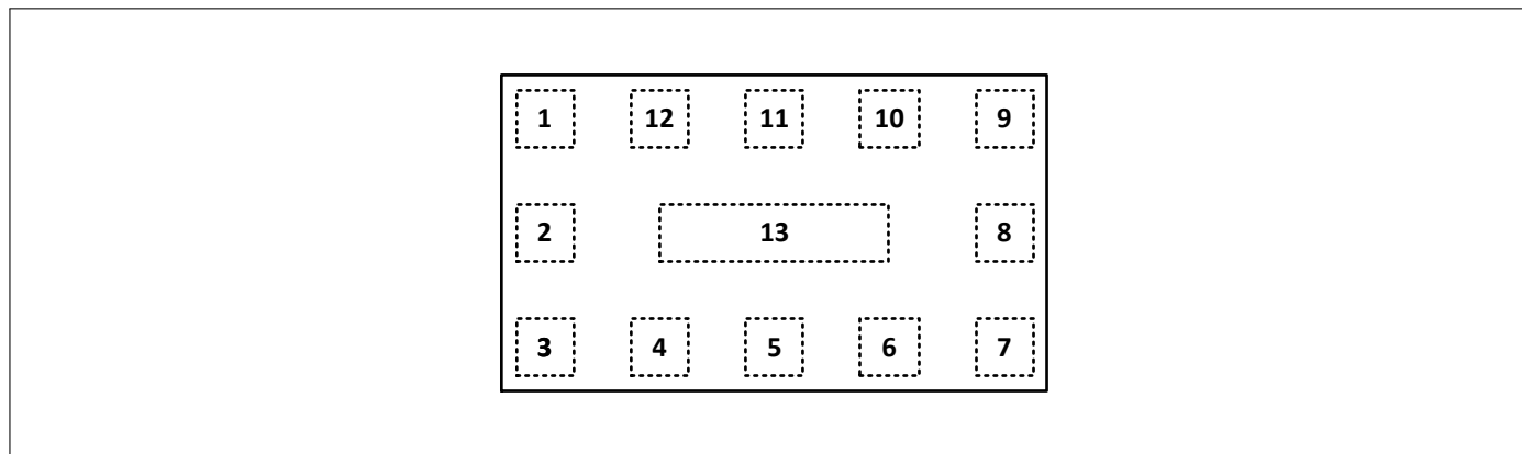
Figure 9: BGS15MA12 Pin Configuration (top view)
