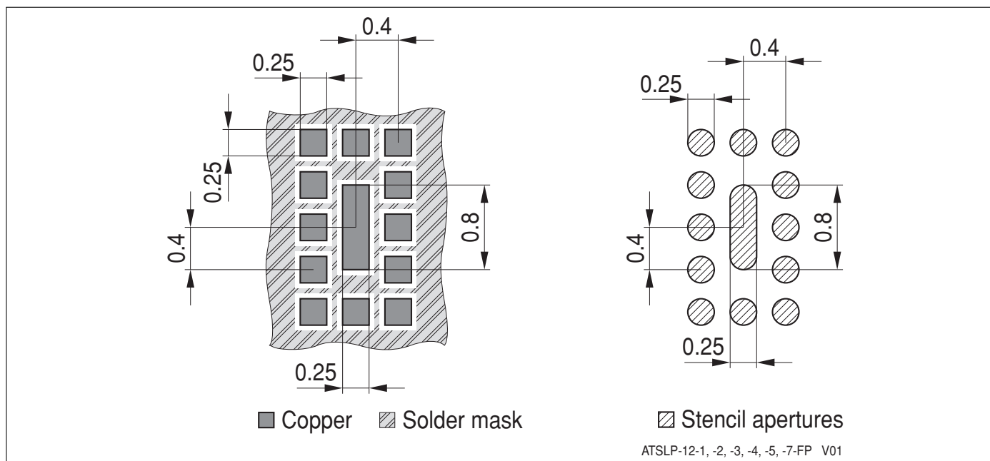
Figure 13: Footprint Recommendation
