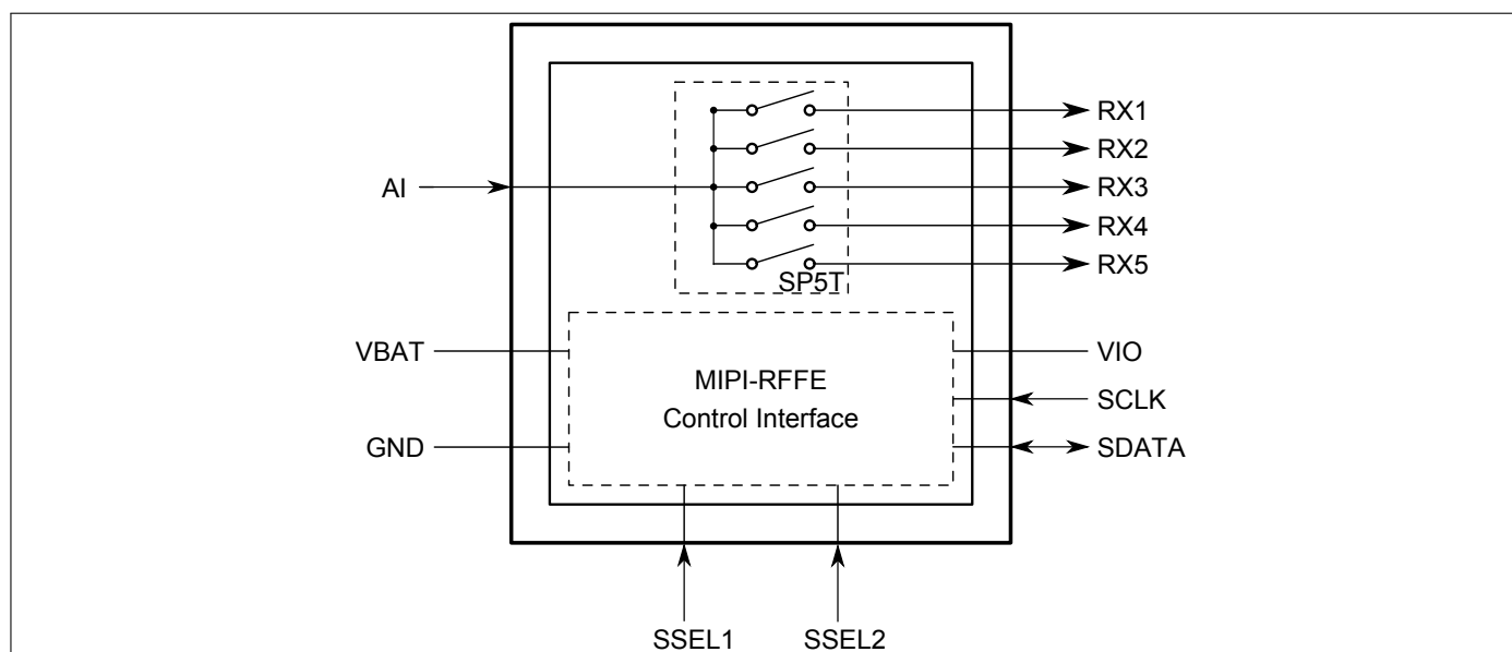
Figure 1: BGS15MA12 Block diagram
