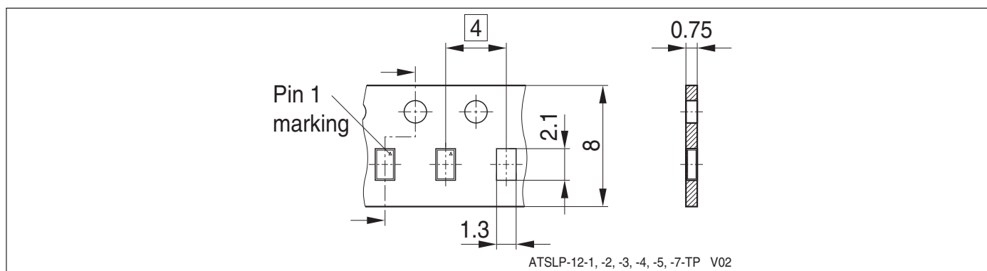
Figure 14: ATSLP-12-4 Carrier Tape
