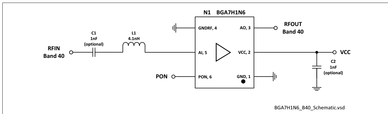
Figure 3 Application Schematic BGA7H1N6
