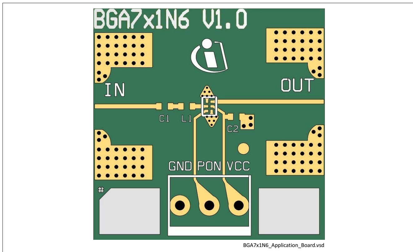
Figure 4 Drawing of Application Board
