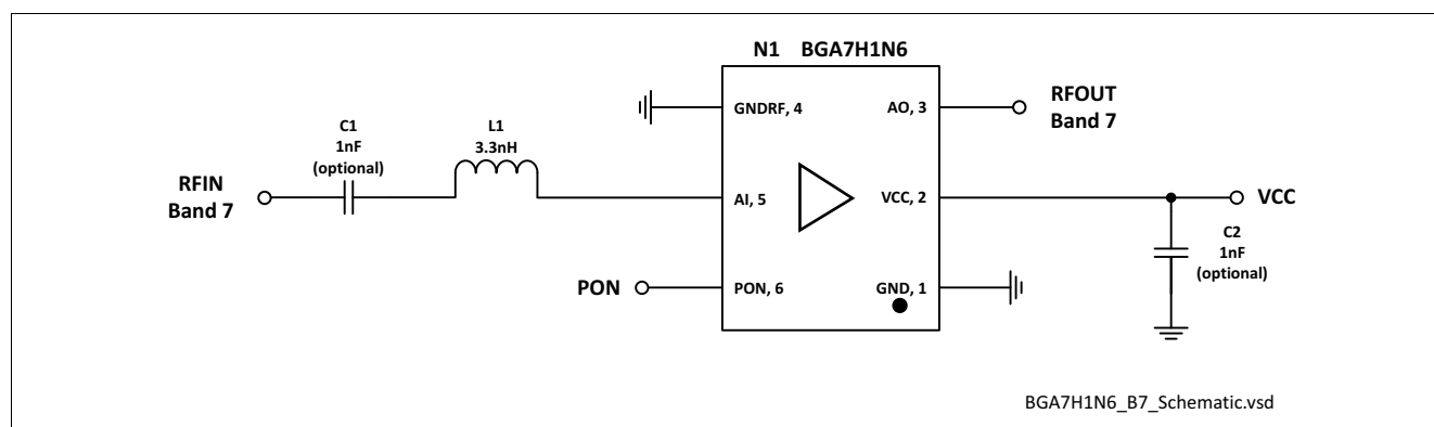
Figure 2 Application Schematic BGA7H1N6
