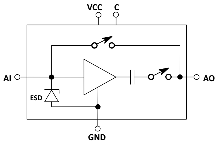
BGA5M1BN6_Blockdiagram.vsd
