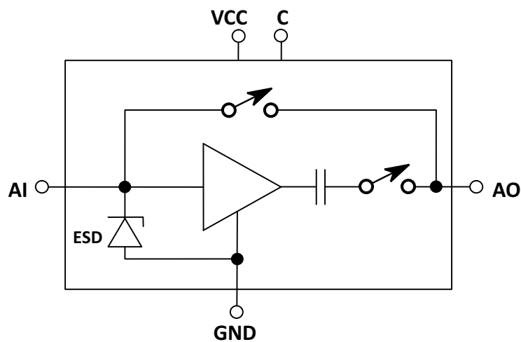
BGA5L1BN6_Blockdiagram.vsd
