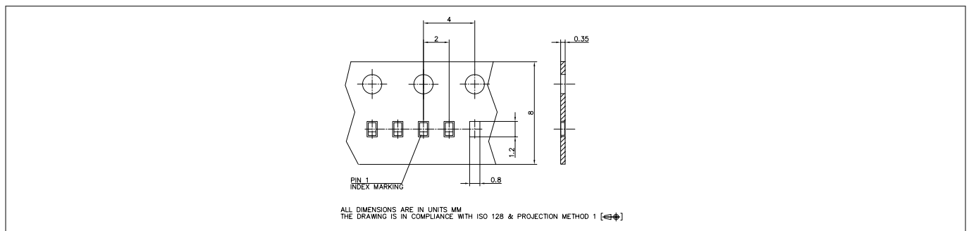
Figure 25 Tape dimensions
