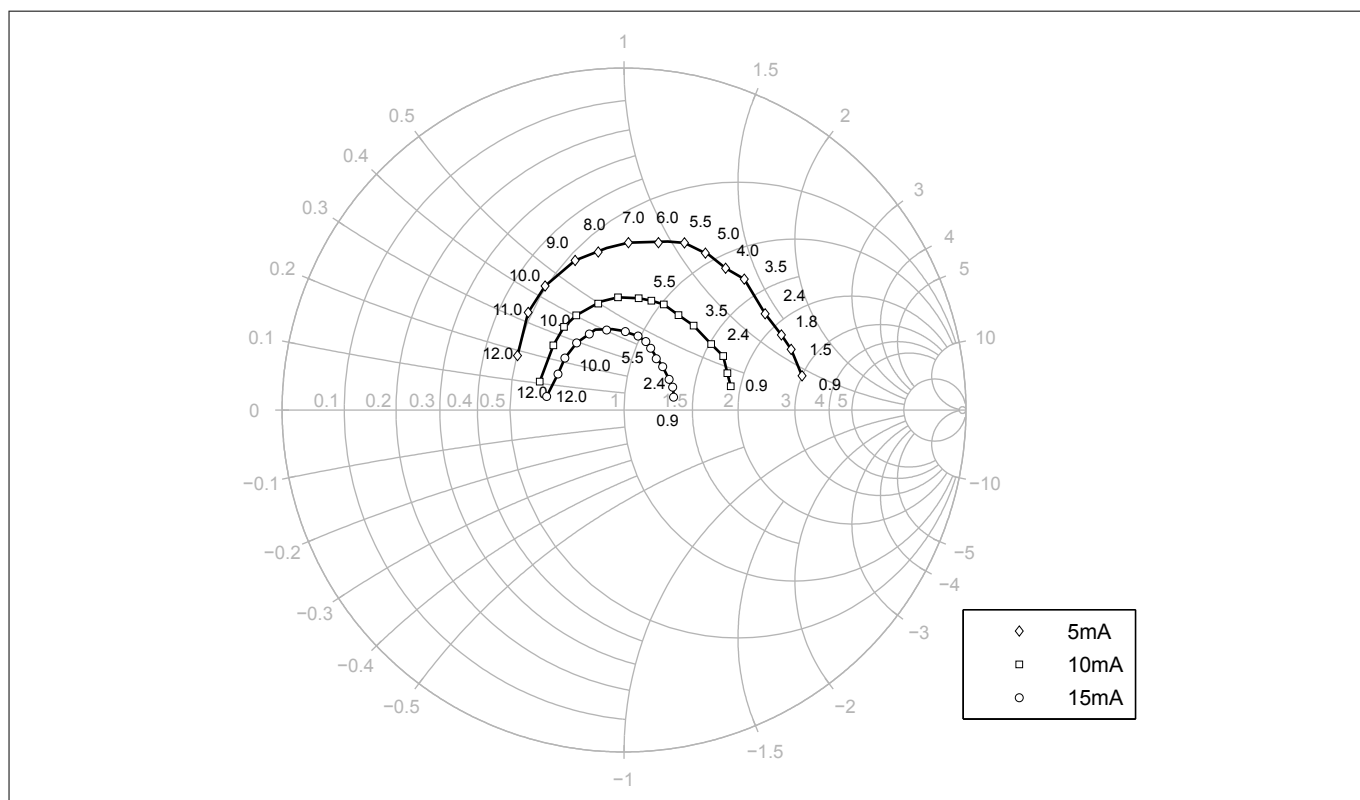
Figure 17 Source impedance for minimum noise figure Z_{s,opt} = f(f) , V_{CE} = 1.8 V, I_C = 5 / 10 / 15 mA
