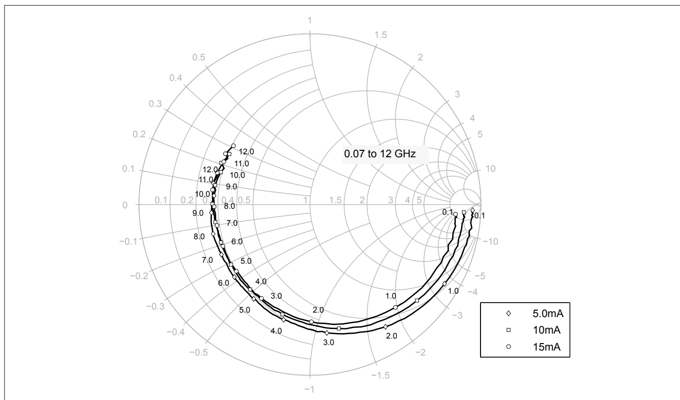
Figure 16 Input reflection coefficient S_{11} = f(f) , V_{CE} = 1.8 V, I_C = 5 / 10 / 15 mA
