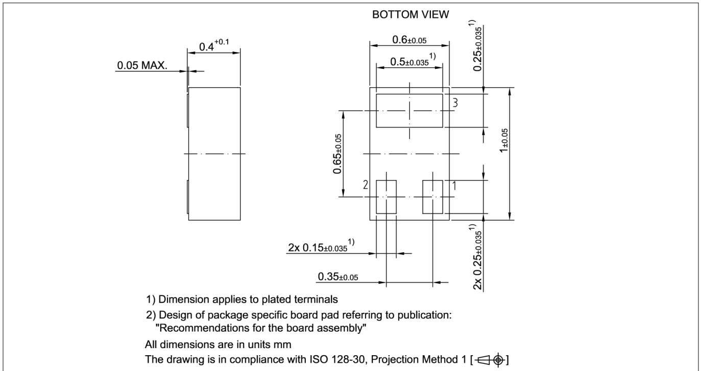
Figure 8 TSLP-3-1 package
