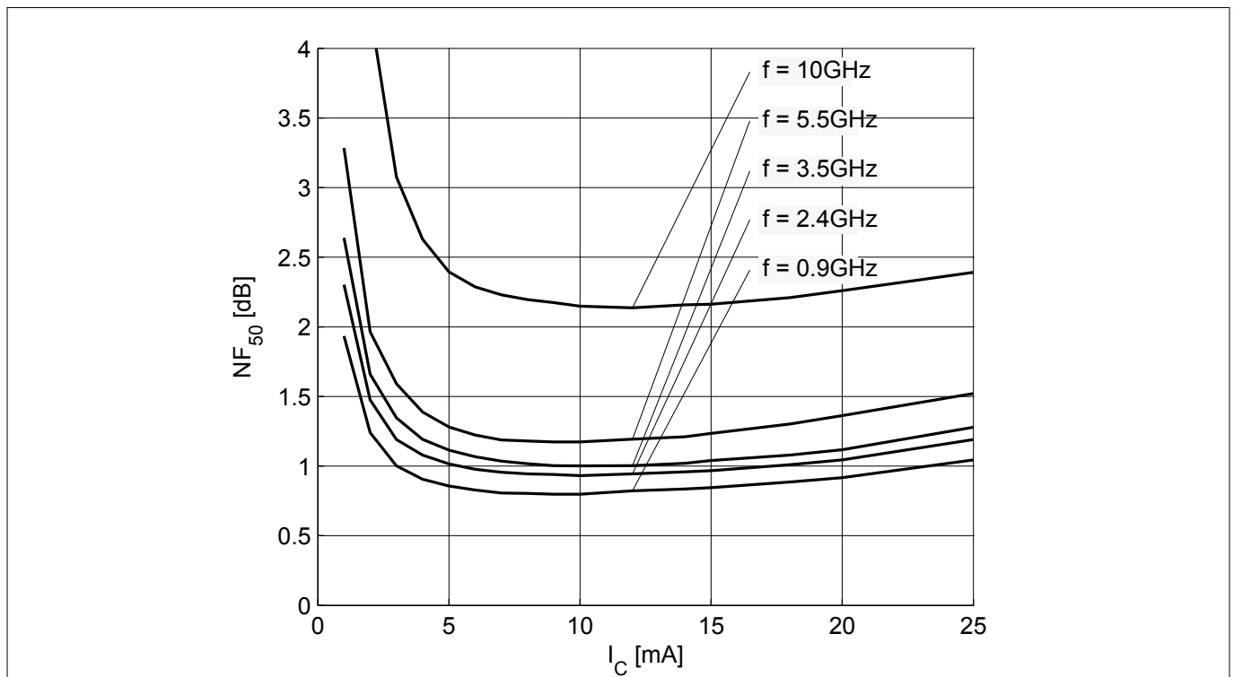
Figure 19 Noise figure NF_{50} = f(I_C) , V_{CE} = 1.8 V, Z_S = 50 \Omega , f = parameter in GHz
