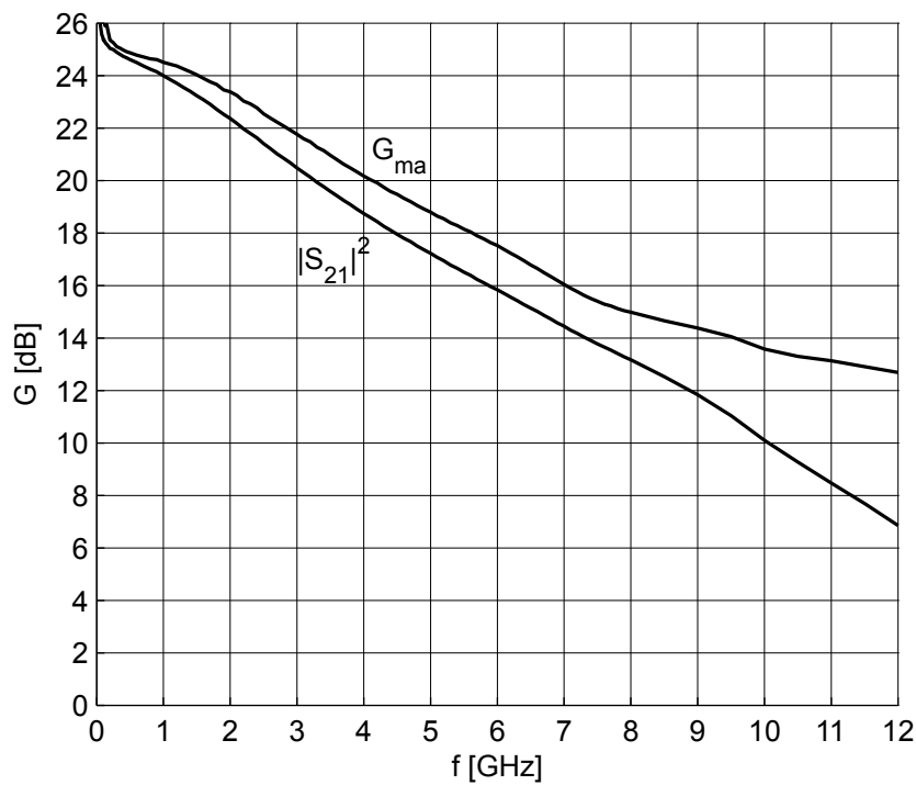
Figure 11 Gain G_{ma} , G_{ms} , |S_{21}|^2 = f(f) , V_{CE} = 1.8 V , I_C = 15 mA
