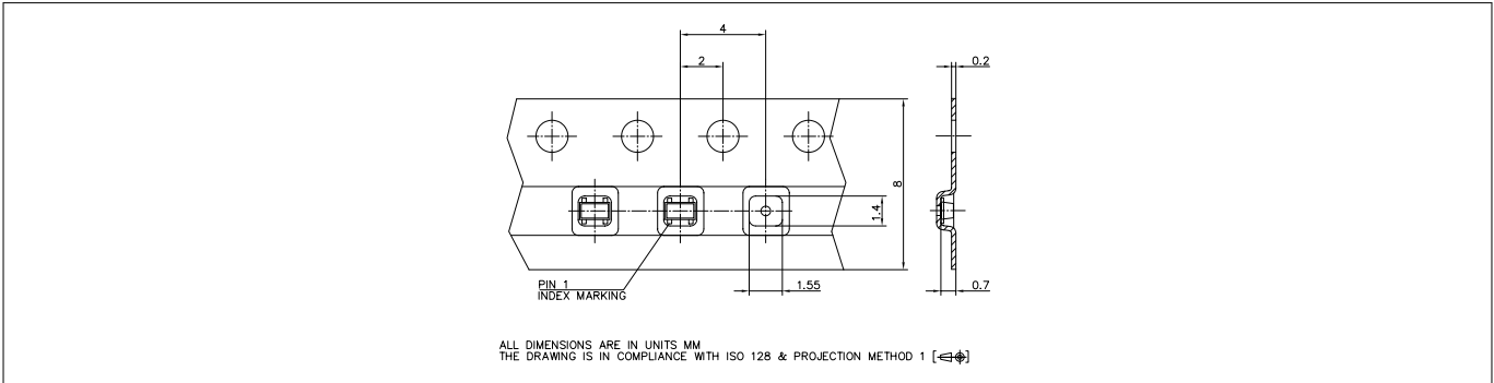
Figure 23 Tape dimensions
