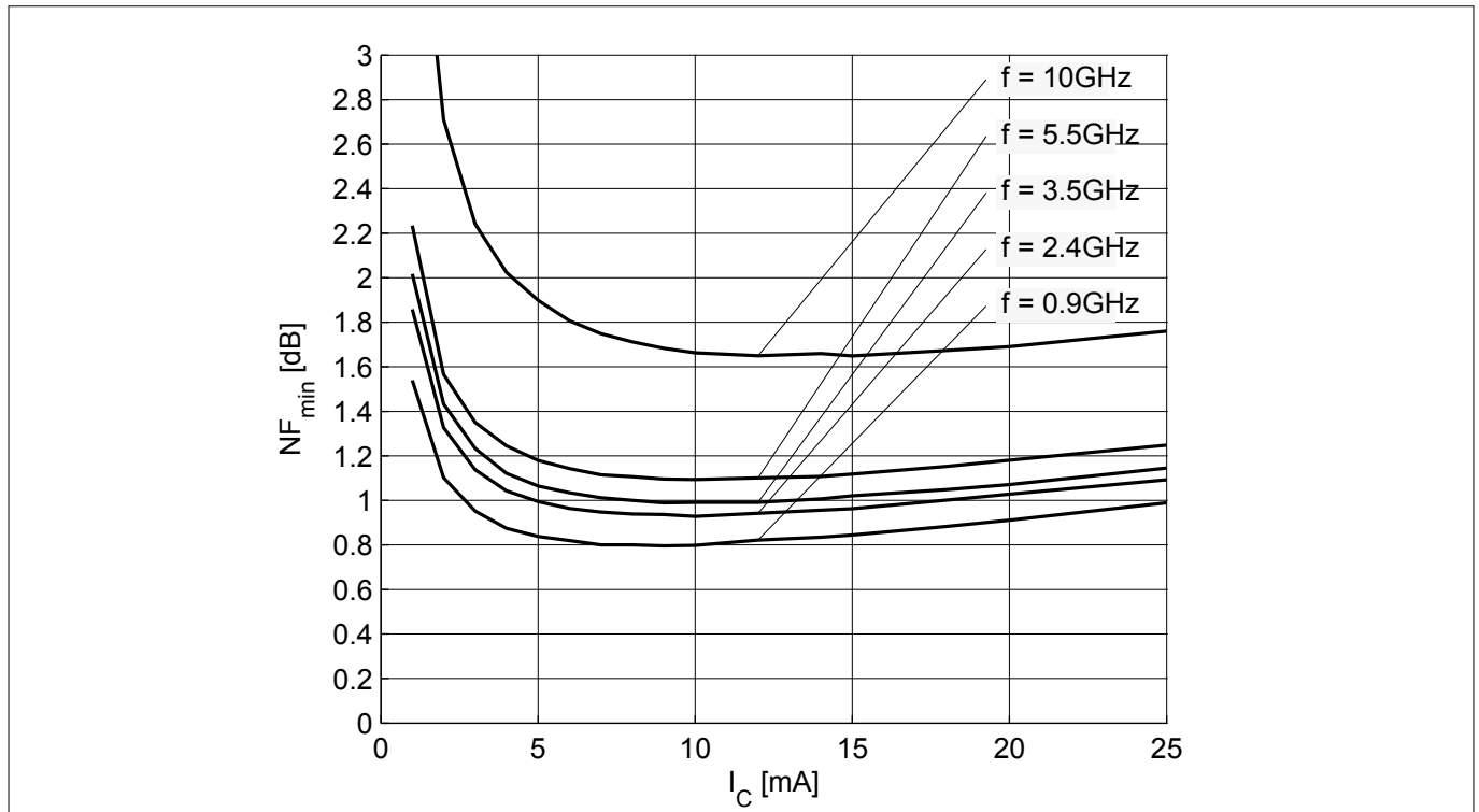
Figure 18 Noise figure NF_{min} = f(I_C) , V_{CE} = 1.8 V, Z_S = Z_{S,opt} , f = parameter in GHz
