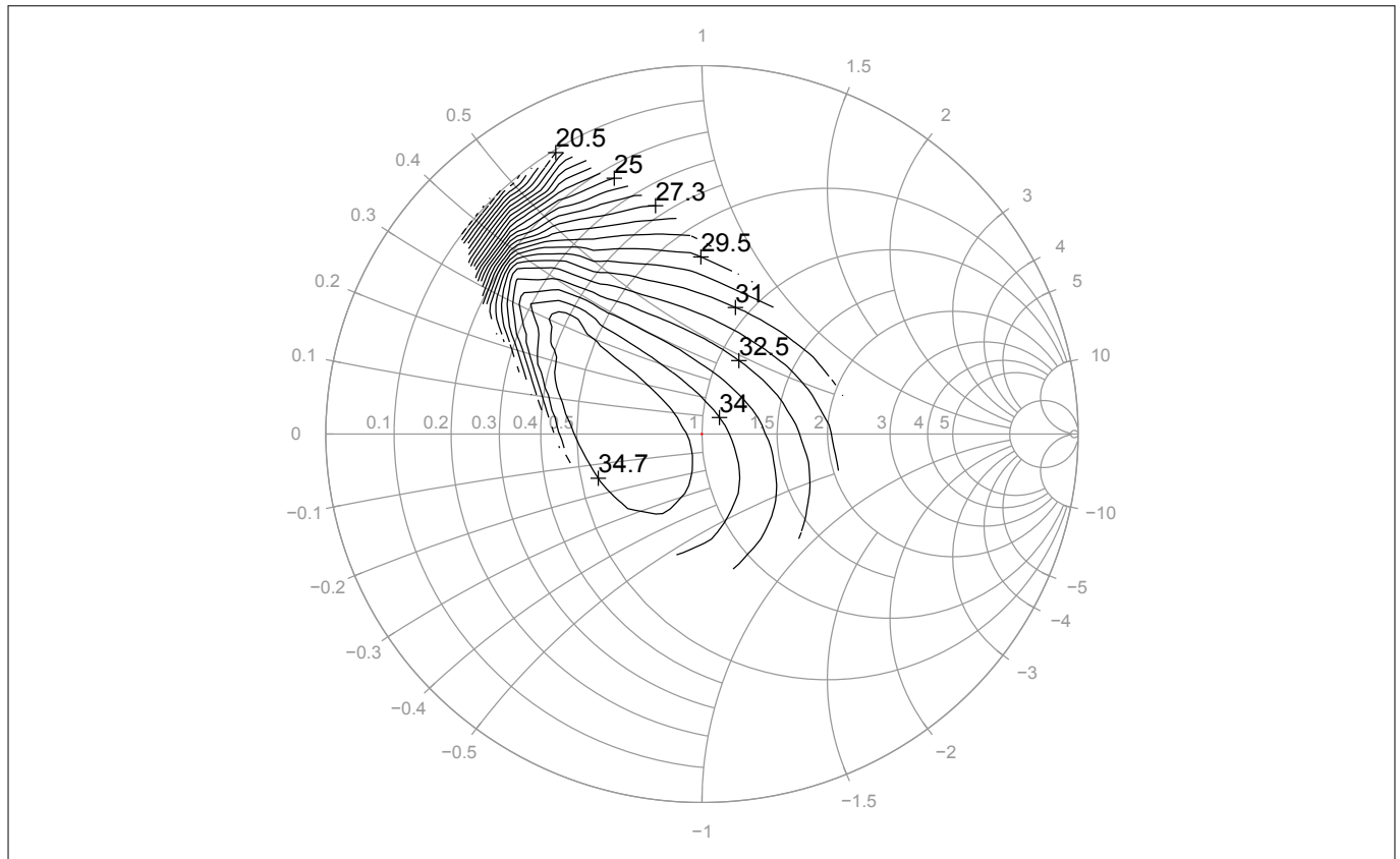
Figure 18 Load pull contour OIP_3 [dBm], V_{CE} = 5 V, I_C = 90 mA, f = 900 MHz
