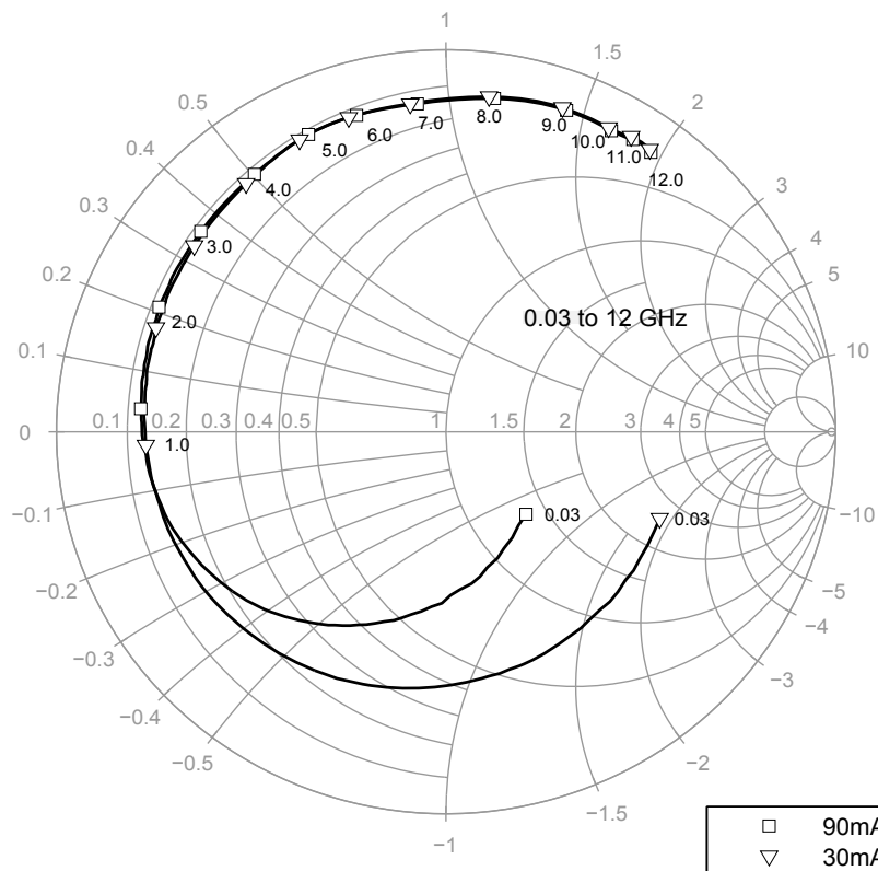
Figure 11 Input reflection coefficient S_{11} = f(f) , V_{CE} = 5 \text{ V} , I_C = \text{parameter}
