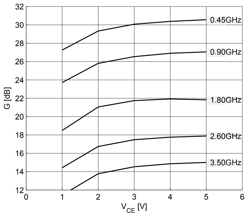
Figure 10 Maximum power gain G_{max} = f(V_{CE}) , I_C = 90 \text{ mA} , f = \text{parameter}
