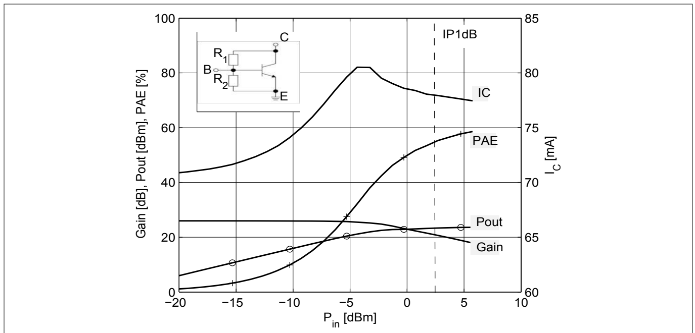
Figure 19 P_{out} , Gain , I_C , PAE = f(P_{in}) , V_{CE} = 5 V, f = 900 MHz, R_1 = 270 \Omega , R_2 = 8 \text{ k}\Omega , Z_L = Z_{L,opt}(P_{out})
