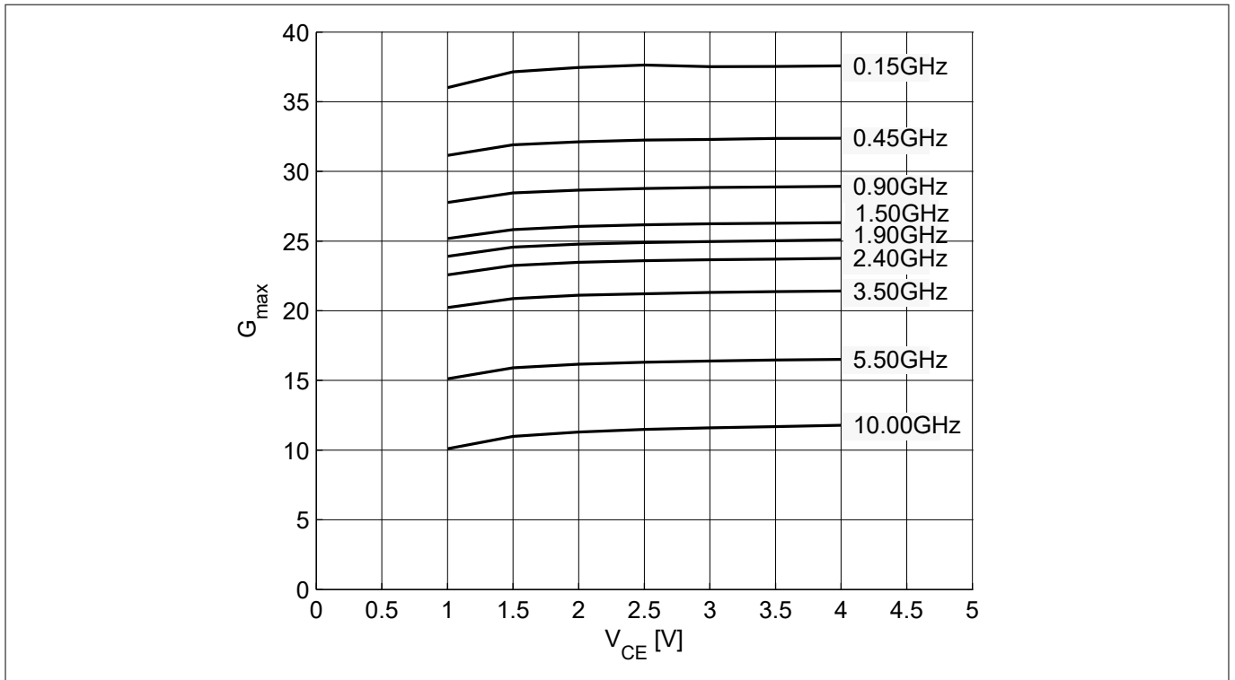
Figure 12 Maximum power gain G_{max} = f(V_{CE}) , I_C = 30 \text{ mA} , f = \text{parameter in GHz}
