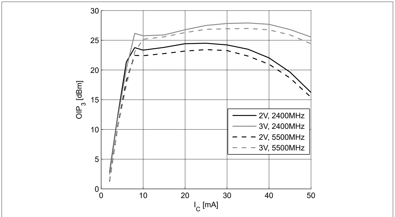
Figure 13 3rd order intercept point at output OIP_3 = f(I_C) , Z_S = Z_L = 50 \Omega , V_{CE} , f = \text{parameters}
