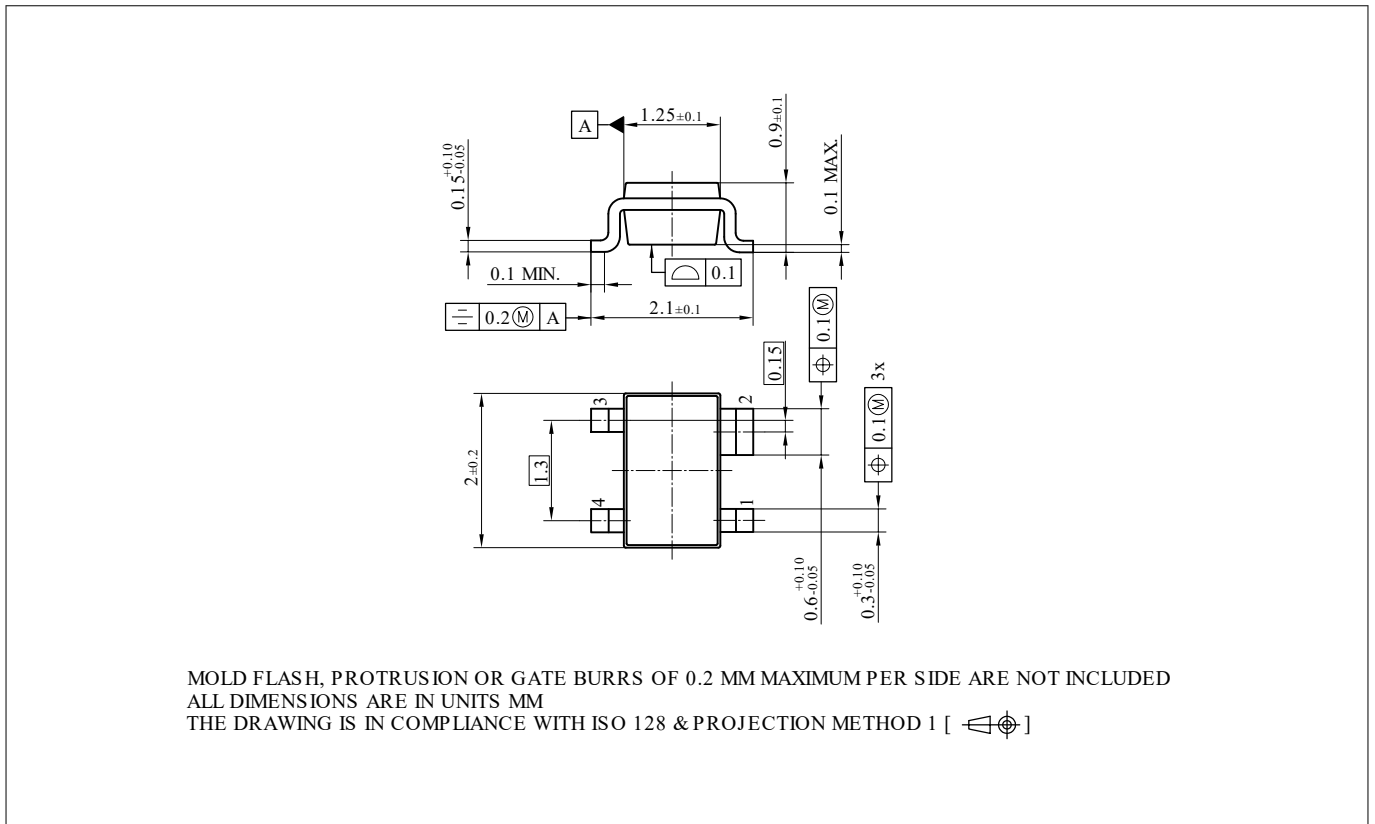
Figure 22 SOT343 package
