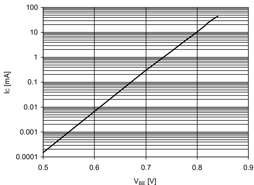
Figure 5 Collector current vs. base emitter voltage I_C = f(V_{BE}) , V_{CE} = 2 V
