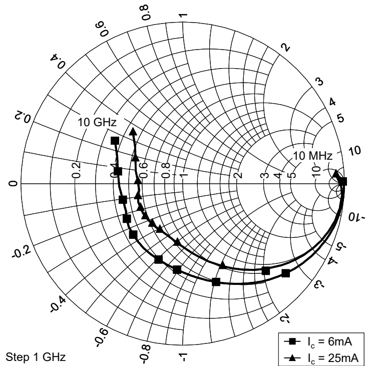
Figure 16 Output reflection coefficient S_{22} = f(f) , V_{CE} = 3\text{ V} , I_C = 6 / 25\text{ mA}
