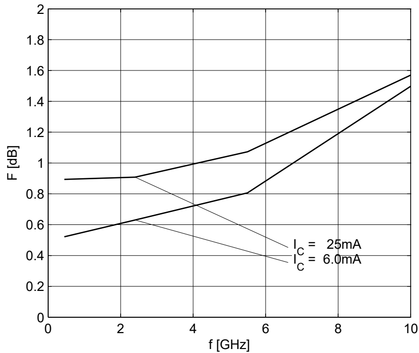
Figure 17 Noise figure NF_{min} = f(f) , V_{CE} = 3\text{ V} , Z_S = Z_{S,opt} , I_C = 6 / 25\text{ mA}
