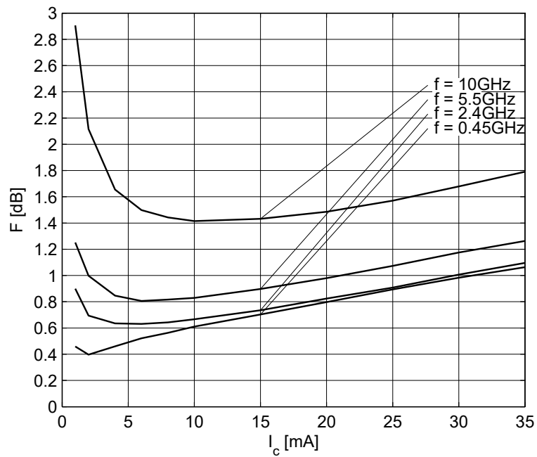
Figure 18 Noise figure NF_{\min} = f(I_c) , V_{CE} = 3\text{ V} , Z_S = Z_{S,\text{opt}} , f = \text{parameter in GHz}
