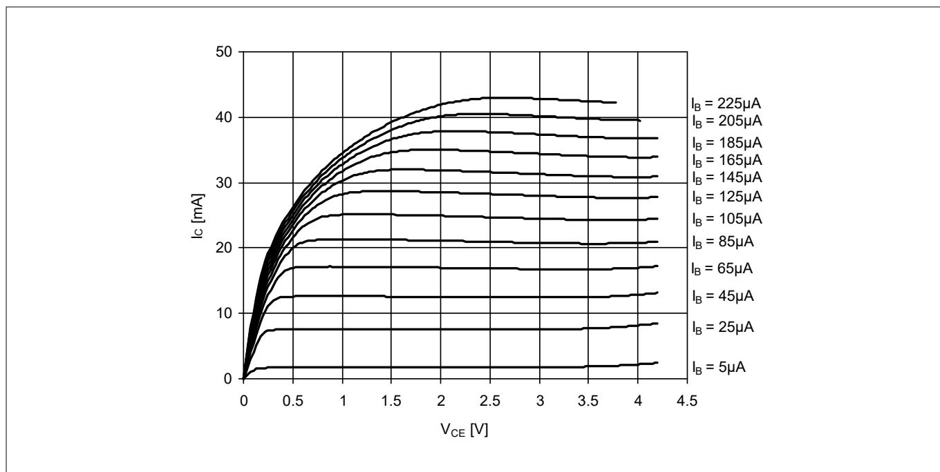
Figure 3 Collector current vs. collector emitter voltage I_C = f(V_{CE}) , I_B = parameter
