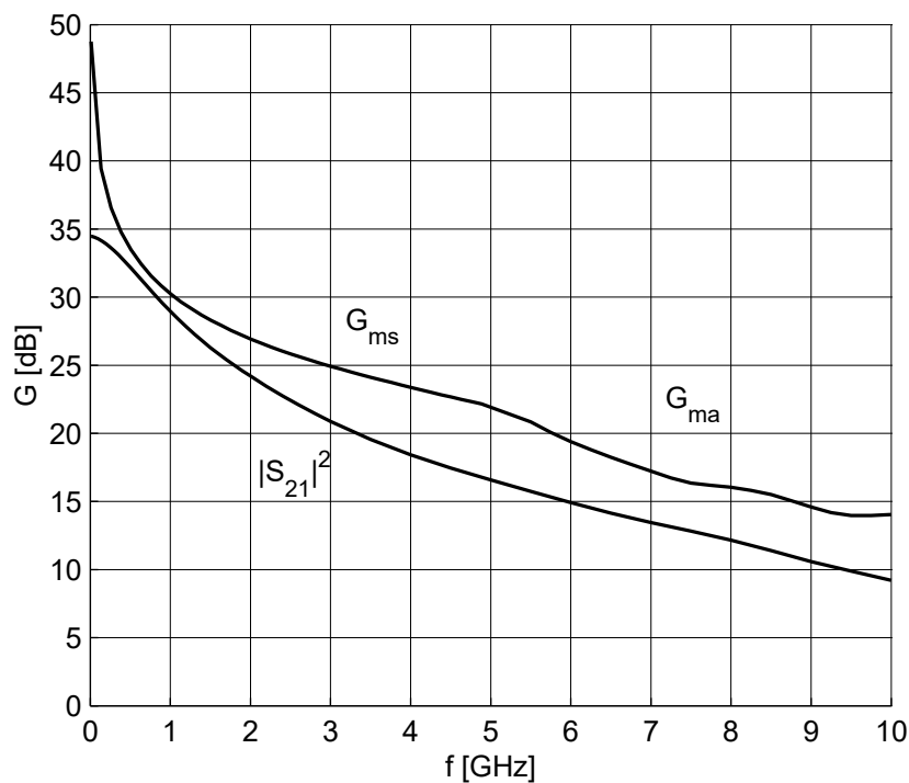
Figure 11 Gain G_{ma} , G_{ms} , |S_{21}|^2 = f(f) , V_{CE} = 3 V, I_C = 25 mA
