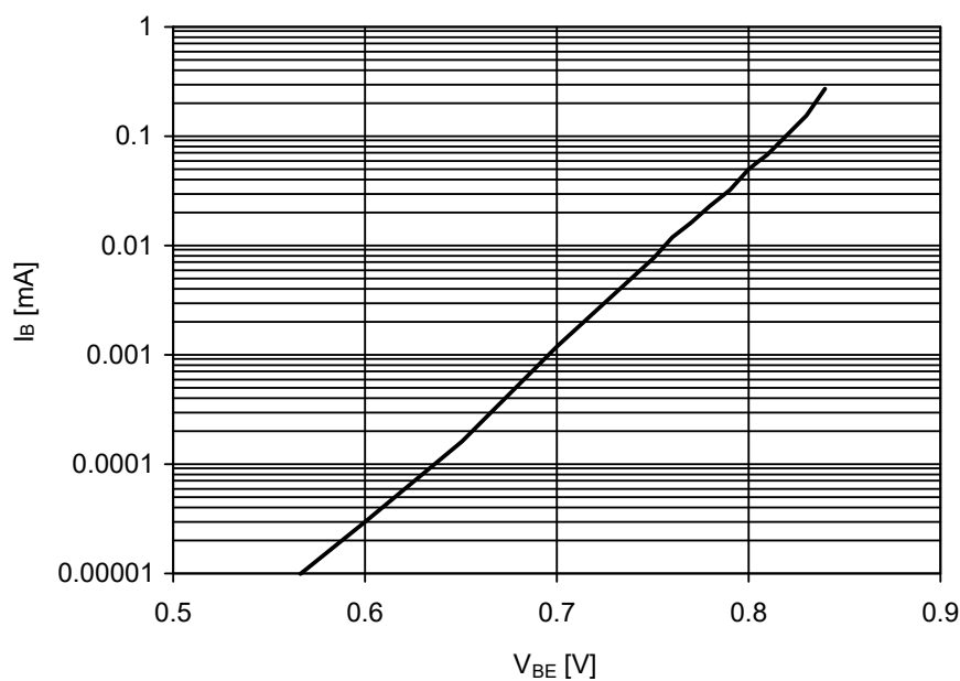
Figure 6 Base current vs. base emitter forward voltage I_B = f(V_{BE}) , V_{CE} = 2 V
