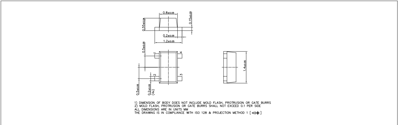
Figure 22 Package outline
