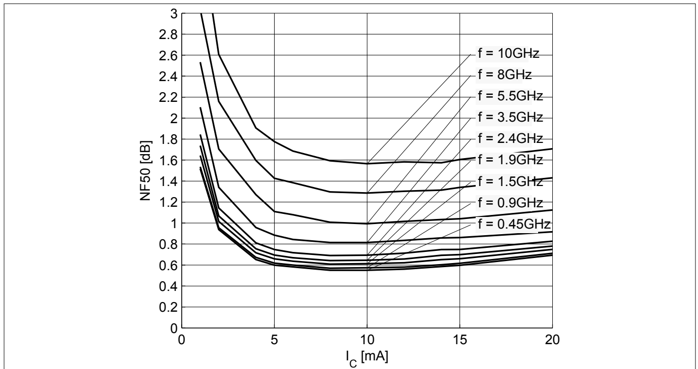
Figure 21 Noise figure NF_{50} = f(I_C) , V_{CE} = 3\text{ V} , Z_S = 50\ \Omega , f = \text{parameter in GHz}
