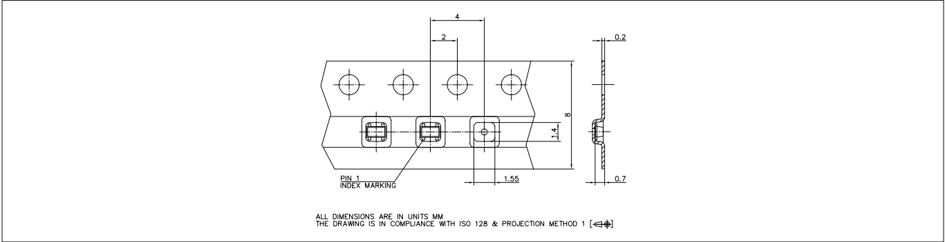
Figure 25 Tape dimensions
