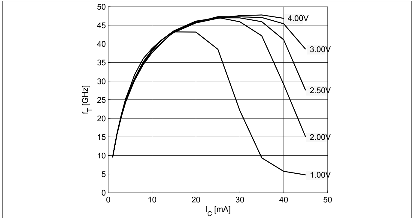
Figure 8 Transition frequency f_T = f(I_C) , f = 2 GHz, V_{CE} = \text{parameter}
