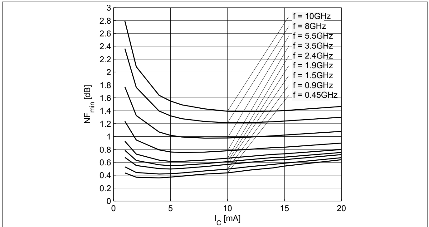
Figure 20 Noise figure NF_{min} = f(I_C) , V_{CE} = 3\text{ V} , Z_S = Z_{S,opt} , f = \text{parameter in GHz}
