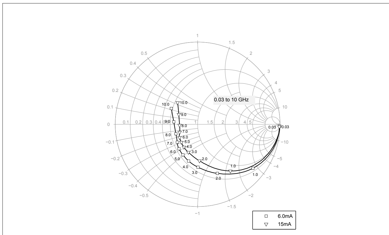
Figure 17 Output reflection coefficient S_{22} = f(f) , V_{CE} = 3 V, I_C = 6 / 15 mA
