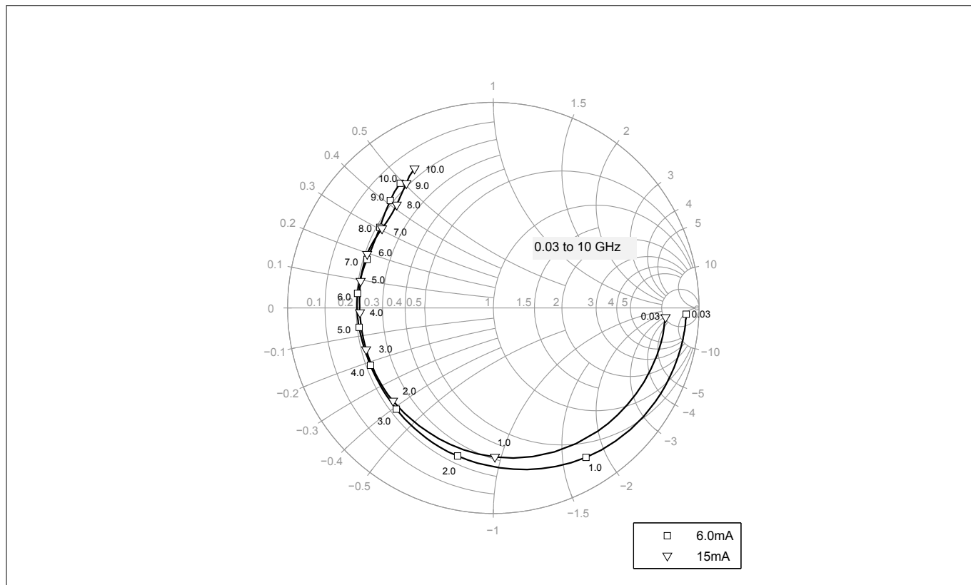
Figure 16 Input reflection coefficient S_{11} = f(f) , V_{CE} = 3 V, I_C = 6 / 15 mA
