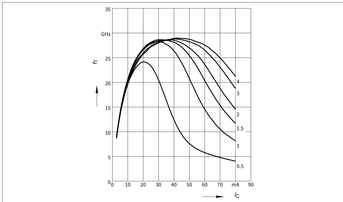
Figure 5 Transition frequency f_T = f(I_C) , f = 1 GHz, V_{CE} = \text{parameter in V}
