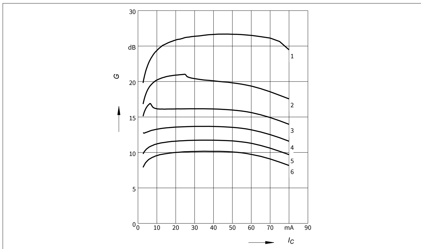
Figure 9 Maximum power gain G_{\max} = f(I_C) , V_{CE} = 2 V, f = parameter in GHz
