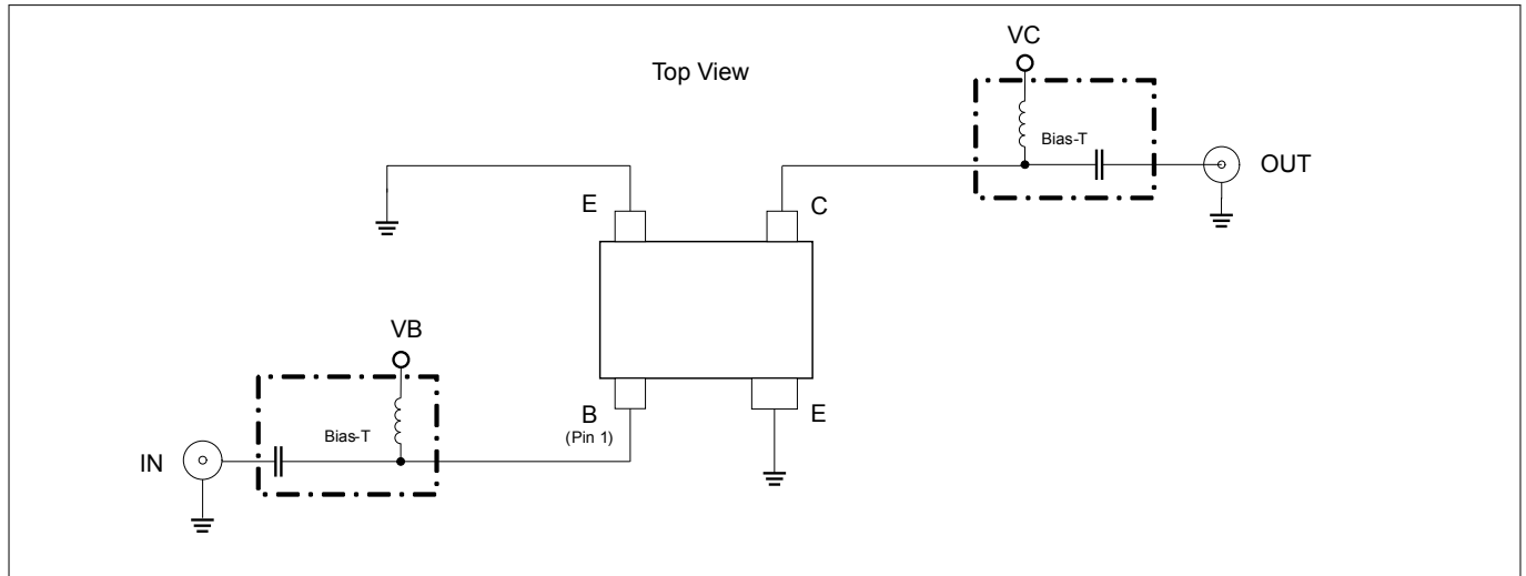
Figure 4 Testing circuit
