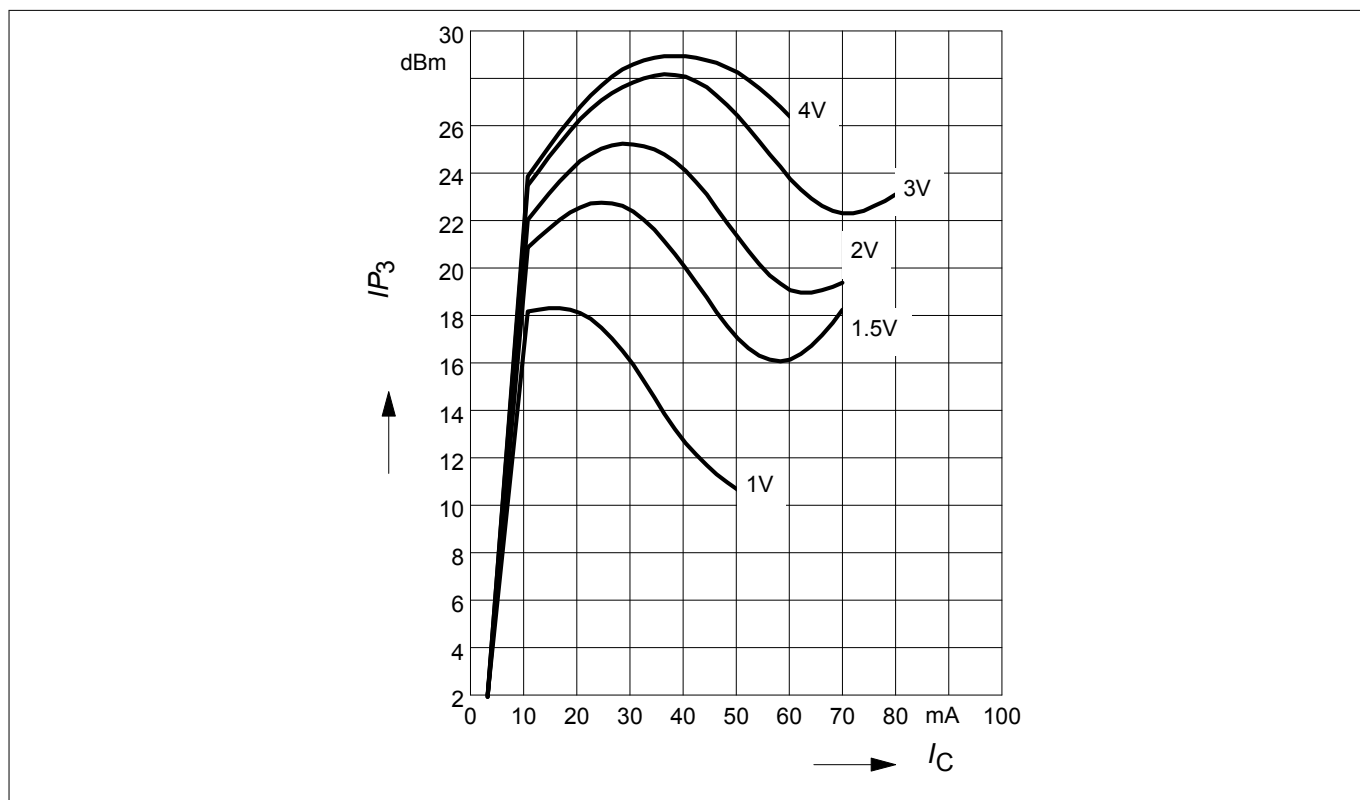
Figure 6 3rd order intercept point OIP_3 = f(I_C) , Z_S = Z_L = 50 \Omega , f = 1.8 GHz, V_{CE} = \text{parameter}
