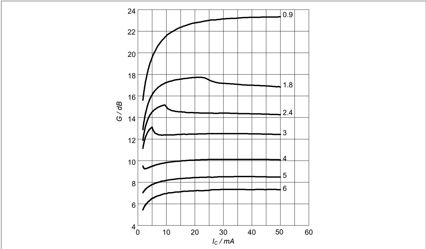
Figure 7 Maximum power gain G_{\text{max}} = f(I_C) , V_{CE} = 3 \text{ V} , f = \text{parameter in GHz}
