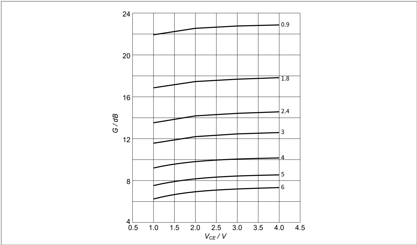
Figure 8 Maximum power gain G_{\text{max}} = f(V_{CE}) , I_C = 20 \text{ mA} , f = \text{parameter in GHz}
