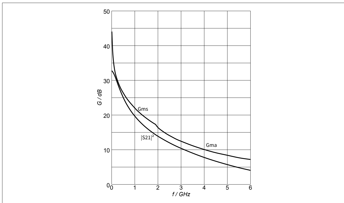
Figure 6 Gain G_{ma} , G_{ms} , |S_{21}|^2 = f(f) , V_{CE} = 3 \text{ V} , I_C = 20 \text{ mA}
