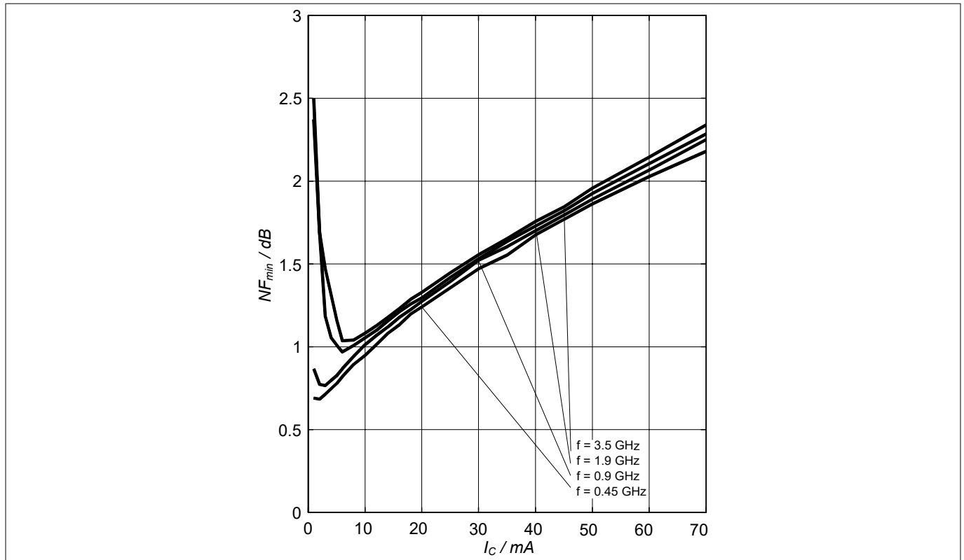
Figure 11 Noise figure NF_{min} = f(I_C) , V_{CE} = 2\text{ V} , Z_S = Z_{S,opt} , f = parameter in GHz
