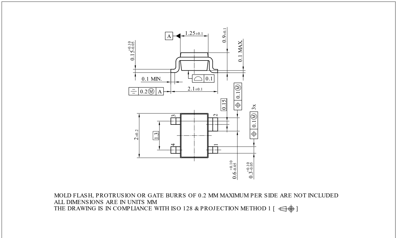
Figure 20 SOT343 package
