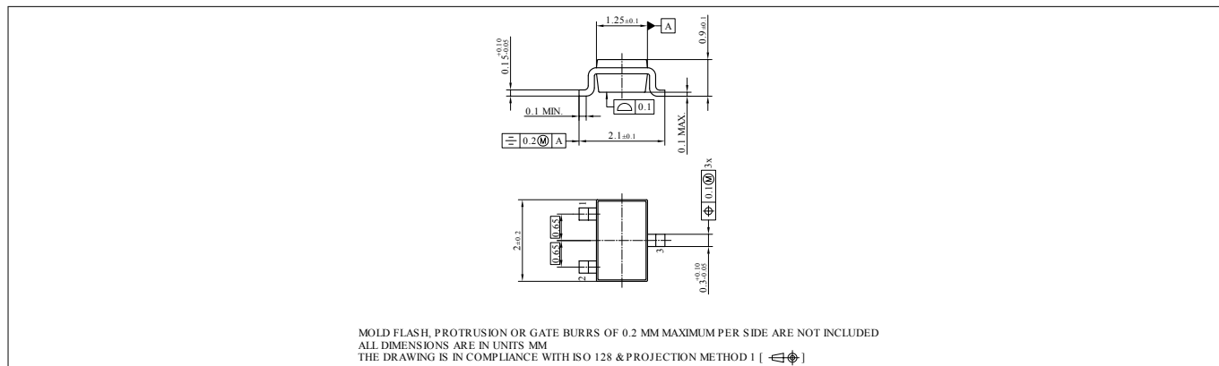
Figure 10 Package outline
