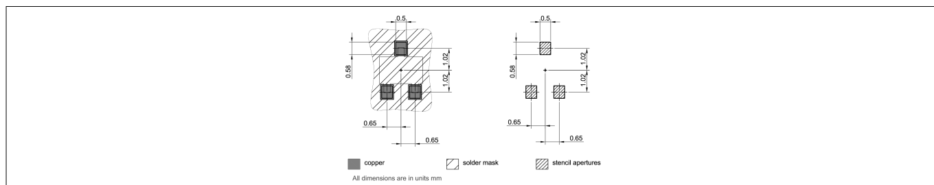
Figure 11 Foot print
