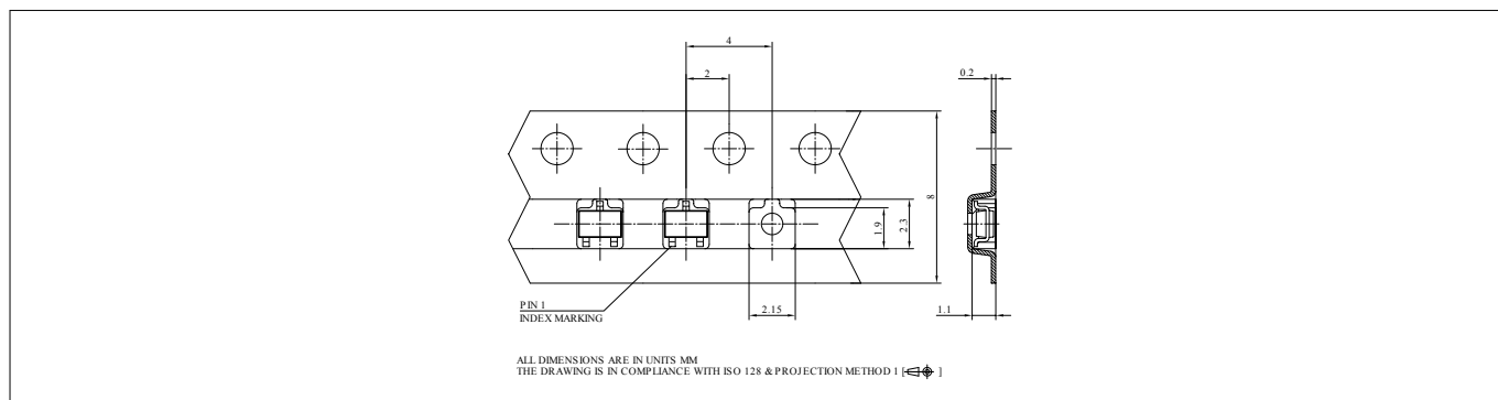
Figure 13 Tape information
