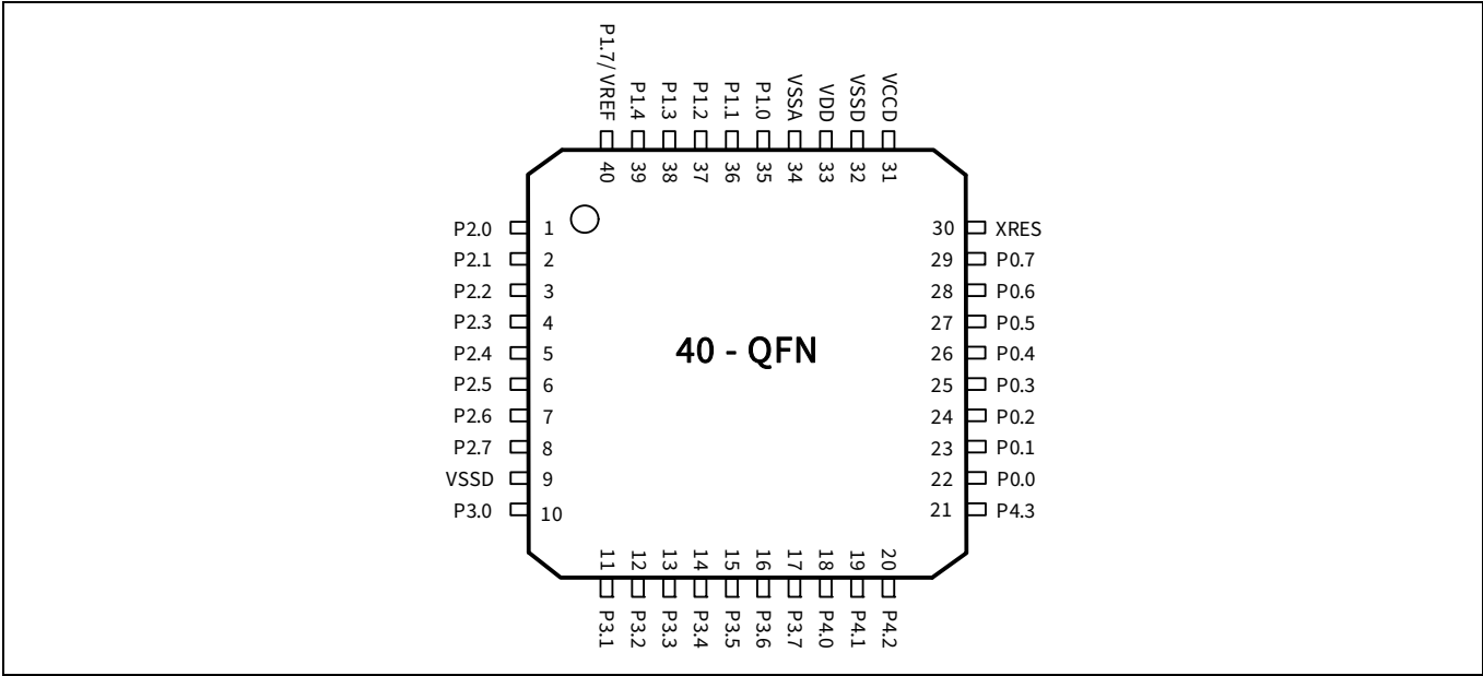
Figure 5 40PIN_QFN
