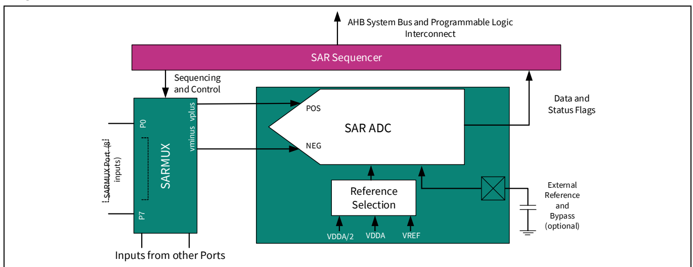
Figure 3 SAR ADC
