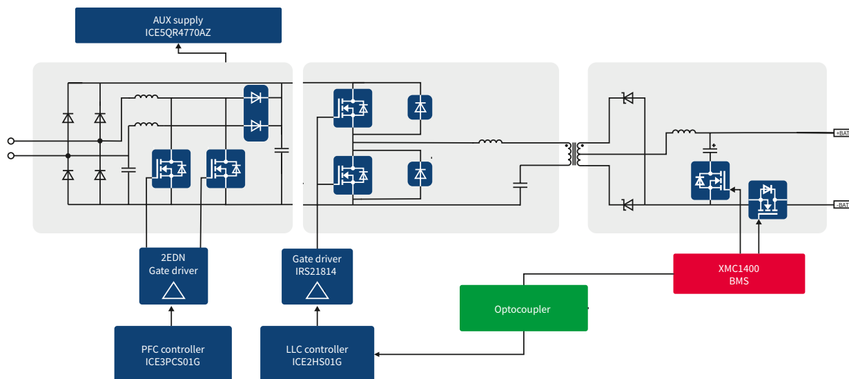
System diagram: 2 kW battery charger for light electric vehicles
