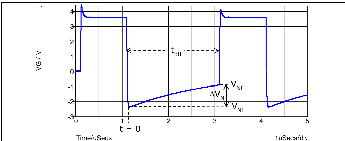
Figure 8 Gate-voltage waveform for V_S = 12 V
