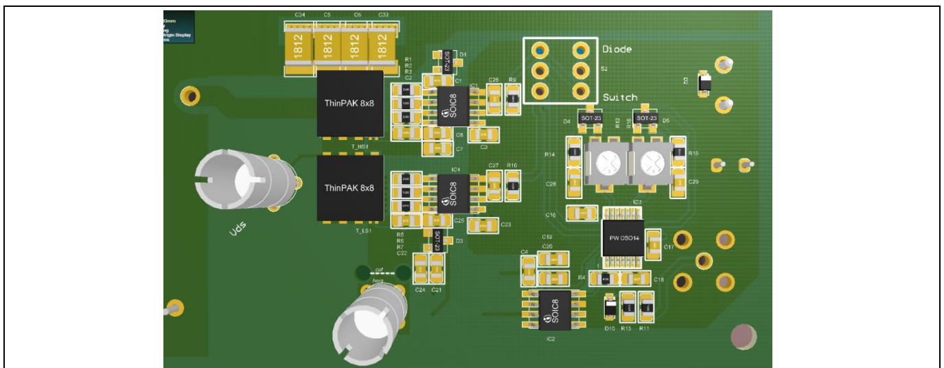
Figure 16 PCB for switching measurements
