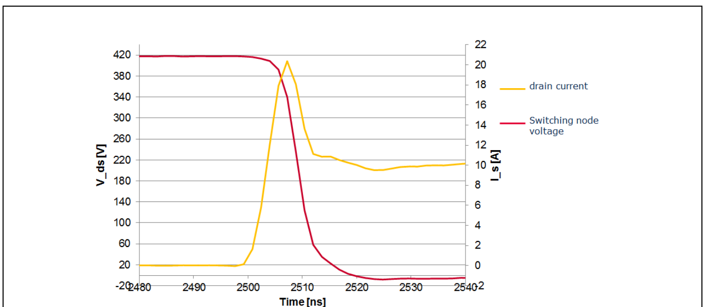
Figure 17 Measured switching voltage and current for I_{Load} = 10\text{ A}
