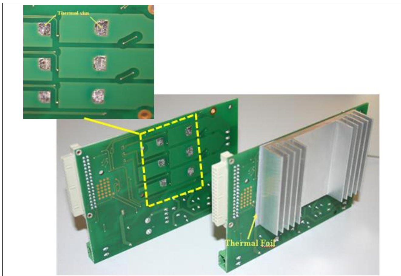
Figure 13 Example of thermal vias and heatsink mounting for RC-D and RC-DF test boards
