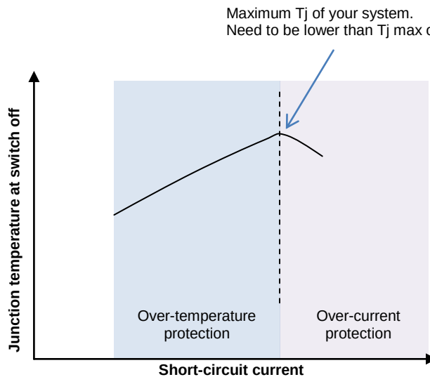
Figure 5: Protection evaluation
