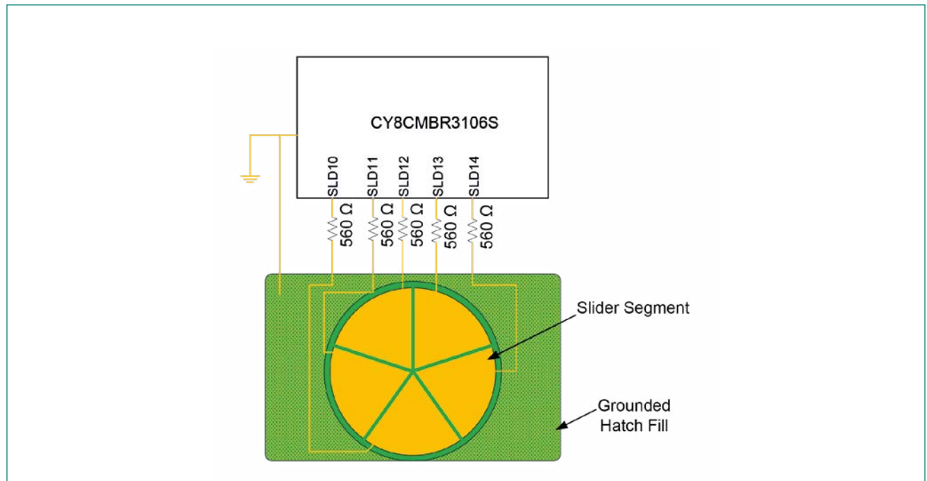
Figure 2-12 Shield Electrode (SH) and Guard Sensor (GUARD) Connected to CY8CMBR3xxx
