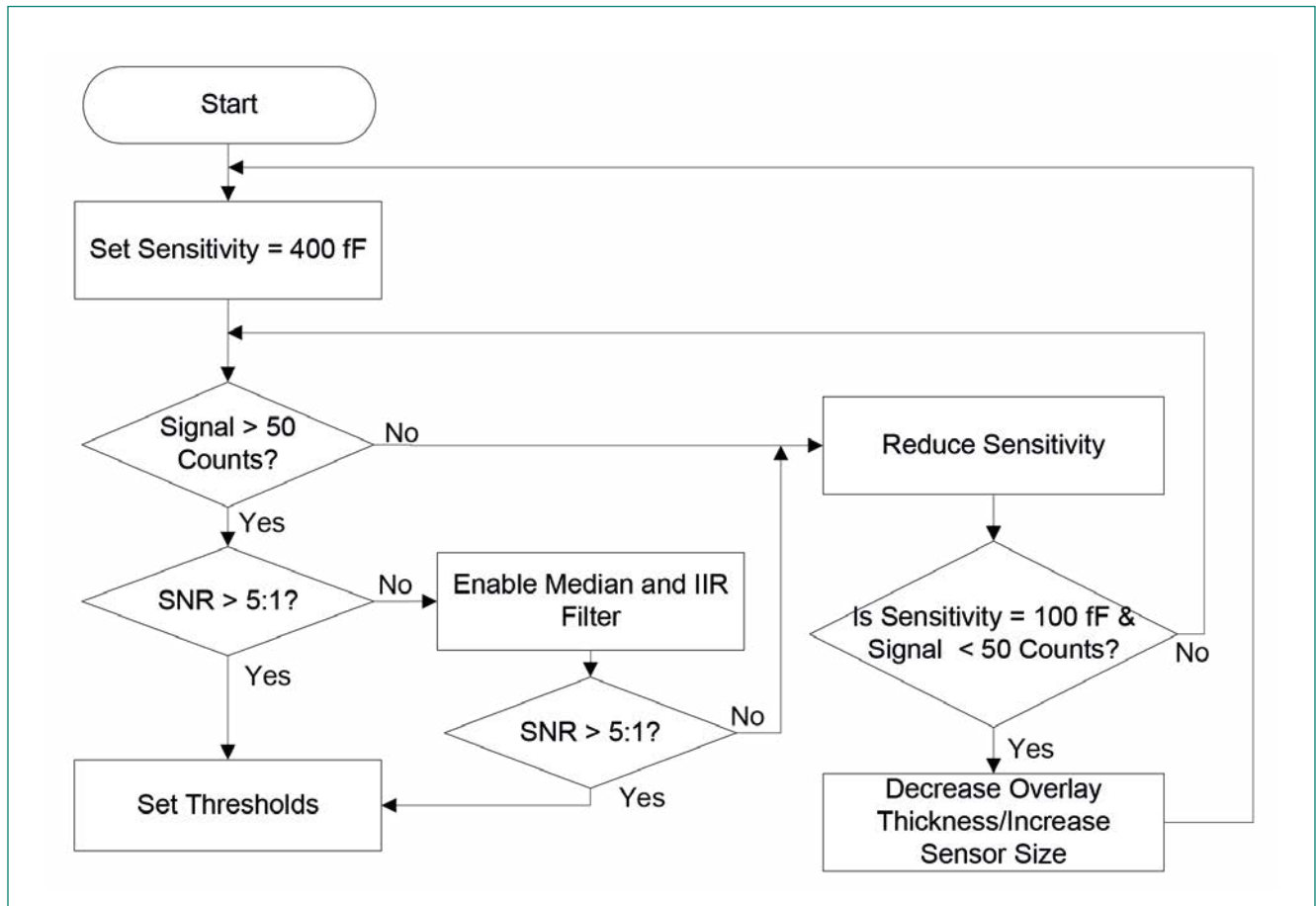
Figure 6-3 Buttons, Sliders, and Guard Sensor Tuning
