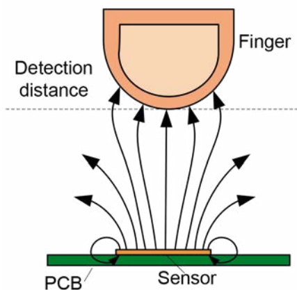
Figure 4-10 Electrical Field Propagation for a Single Sensor Configuration without a Metal Object
