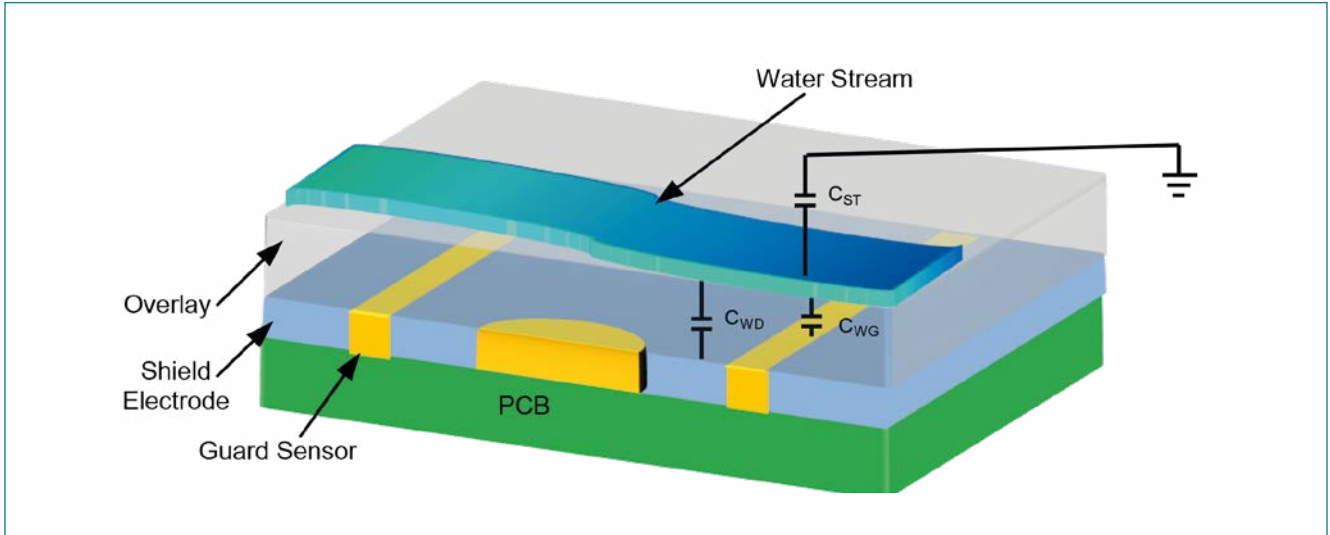
Figure 2-14 Capacitance Measurement With Liquid Stream
