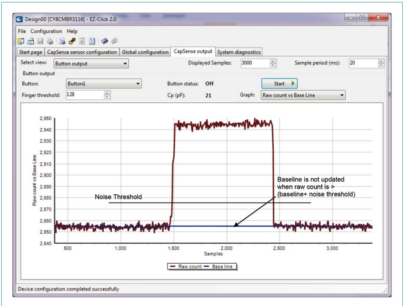
Figure 6-4 Noise Threshold
