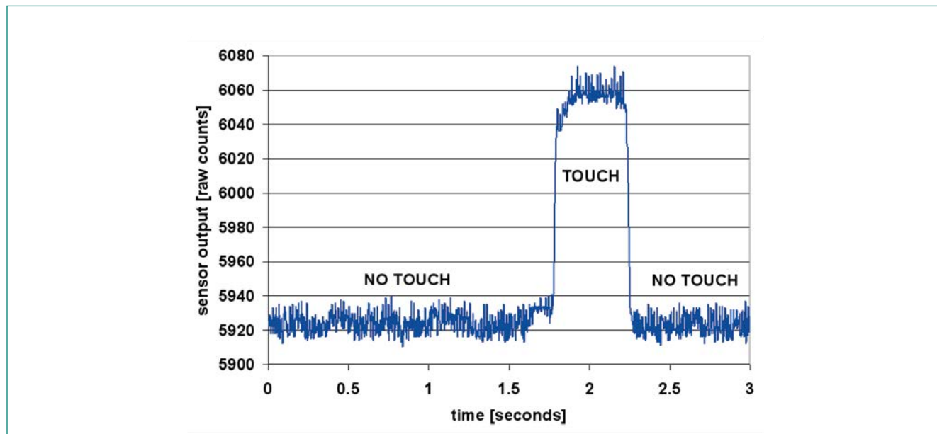
Figure 2-6 Raw Counts during Finger Touch
