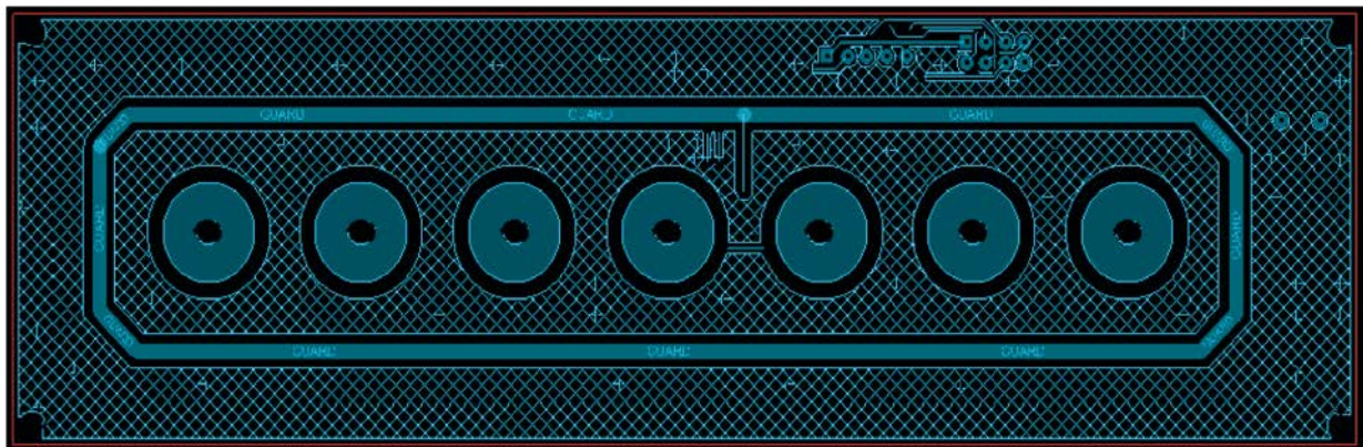
Figure 4-17 Liquid-Tolerant Touch Buttons on FR4 PCB – Top Layer
