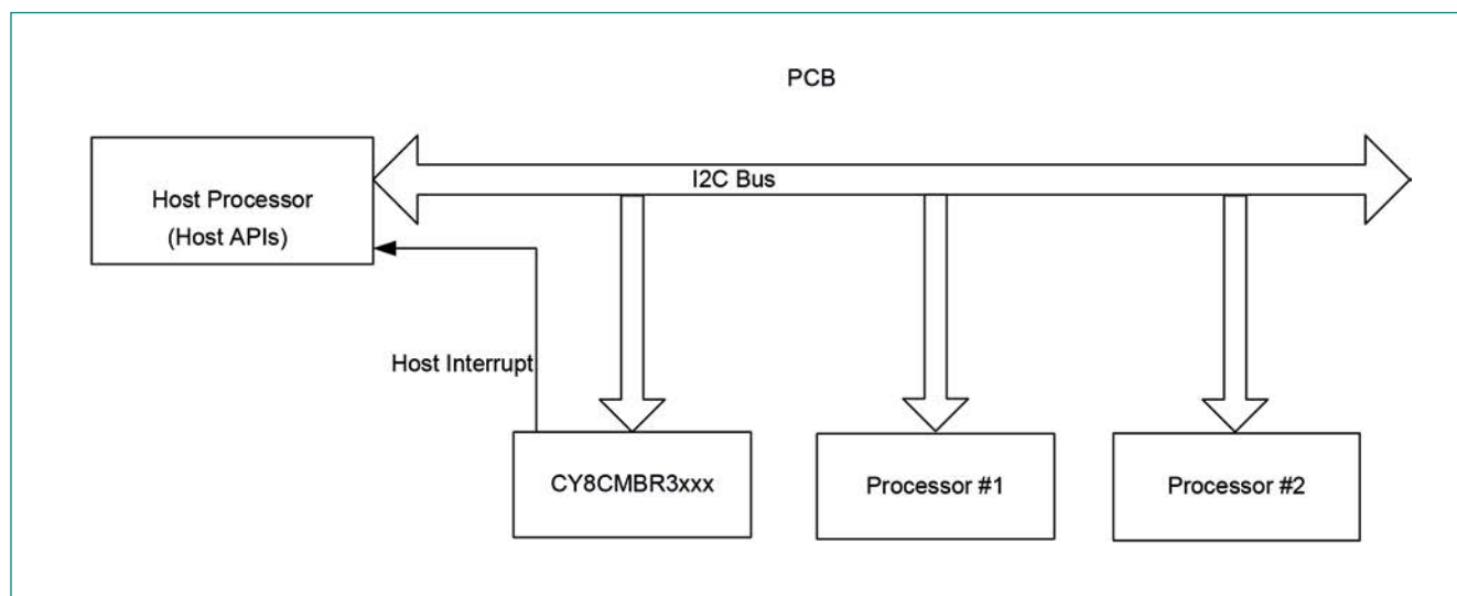
Figure 5-17 System Demonstrating Host API Usage
