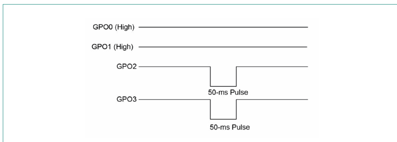
Figure 5-4 Example Showing CS0, CS1 Passing the BIST and CS2, CS3 Failing
