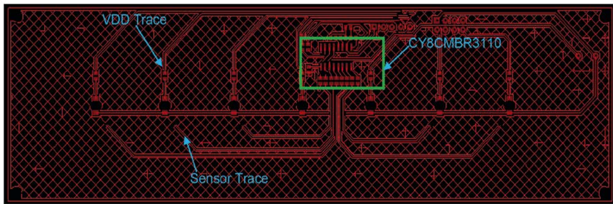
Figure 4-18 Liquid-Tolerant Touch Buttons on FR4 PCB – Bottom Layer
