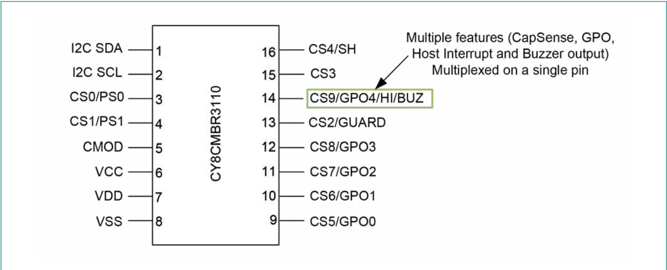
Figure 3-1 Multiple Features Supported on a Single Pin
