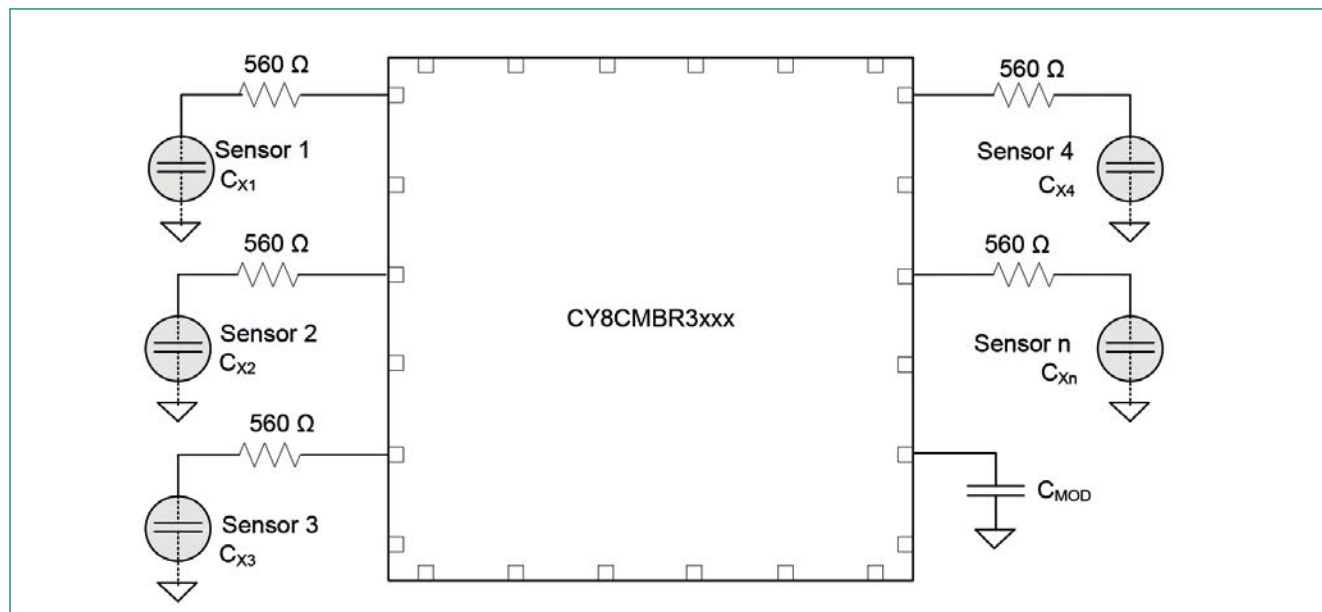
Figure 2-2 CAPSENSE™ Implementation in the CY8CMBR3xxx Device
