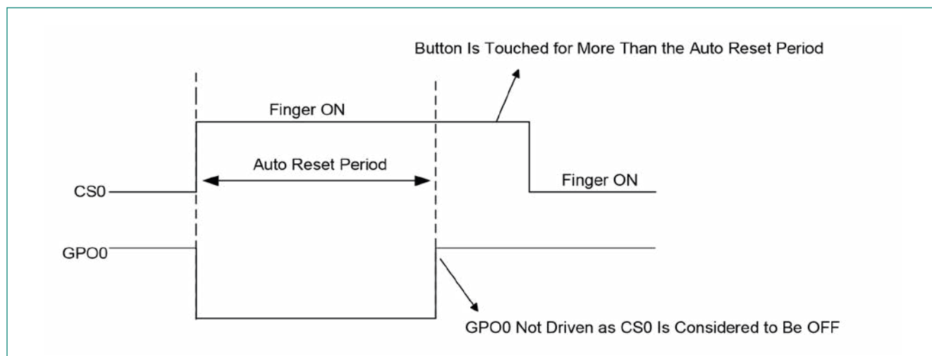
Figure 5-3 Sensor Auto Reset
