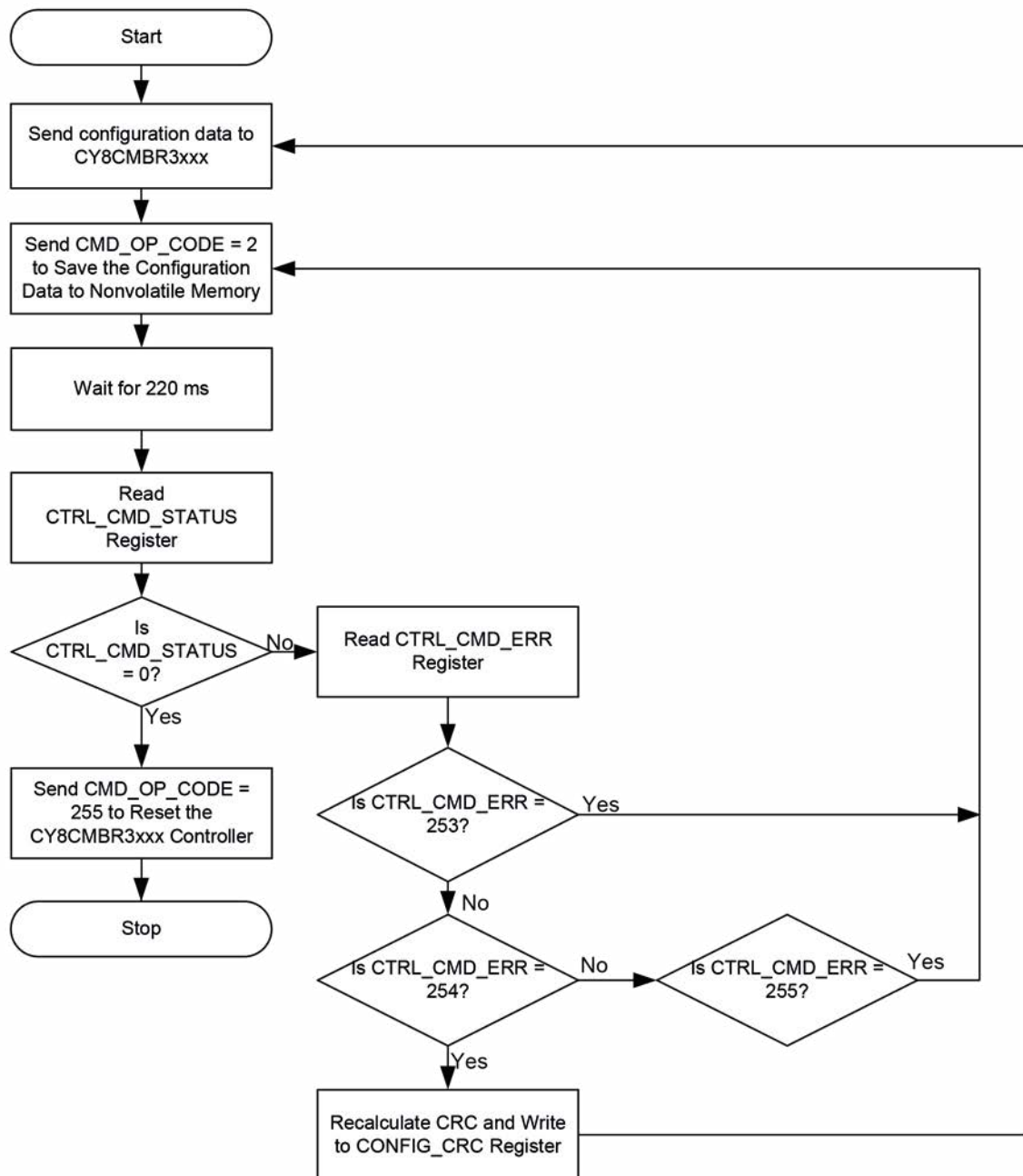
Figure 5-24 Flowchart for Configuring the CY8CMBR3xxx Using BCP
