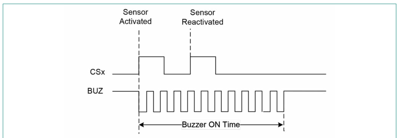
Figure 5-10 Buzzer Operation with Consecutive Touches of the Same Sensor
