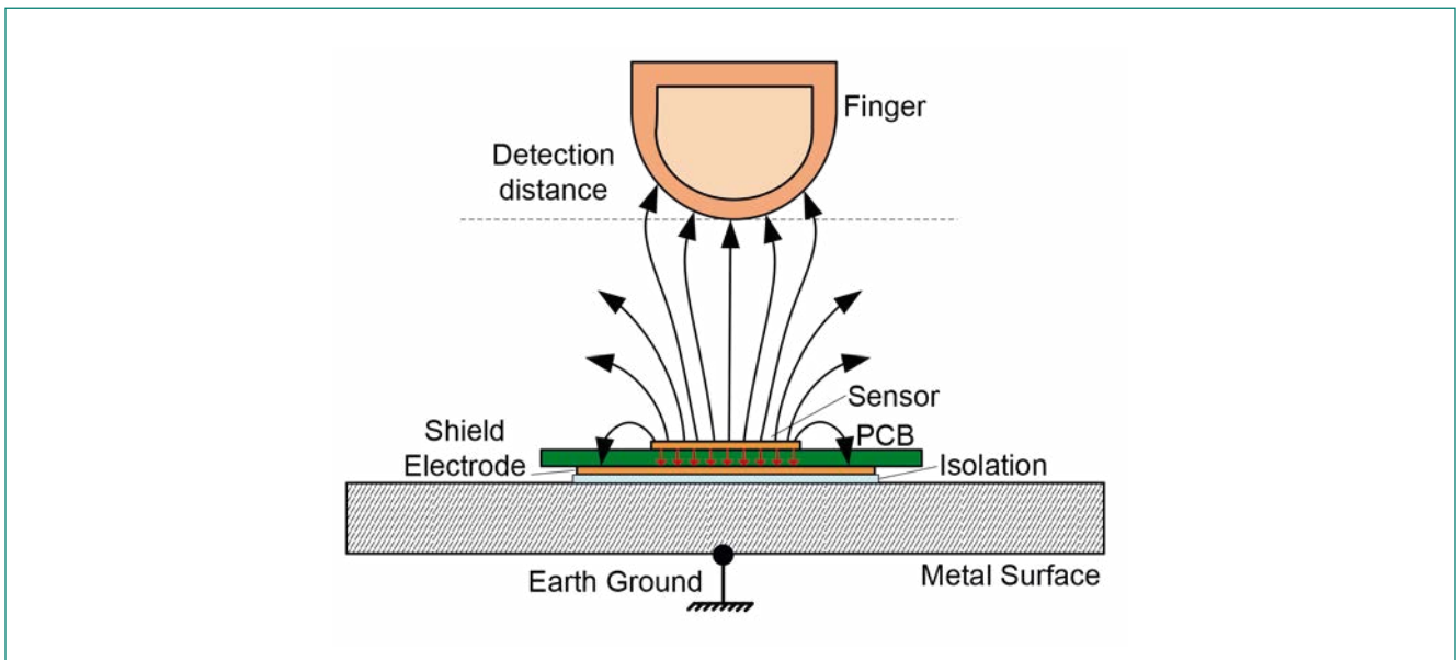
Figure 4-12 Using a Shield Electrode to Decrease the Metal Object's Influence
