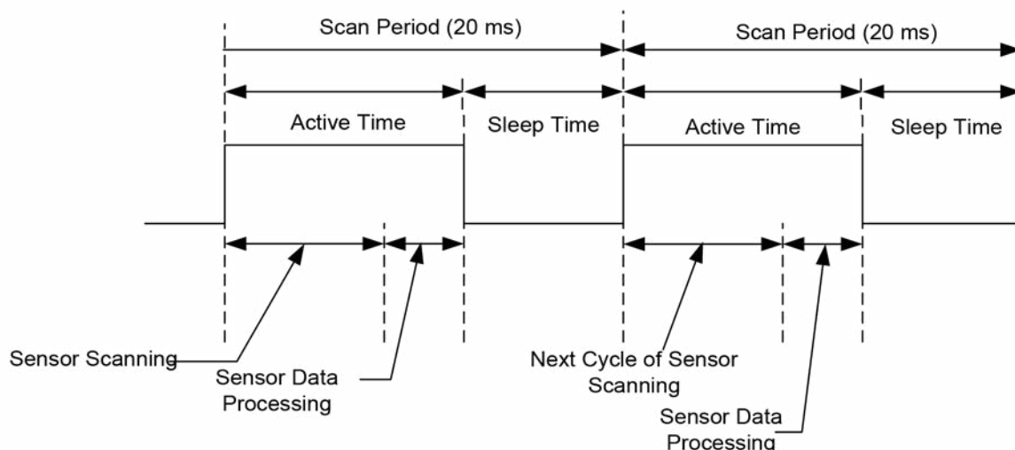
Figure 7-2 Active Mode Scan-Sleep Sequence When Active Time < 20 ms
