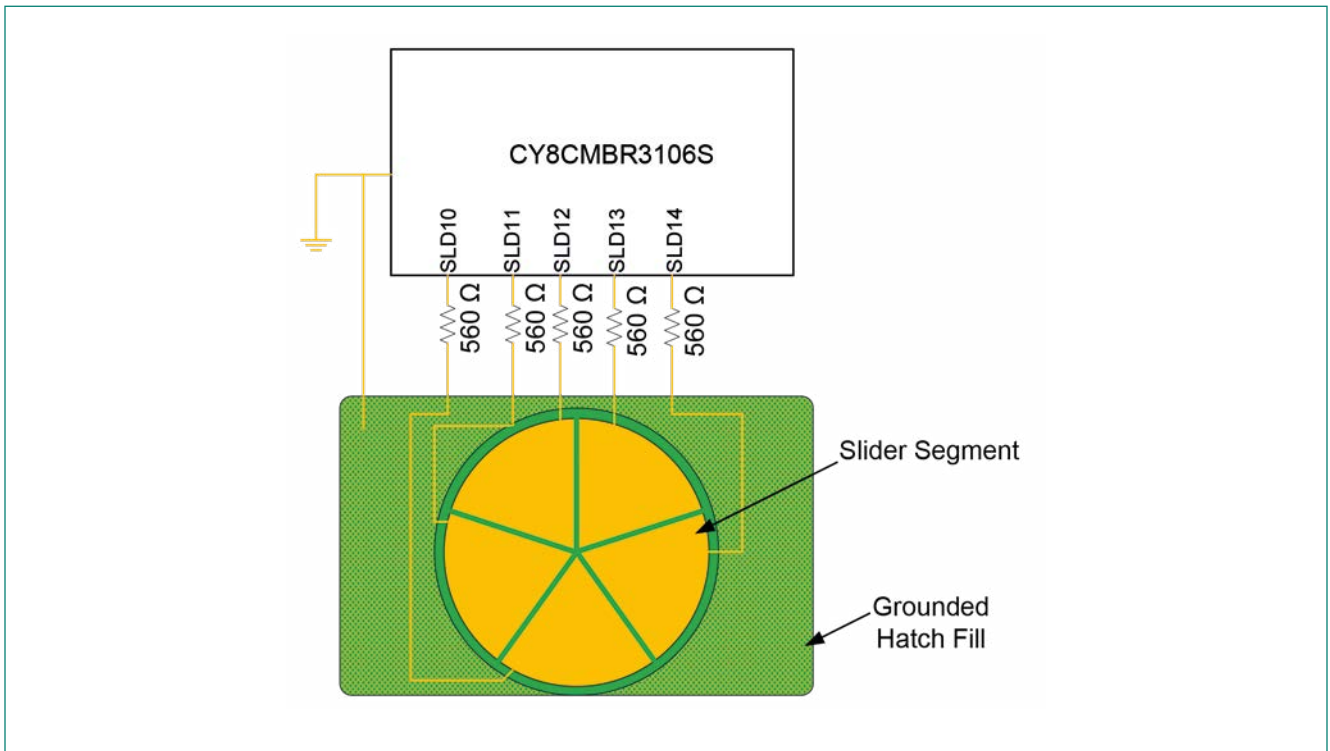
Figure 2-10 Radial Slider
