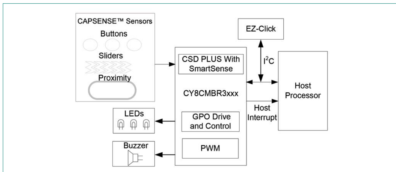
Figure 1-1 Block Diagram of a CAPSENSE™ System With CY8CMBR3xxx Controller
