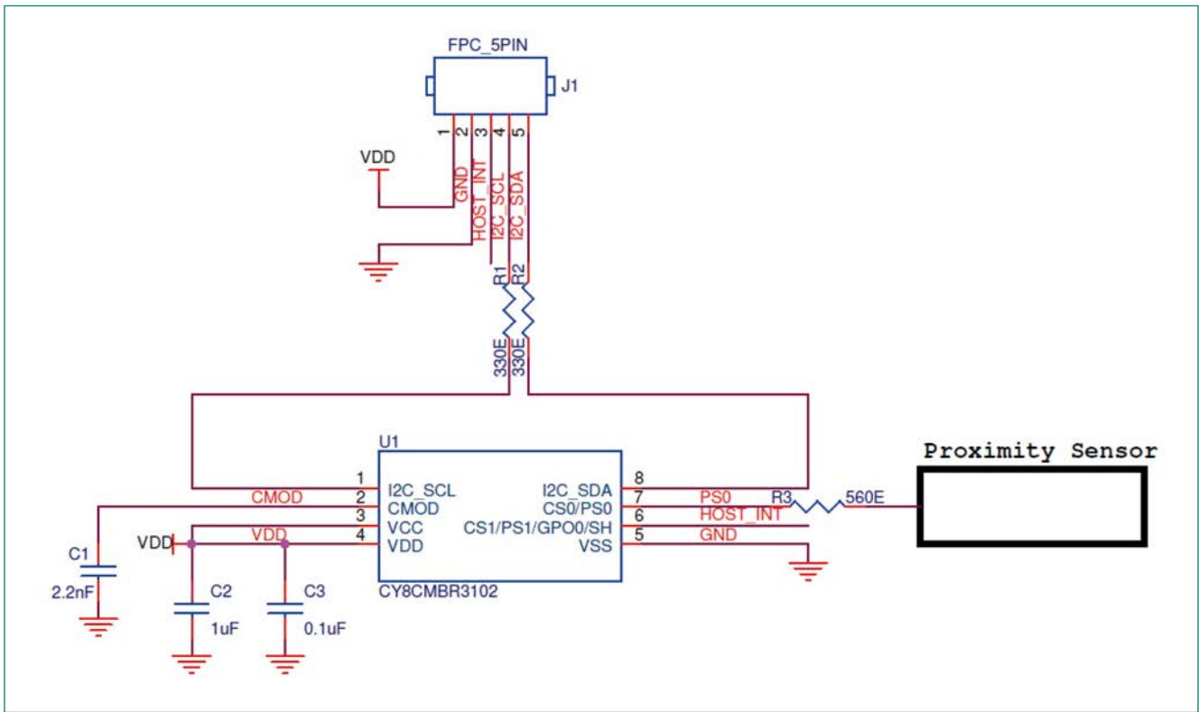
Figure 3-8 Schematic for Proximity-Sensing Application
