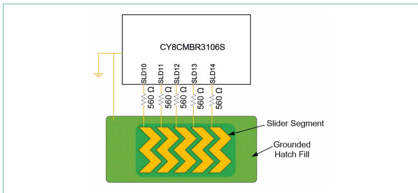
Figure 2-9 Linear Slider
