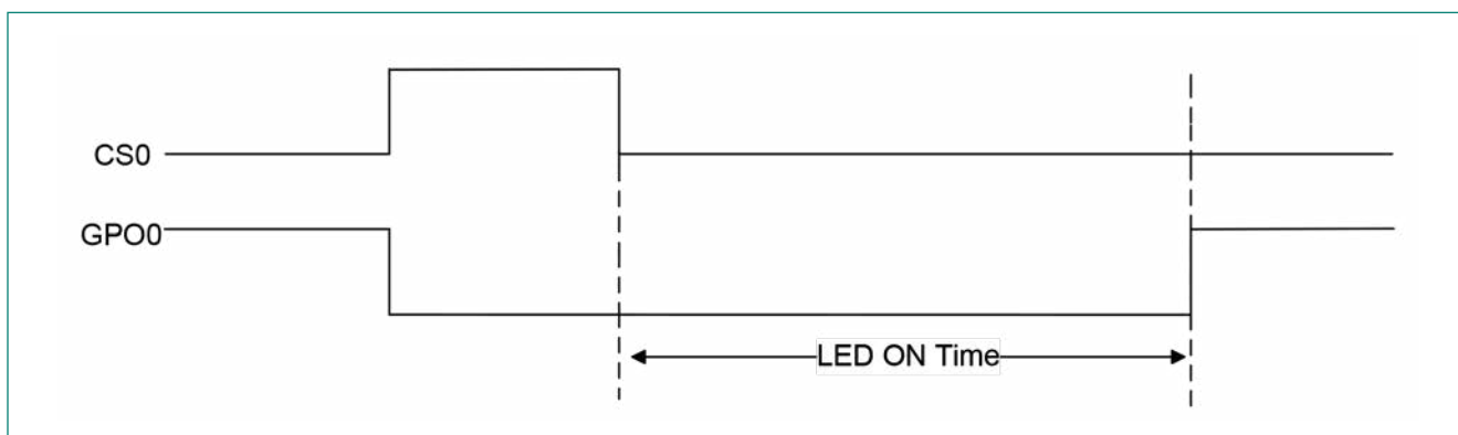
Figure 5-7 LED ON Time
