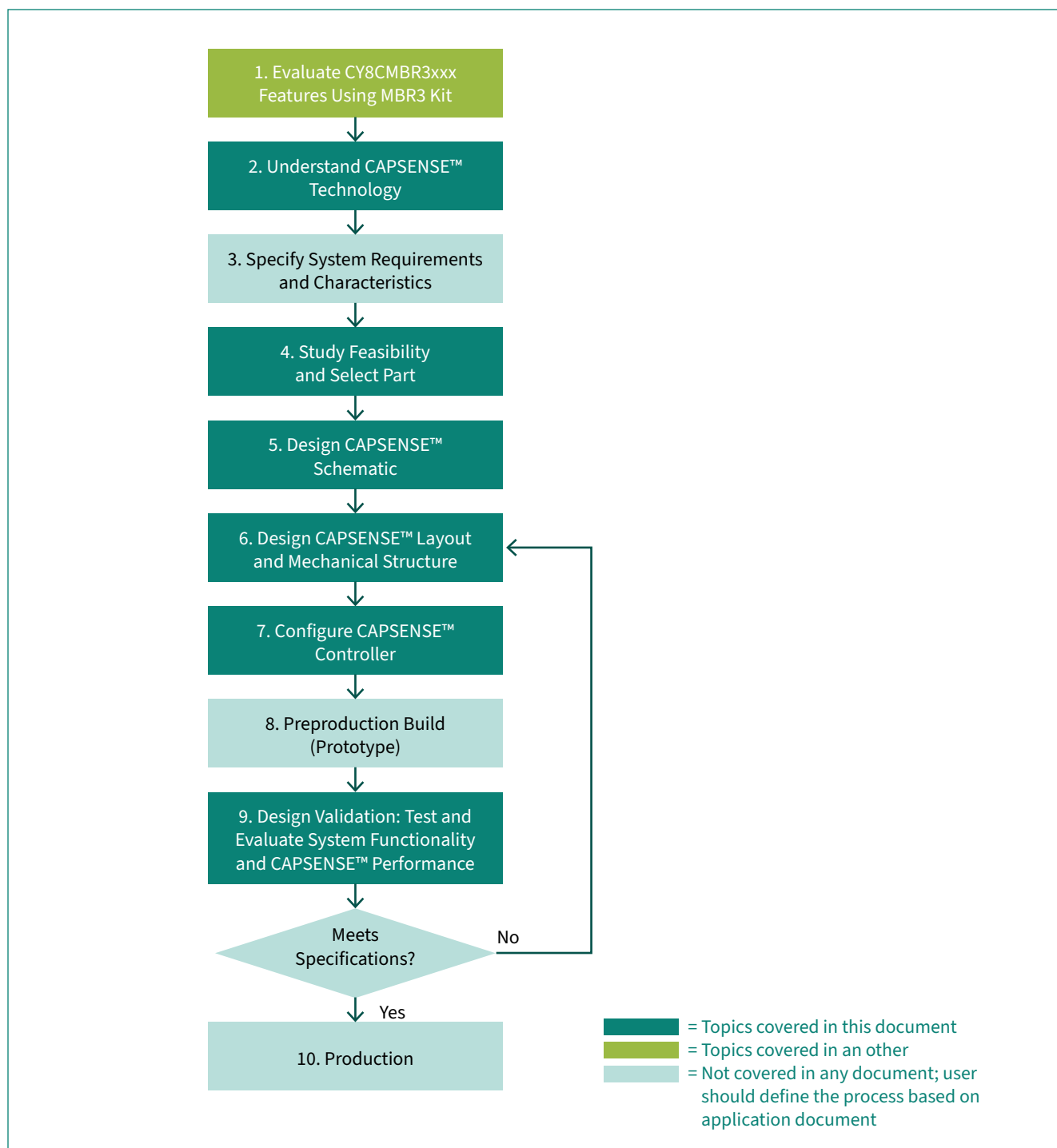
Figure 1-2 Typical CAPSENSE™ Product Design Flow
