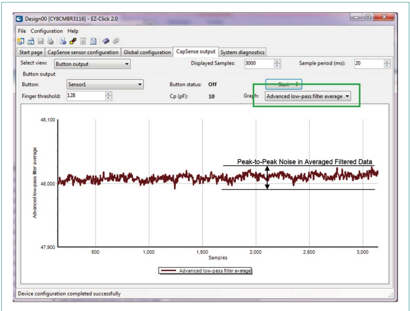
Figure 6-8 Peak-to-Peak Noise in Average Filtered Data
