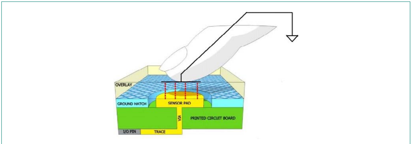
Figure 2-4 Section of Typical CAPSENSE™ PCB With the Sensor Being Activated by a Finger
