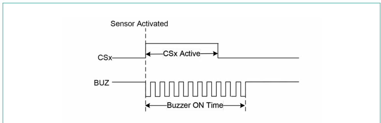
Figure 5-9 Buzzer Activation on Touch Event
