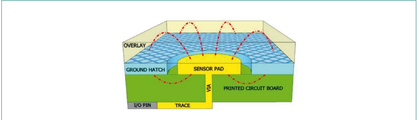
Figure 2-3 Parasitic Capacitance
