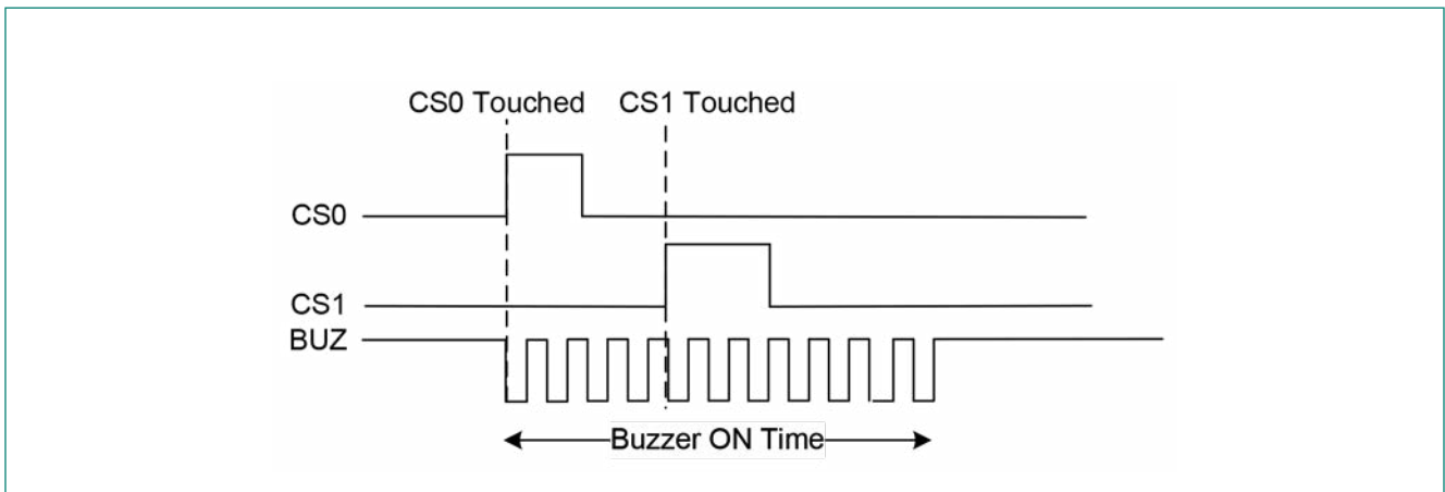
Figure 5-11 Buzzer Operation When Multiple Sensors Are Activated
