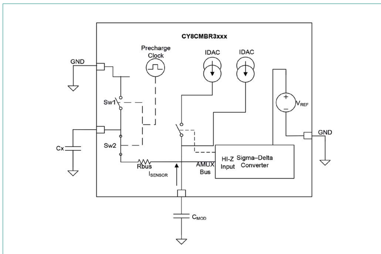
Figure 2-5 CSD PLUS Block Diagram
