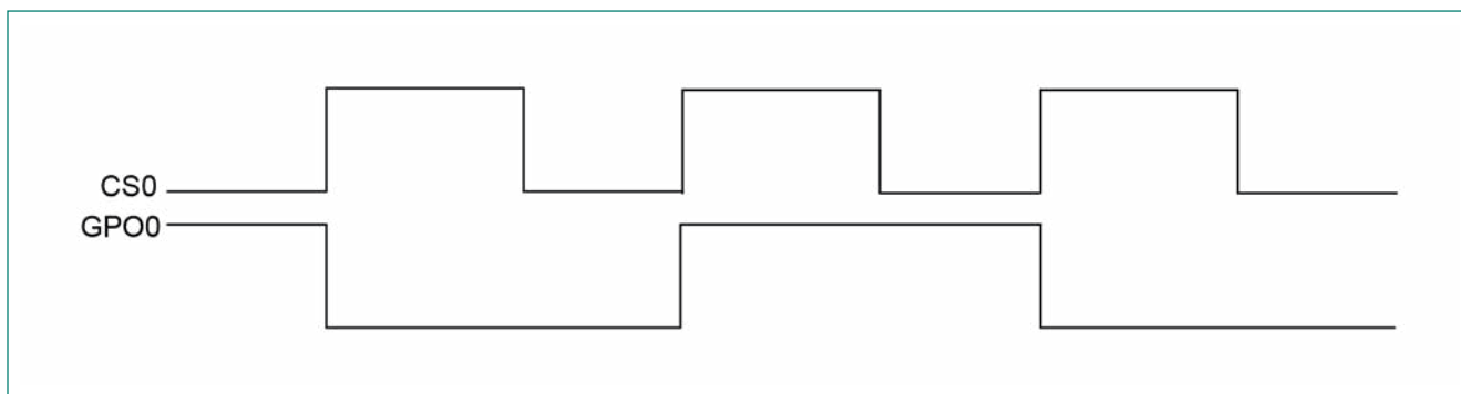
Figure 5-6 Example of Toggle Feature
