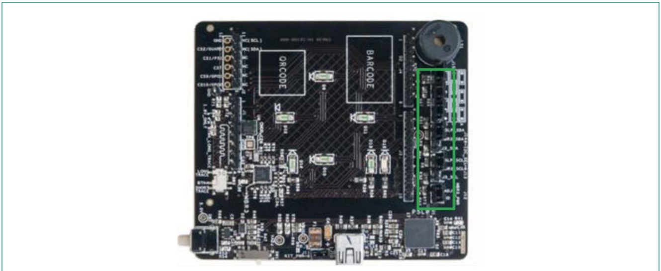
Figure 5-18 Jumper J13, J14 and J15 Location on the MBR3 Evaluation Kit
