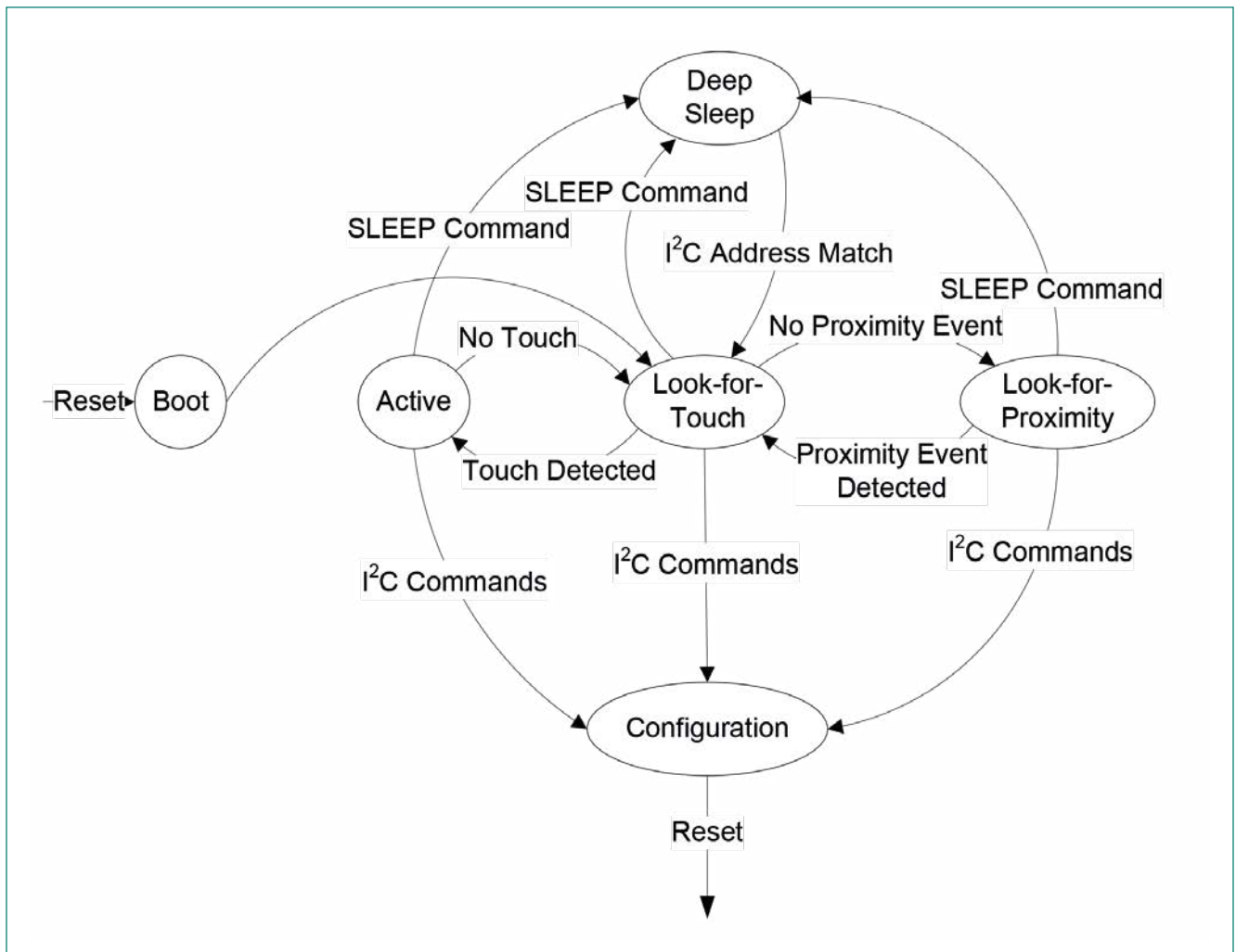
Figure 7-1 CY8CMBR3xxx Operational Modes
