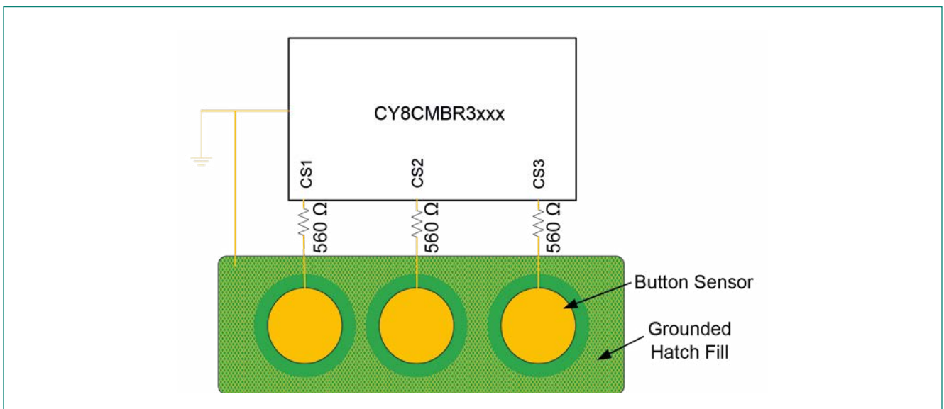
Figure 2-8 Simple CAPSENSE™ Buttons
