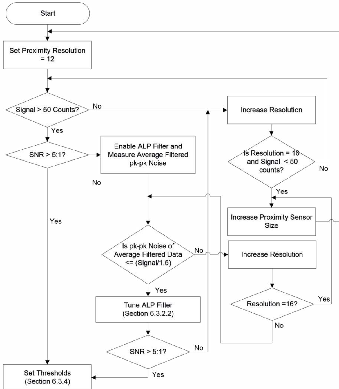
Figure 6-6 Proximity Sensor Tuning
