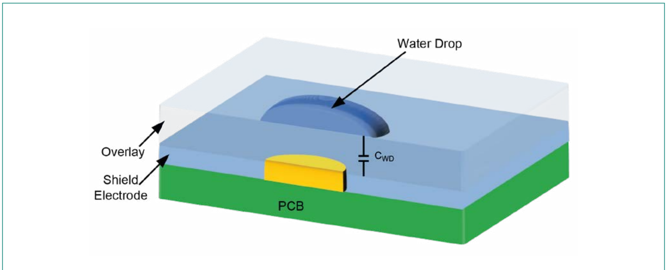
Figure 2-13 Capacitance Measurement with Liquid Drop
