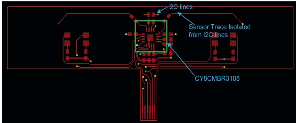
Figure 4-16 Touch Buttons on FPC – Button Layer
