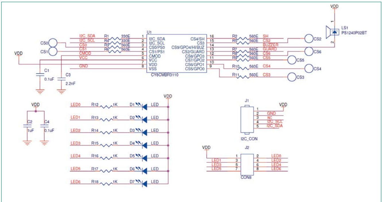
Figure 3-7 Schematic for Touch Buttons in Induction Cooker
