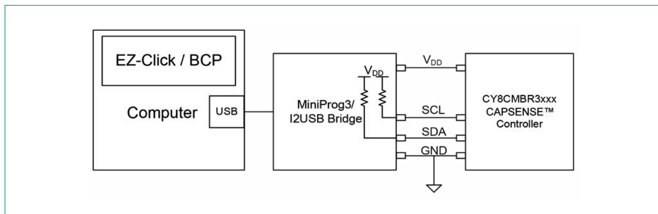
Figure 5-13 Hardware Setup Required for Configuring CY8CMBR3xxx Using EZ-Click or BCP
