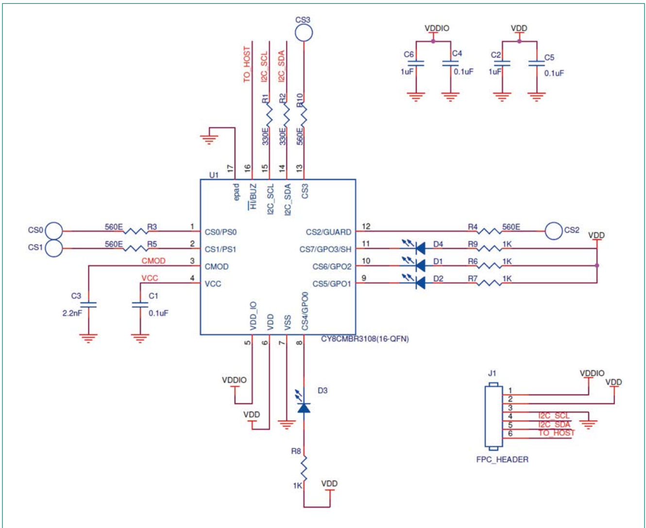
Figure 3-6 Schematic for Touch Buttons in Mobile Phone
