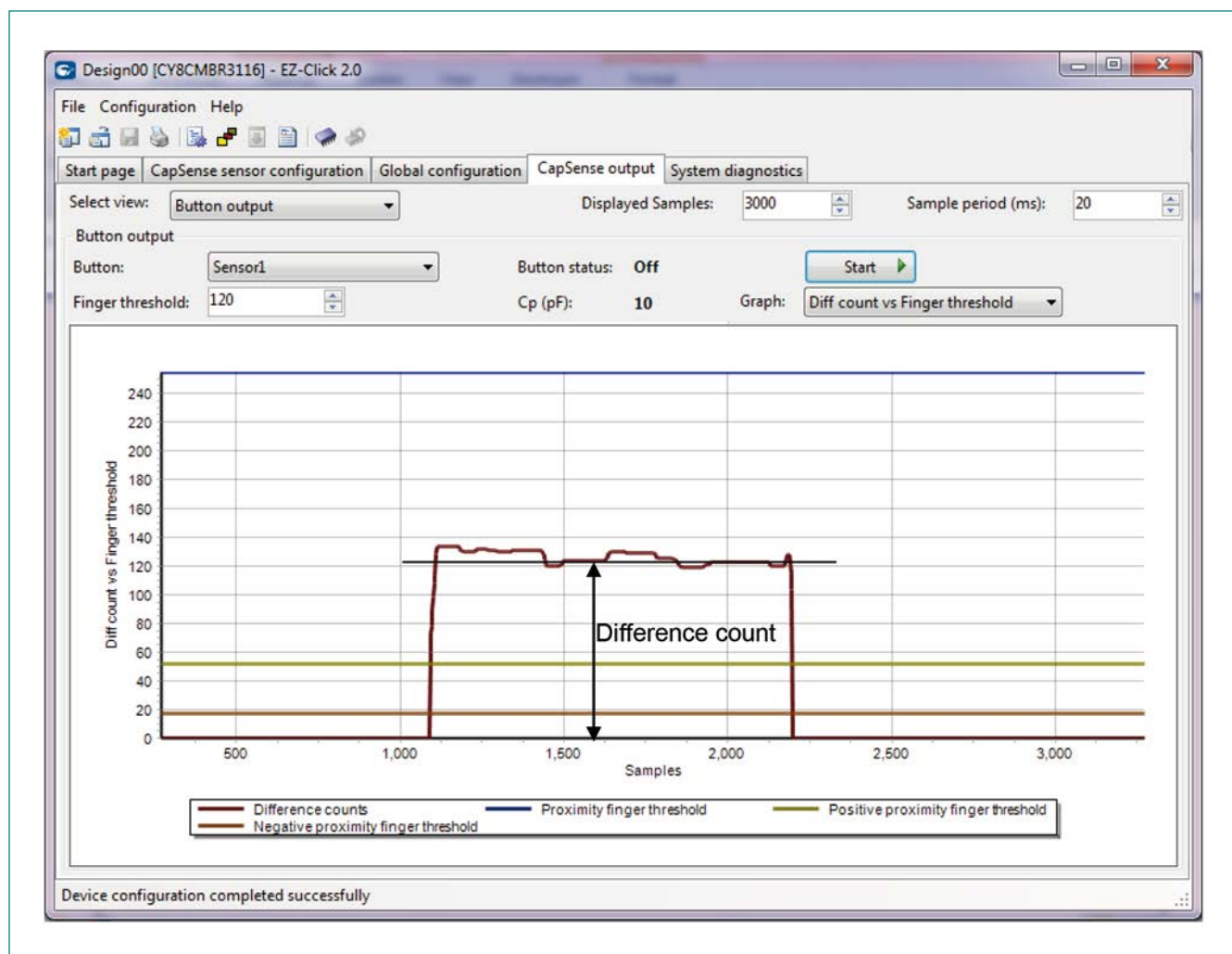
Figure 6-10 Measuring Difference Count to Set Proximity Sensor Thresholds
