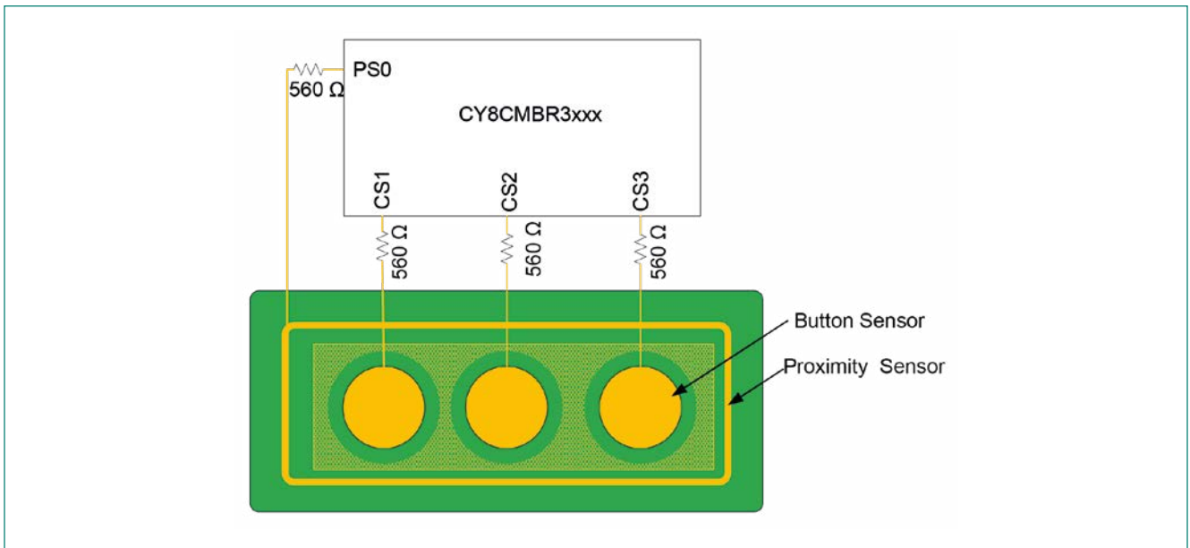
Figure 2-11 Proximity Sensor
