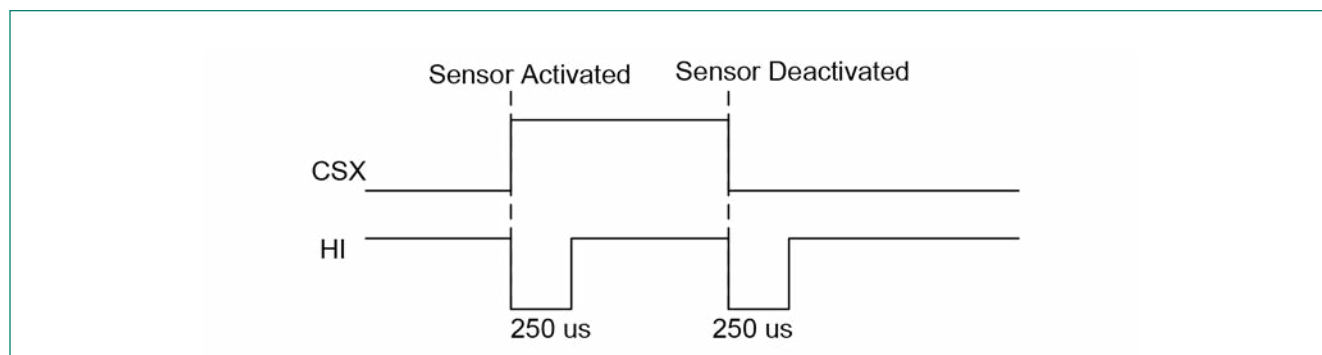
Figure 5-5 Host Interrupt Line when CSx Button is Touched
