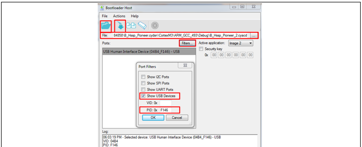
Figure 11 Bootloader host application
