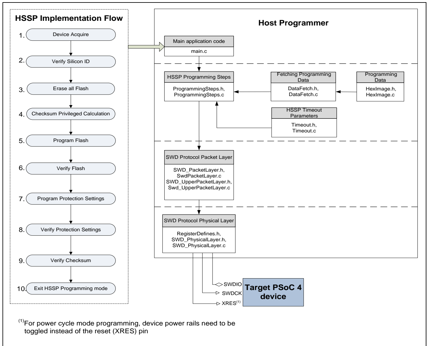
Figure 1 HSSP firmware architecture
