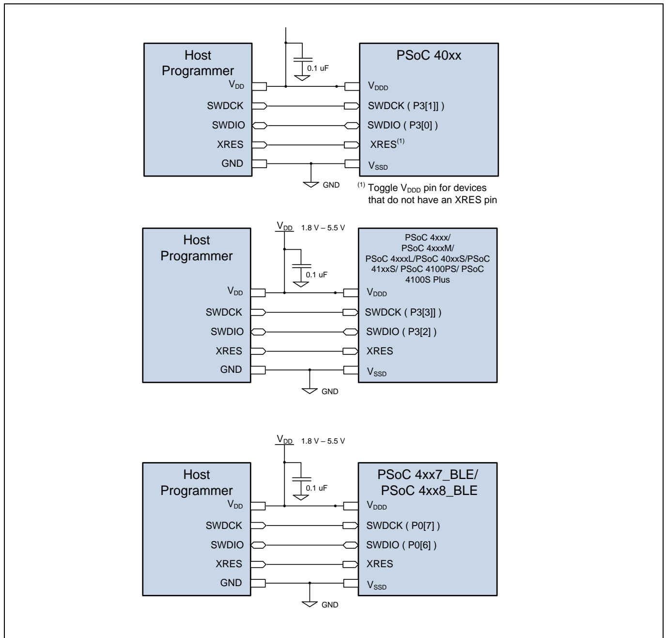
Figure 3 Basic host/target connections
