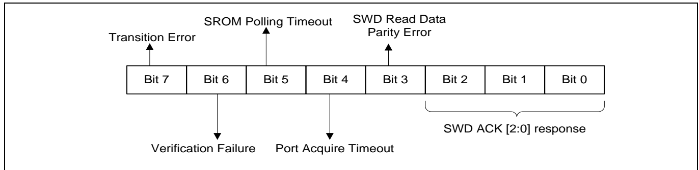
Figure 2 HSSP Error Status register
