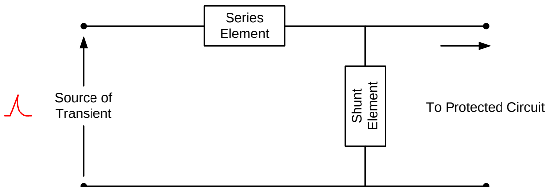
Figure 21. Transient-Protection Network
