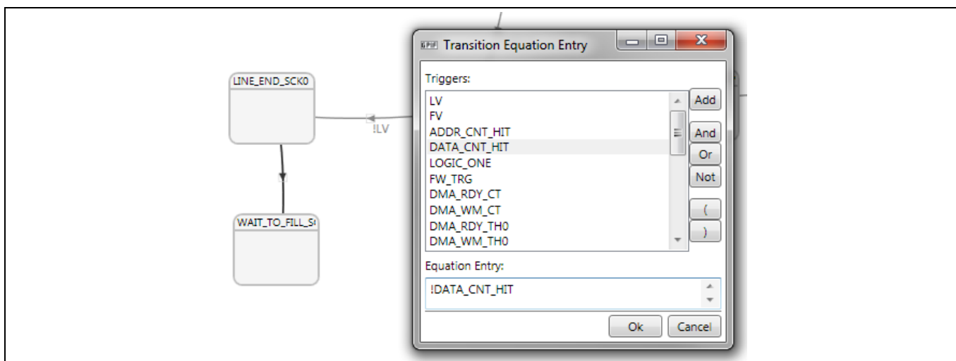
Figure 35 DATA_CNT_HIT indicates the counter has reached its programmed limit
