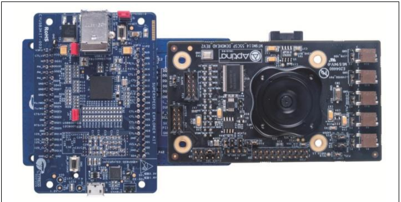
Figure 61 SuperSpeed explorer kit, Aptina interconnect, and Aptina sensor board assembly
