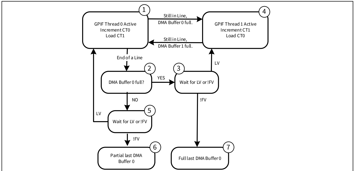
Figure 12 Data transfer decisions at the end of a video line
