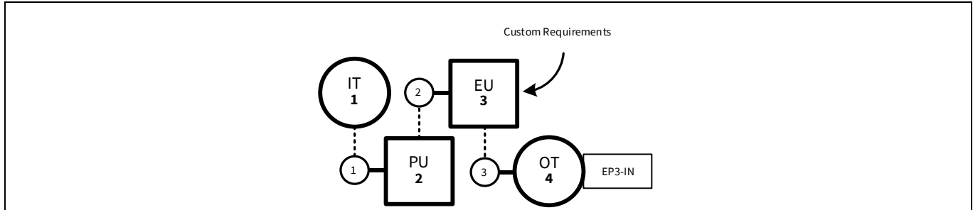
Figure 3 UVC diagram of the camera architecture
