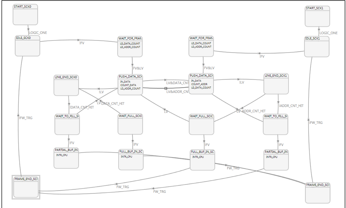
Figure 39 Final state machine diagram
