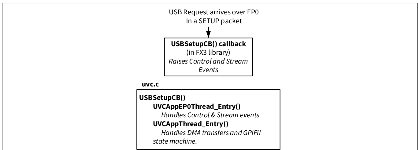
Figure 47 Camera project structure
