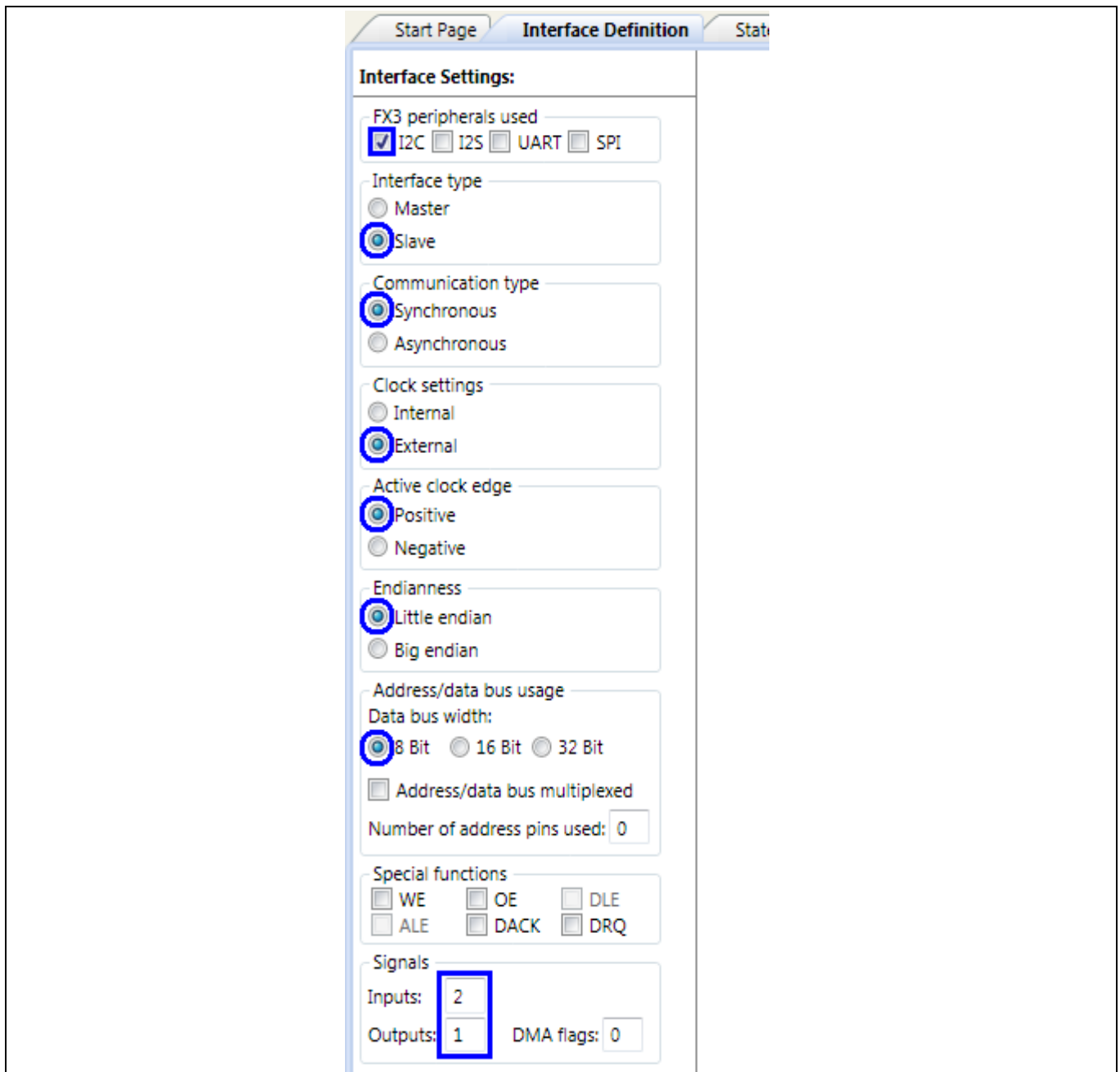
Figure 18 Interface setting selections
