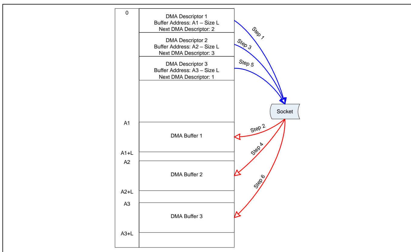
Figure 10 DMA Transfer Example
