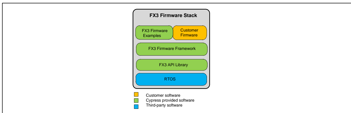
Figure 28 Structure of Firmware SDK
