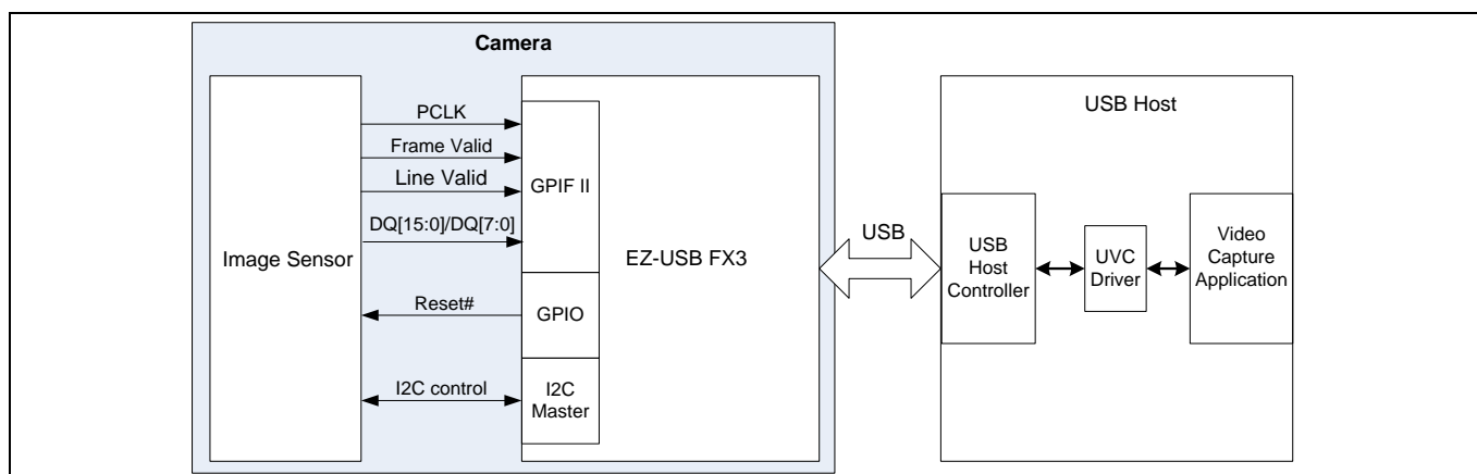
Figure 4 Image Sensor Interfaced to FX3
