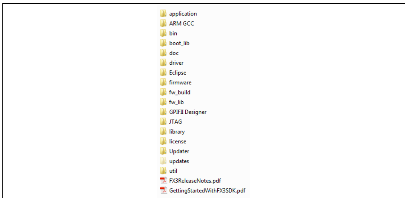
Figure 27 Directory Structure
