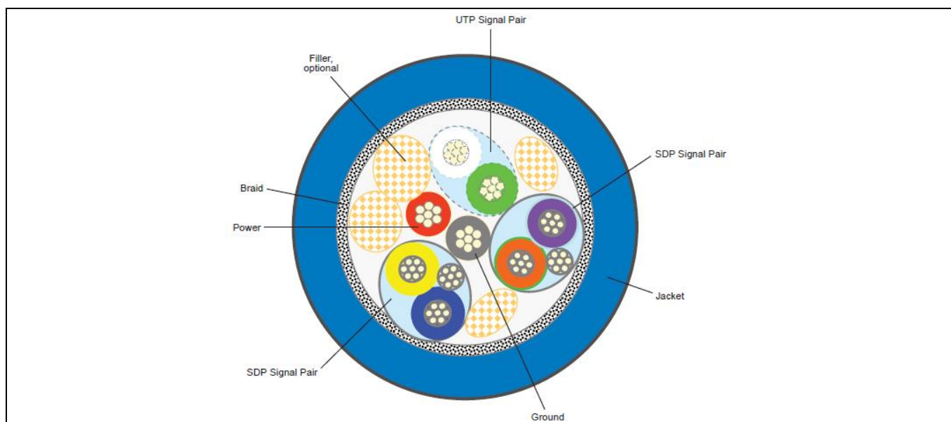
Figure 34 USB 3.0 Cable Architecture
