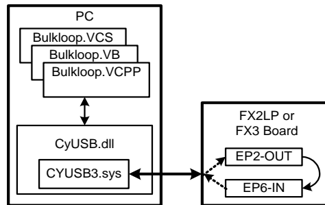
Figure 2. Bulkloop Data Flow
