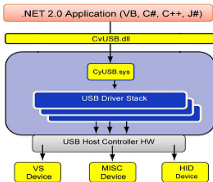
Figure 8. Application Development with CyUSB.dll
