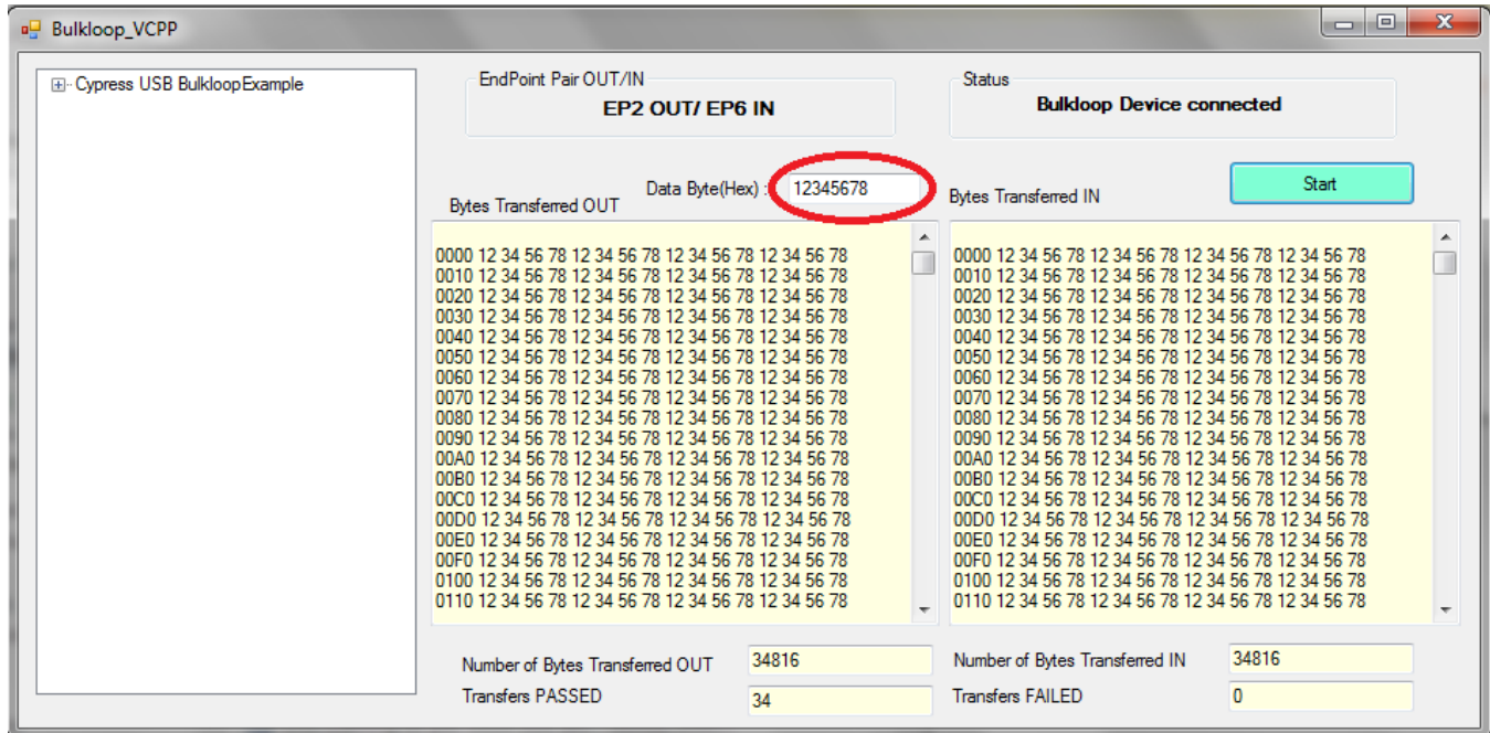
Figure 7. Data Transfer from Bulkloop Application
