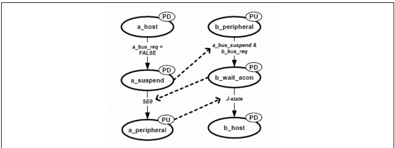
Figure 6 HNP Simplified and Combined State Diagram
