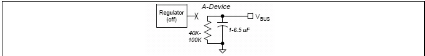
Figure 8 Load Presented by an Unpowered A-Device
