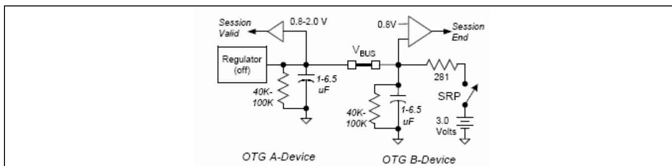
Figure 9 B-Device Pulses VBUS to Wake Up A-Device
