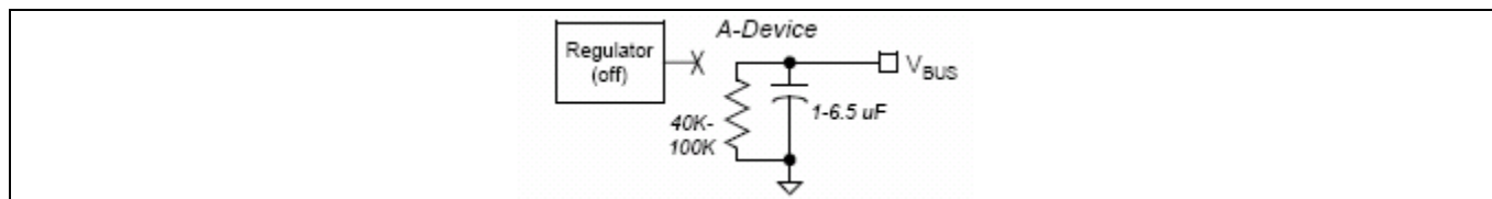
Figure 8 Load Presented by an Unpowered A-Device
