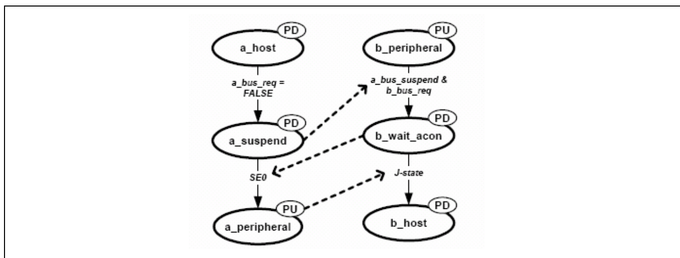
Figure 6 HNP Simplified and Combined State Diagram
