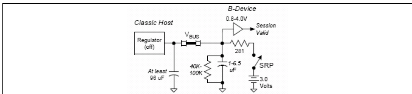
Figure 10 A Cost-Sensitive B-Device
