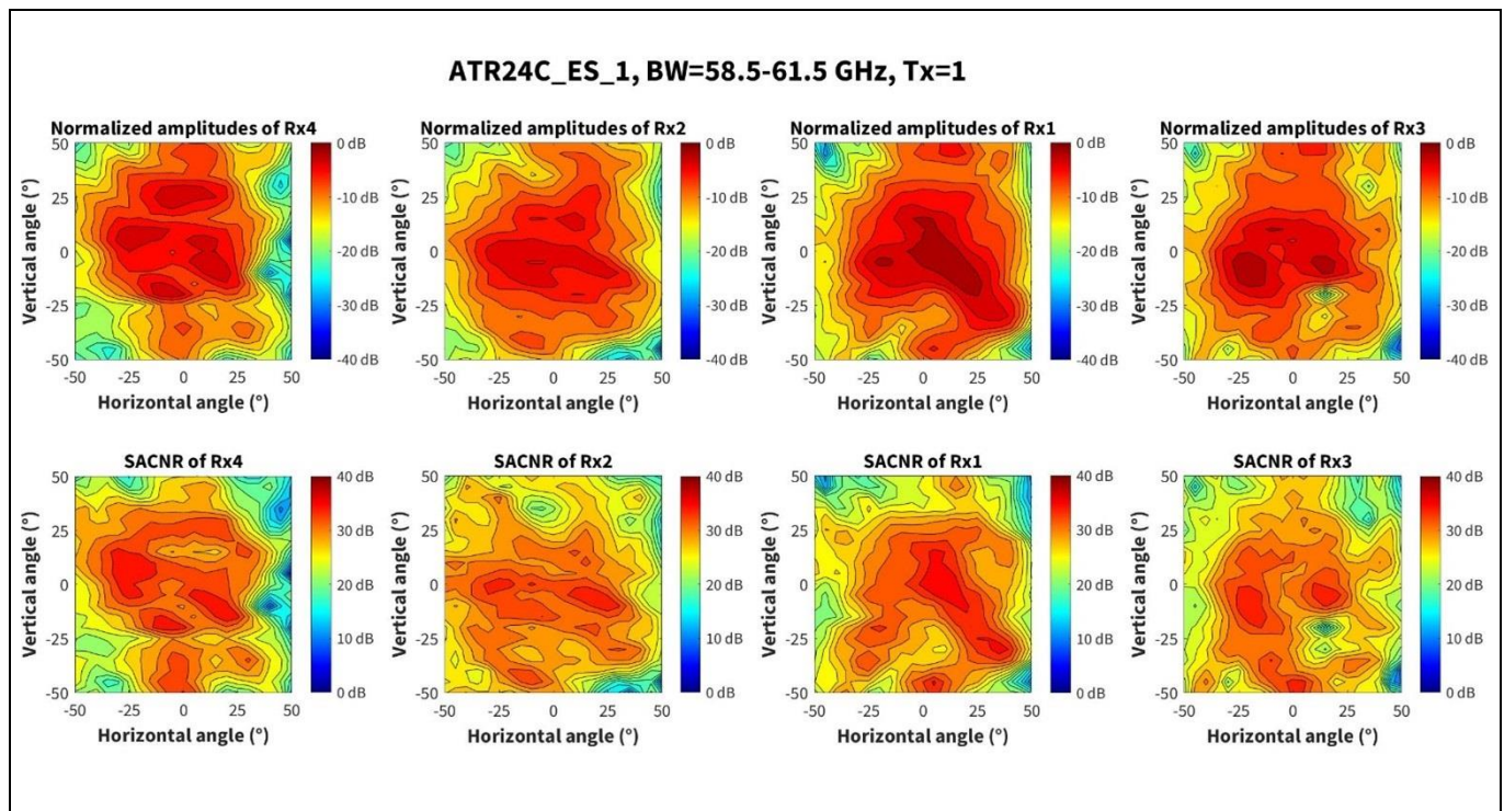
Figure 12 Amplitude and SACNR characteristics with Tx1 channel for 58.5 to 61.5 GHz band
