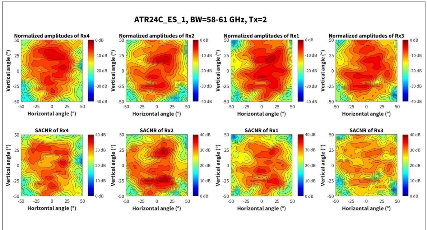
Figure 9 Amplitude and SACNR characteristics with Tx2 channel for 58 to 61 GHz band
