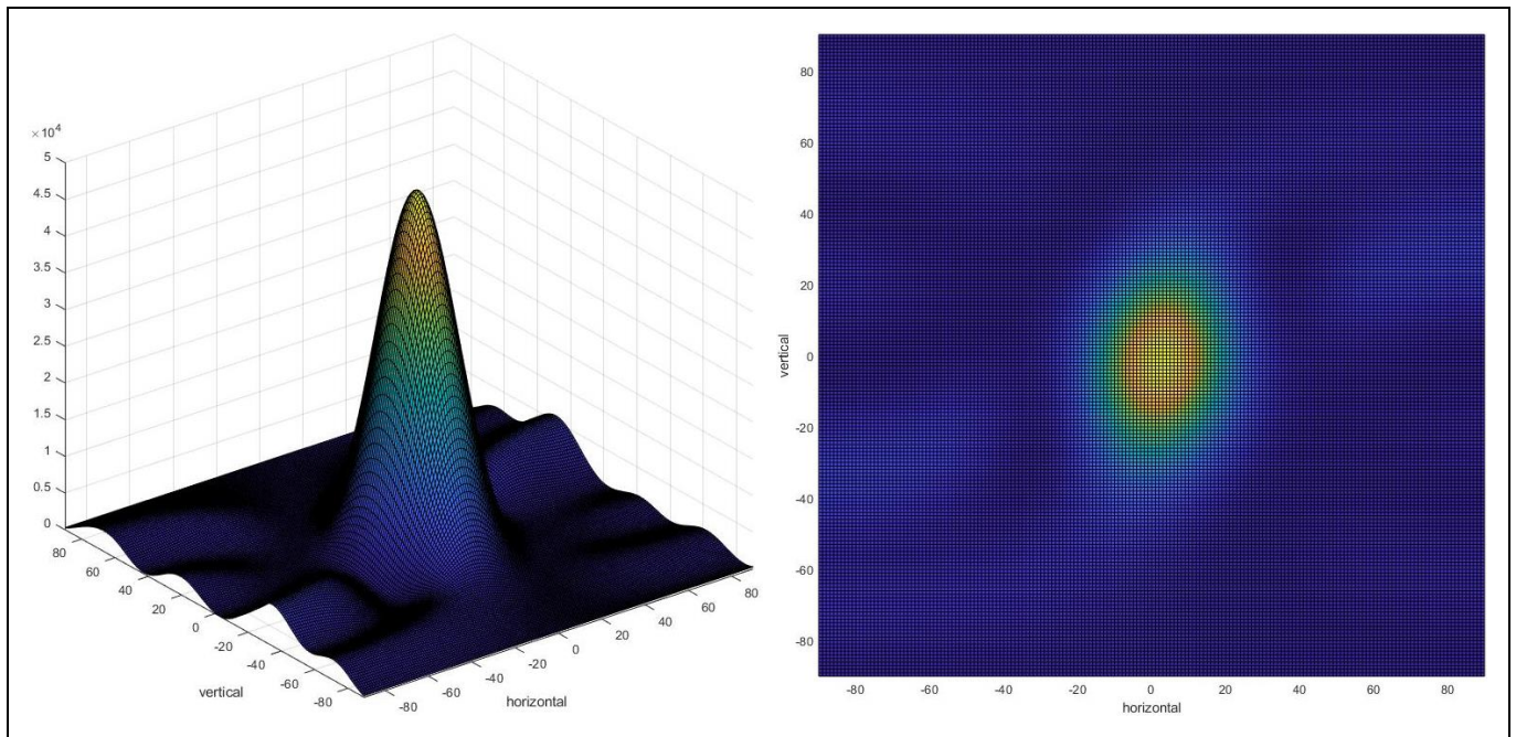
Figure 31 Angle spectrum after 2D beamforming for 0-degree azimuth and 0-degree elevation angle measurement
