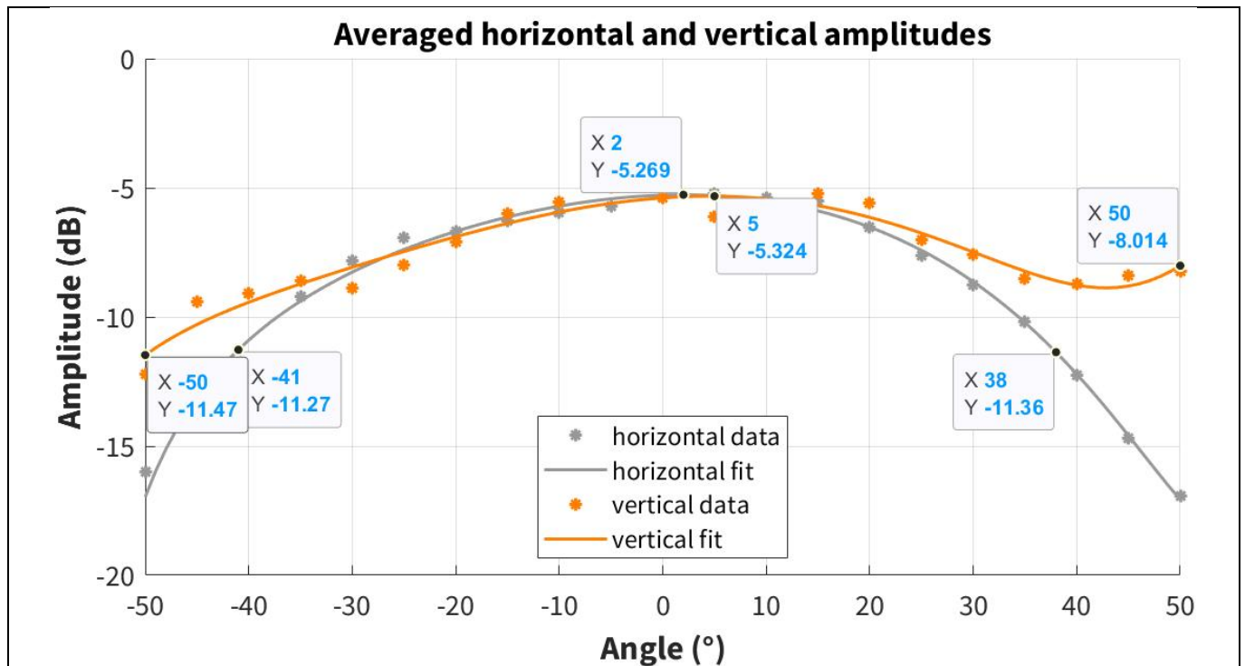
Figure 30 Averaged horizontal and vertical amplitudes and HPBW values for E-plane and H-plane
