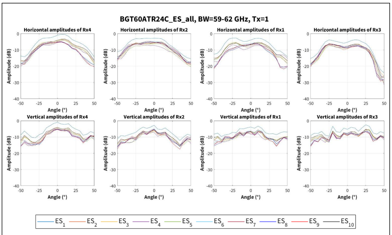
Figure 18 Amplitude characteristics on horizontal and vertical cross-sections with Tx1 channel for 59 to 62 GHz band for 10 boards
