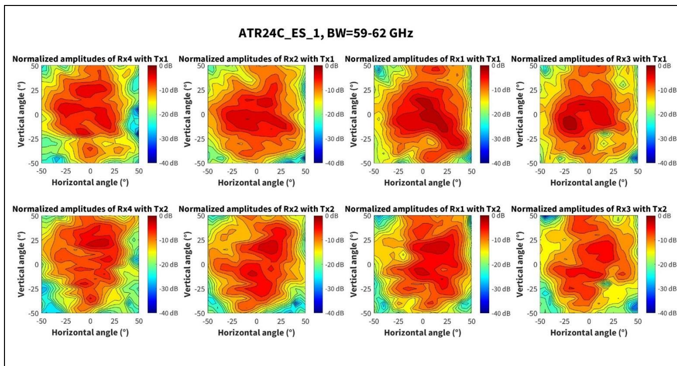
Figure 16 Amplitude characteristics of all virtual antennas for 59 to 62 GHz band
