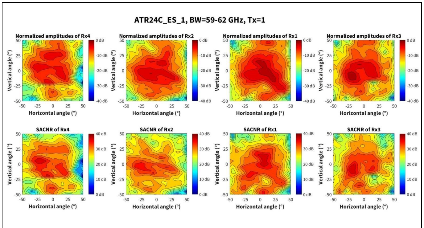
Figure 17 Amplitude and SACNR characteristics with Tx1 channel for 59 to 62 GHz band
