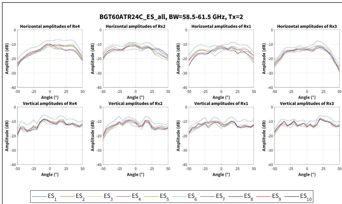
Figure 15 Amplitude characteristics on horizontal and vertical cross-sections with Tx2 channel for 58.5 to 61.5 GHz band for 10 boards
