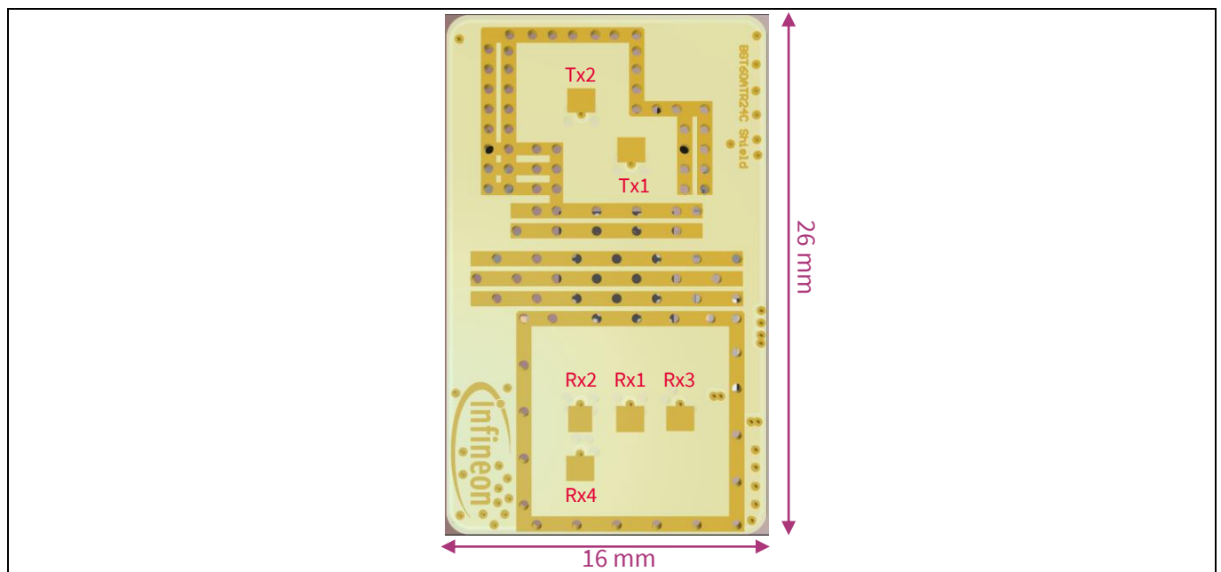
Figure 1 Antenna orientation and size of the BGT60ATR24C ES shield
