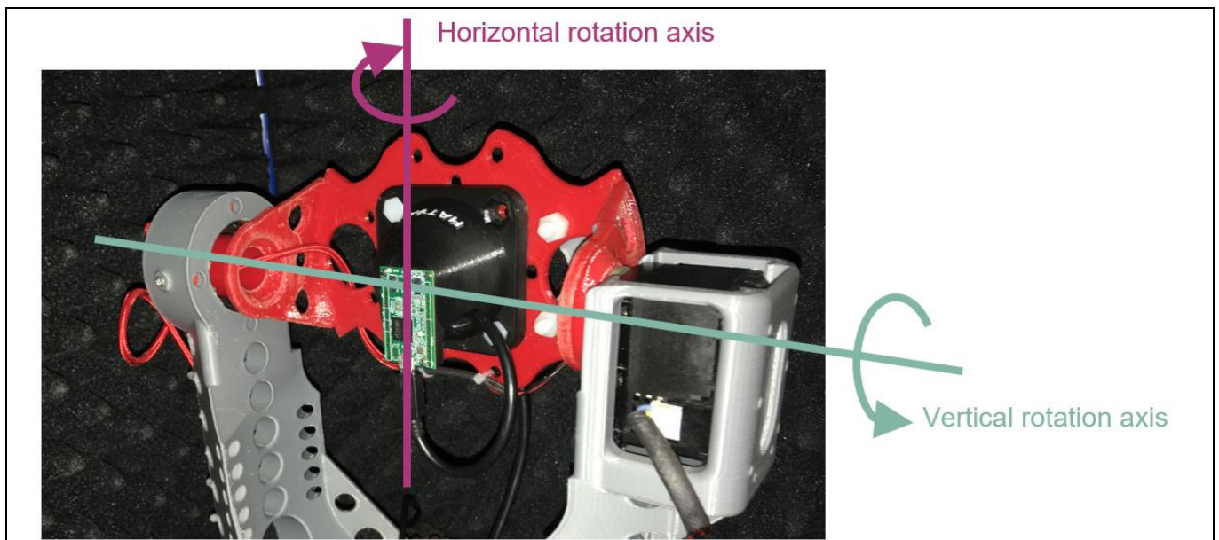
Figure 4 Antenna positioner (gimbal) for horizontal and vertical rotation of antennas
