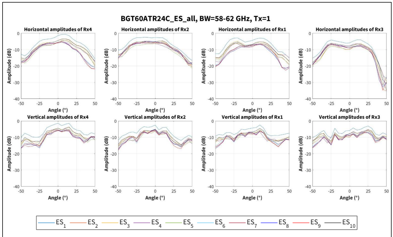
Figure 23 Amplitude characteristics on horizontal and vertical cross-sections with Tx1 channel for 58 to 62 GHz band for 10 boards
