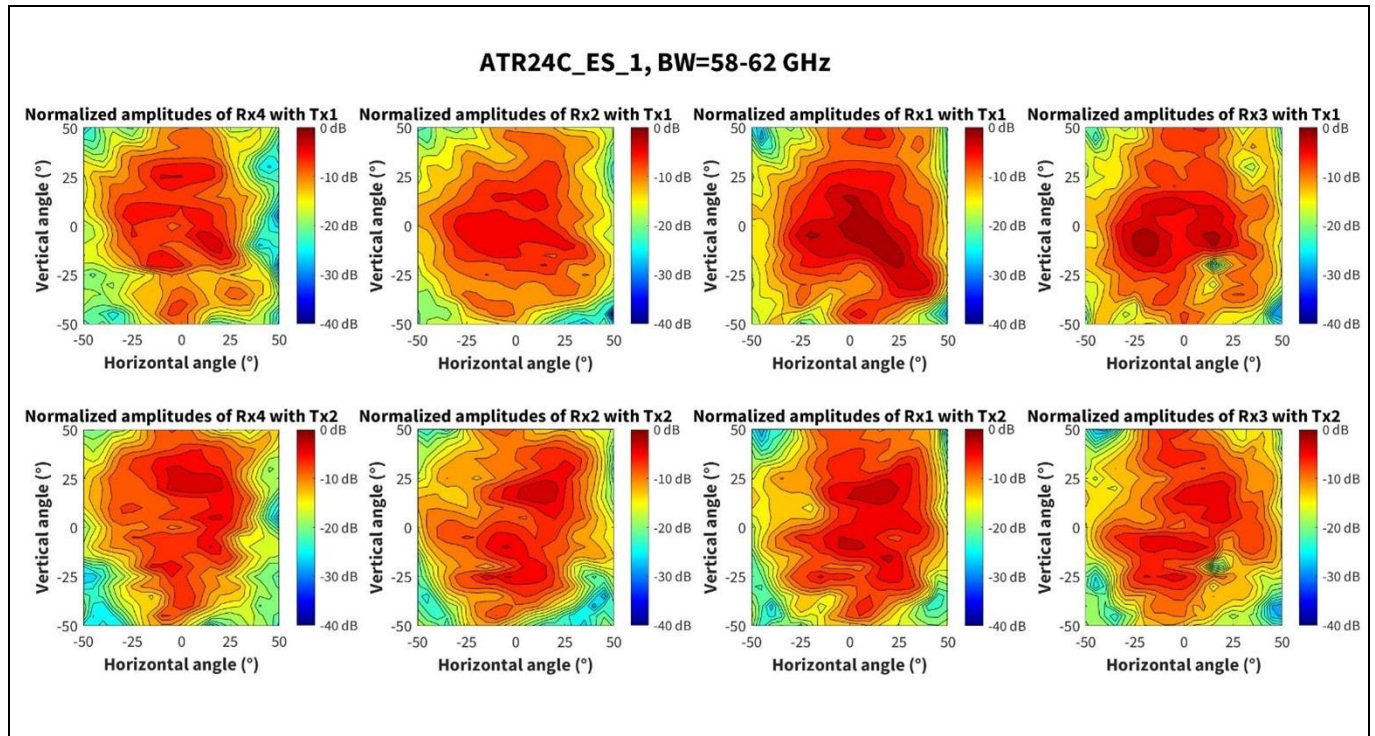
Figure 21 Amplitude characteristics of all virtual antennas for 58 to 62 GHz band
