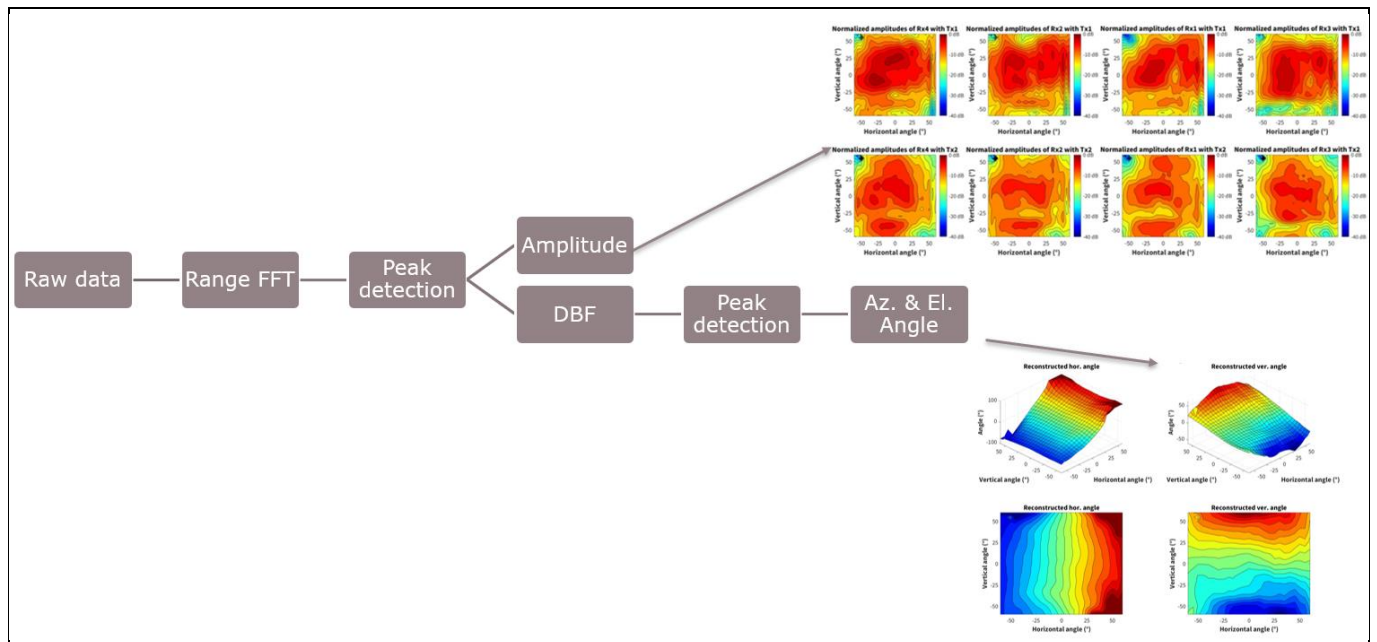
Figure 5 Characterization algorithm for amplitude and angle reconstruction
