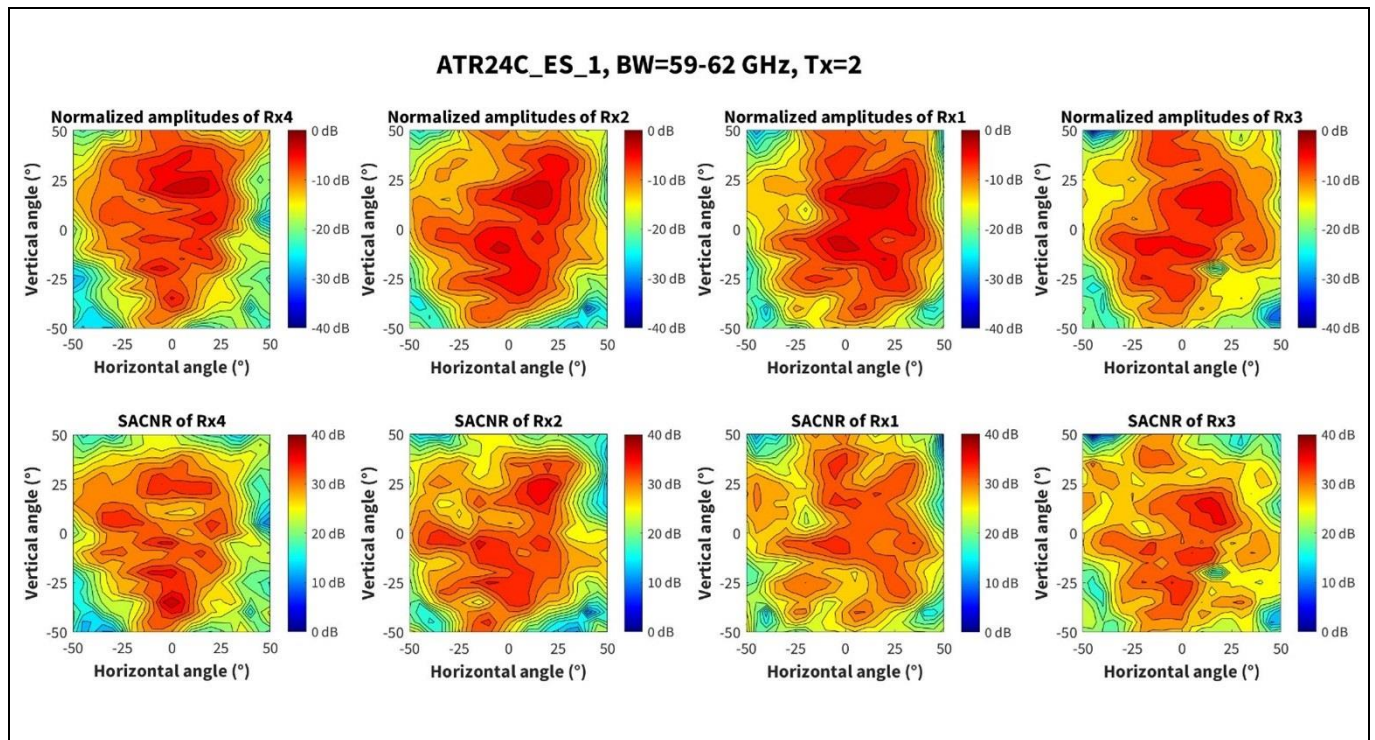
Figure 19 Amplitude and SACNR characteristics with Tx2 channel for 59 to 62 GHz band
