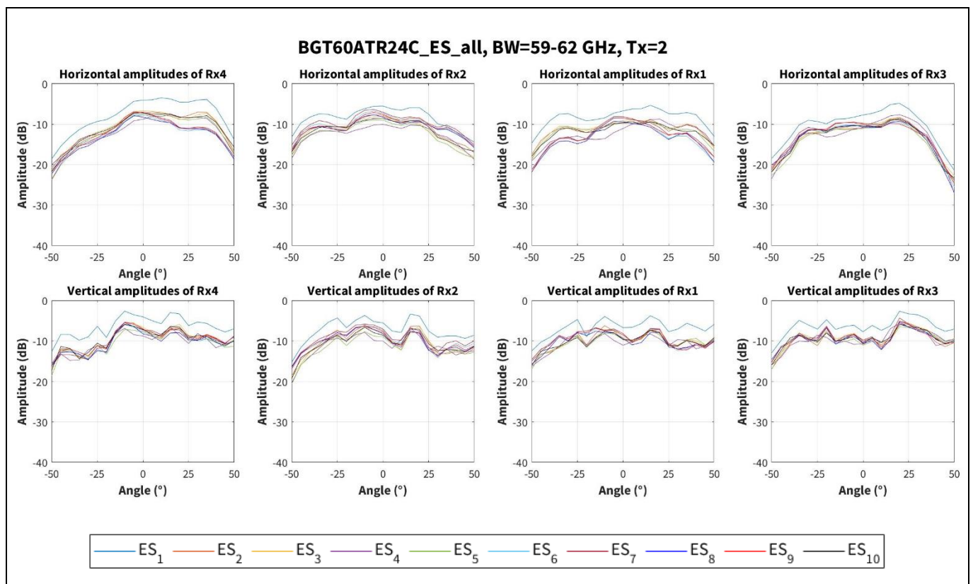
Figure 20 Amplitude characteristics on horizontal and vertical cross-sections with Tx2 channel for 59 to 62 GHz band for 10 boards
