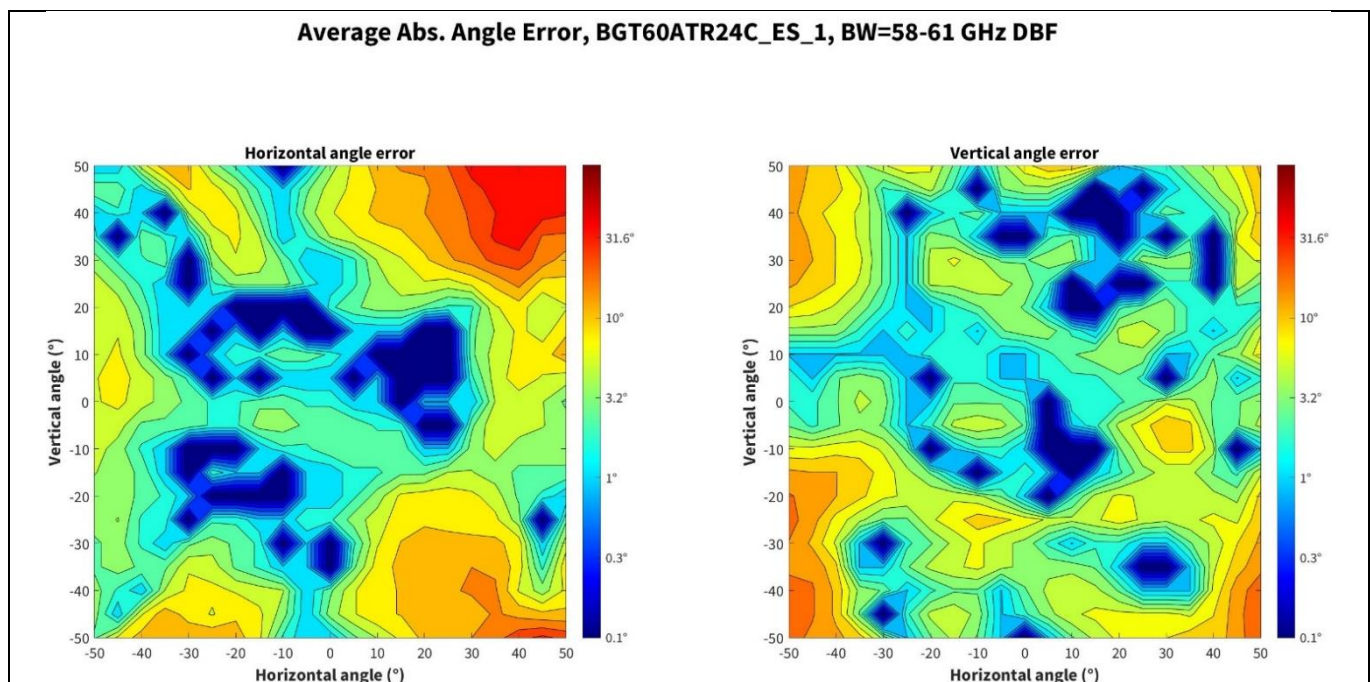
Figure 33 Angle reconstruction errors for 58 to 61 GHz measurements
