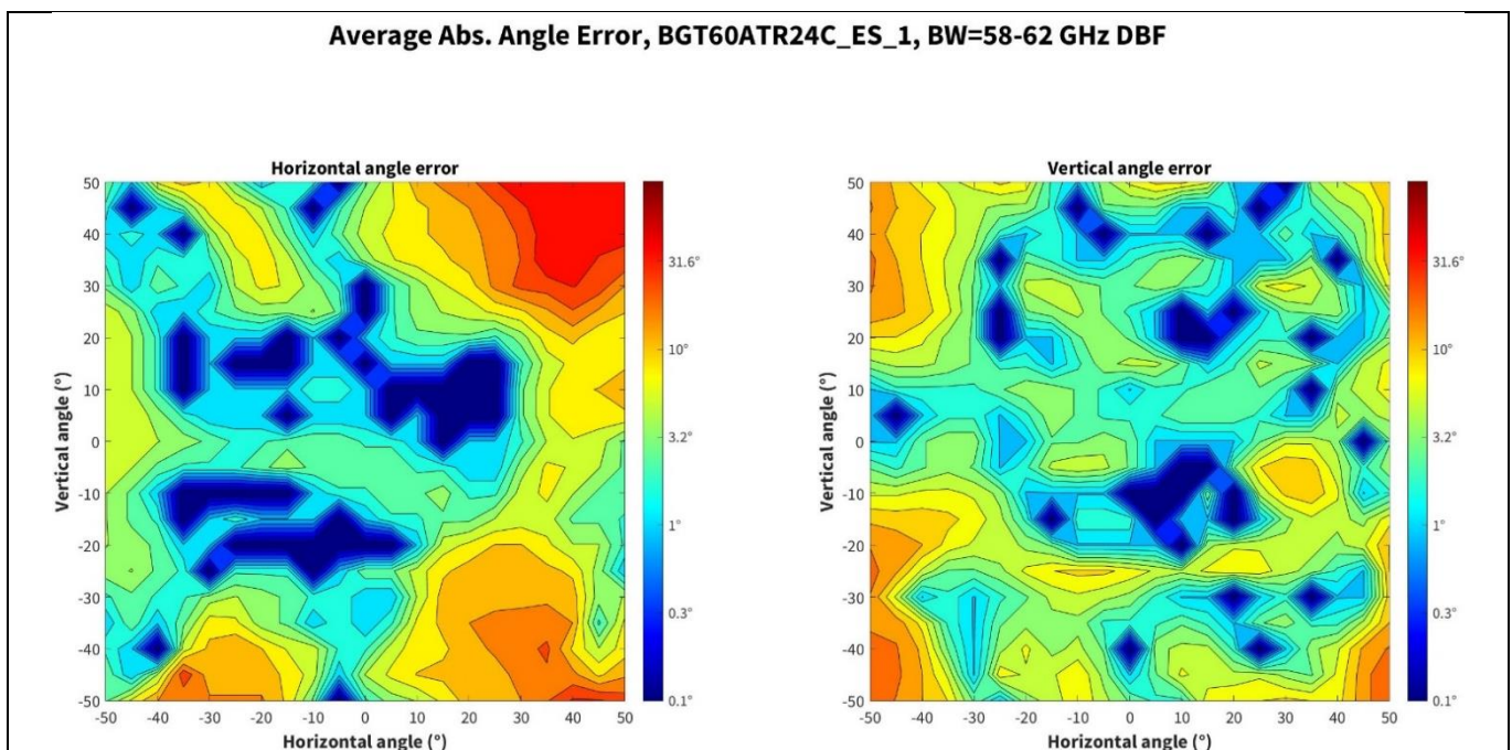
Figure 39 Angle reconstruction errors for 58 to 62 GHz measurements
