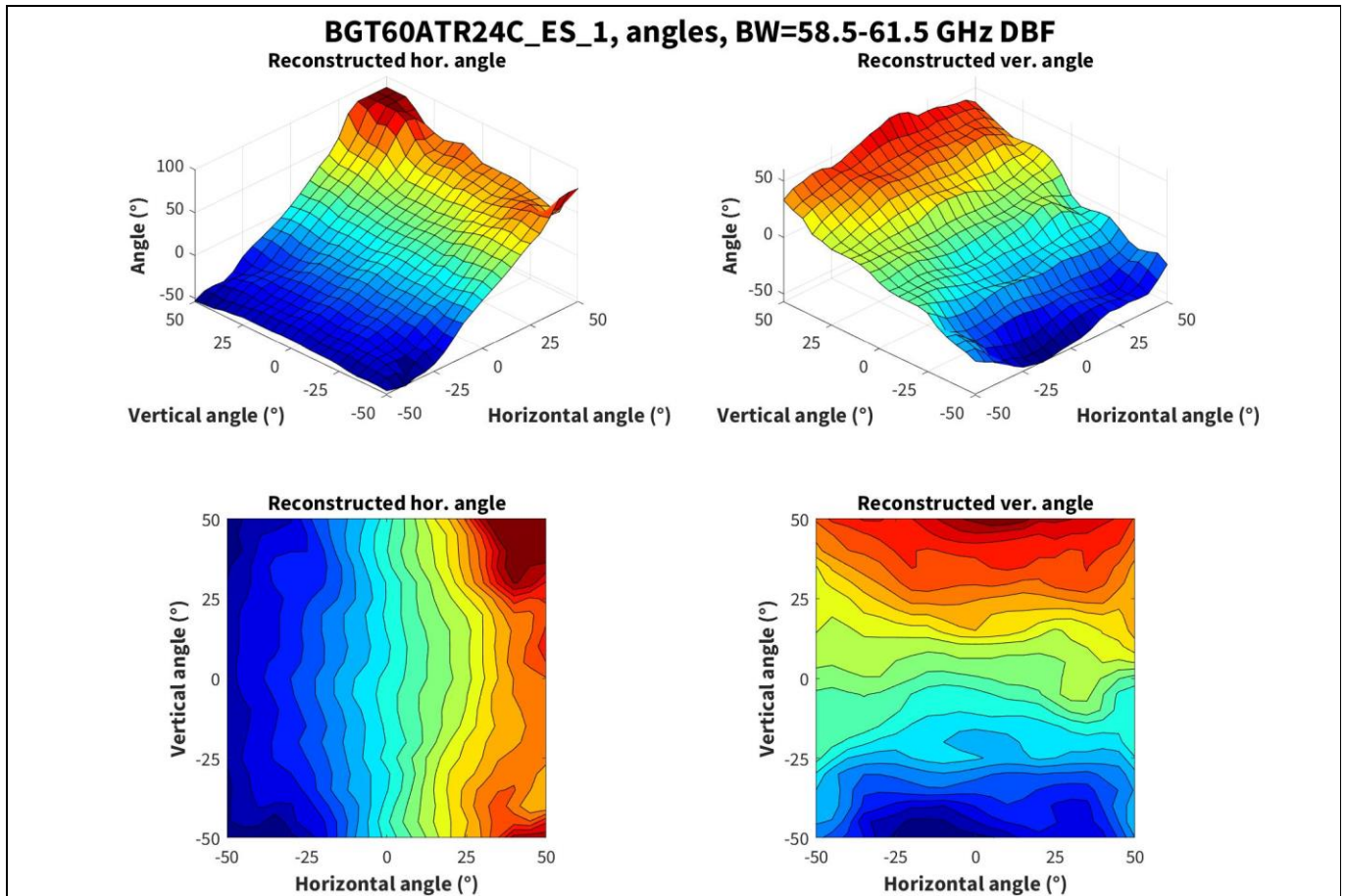
Figure 34 Reconstructed horizontal and vertical angles for 58.5 to 61.5 GHz measurements
