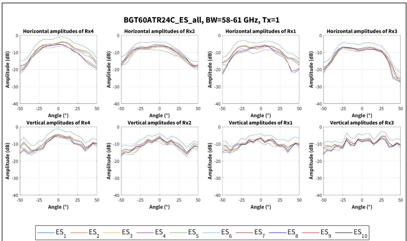
Figure 8 Amplitude characteristics on horizontal and vertical cross-sections with Tx1 channel for 58 to 61 GHz band for 10 boards
