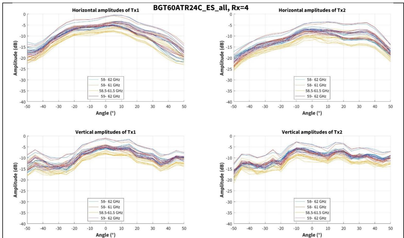
Figure 29 Amplitude characteristics on horizontal and vertical cross-sections with Rx4 channel for all frequency bands and 10 boards
