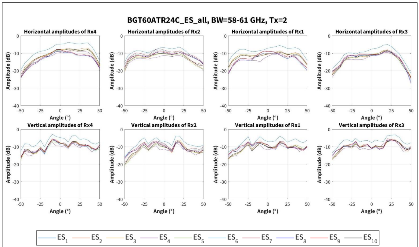
Figure 10 Amplitude characteristics on horizontal and vertical cross-section with Tx2 channel for 58 to 61 GHz band for 10 boards
