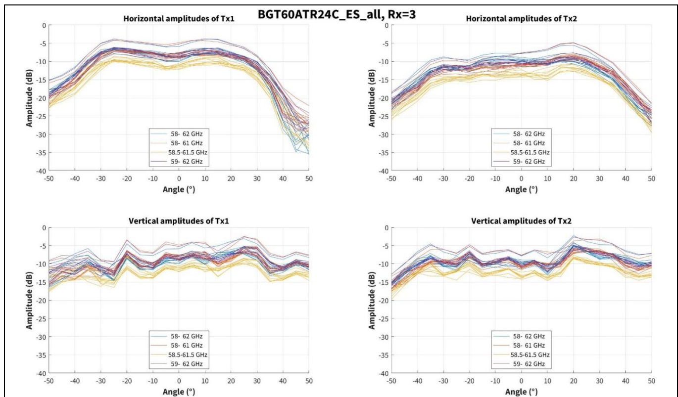
Figure 28 Amplitude characteristics on horizontal and vertical cross-sections with Rx3 channel for all frequency bands and 10 boards
