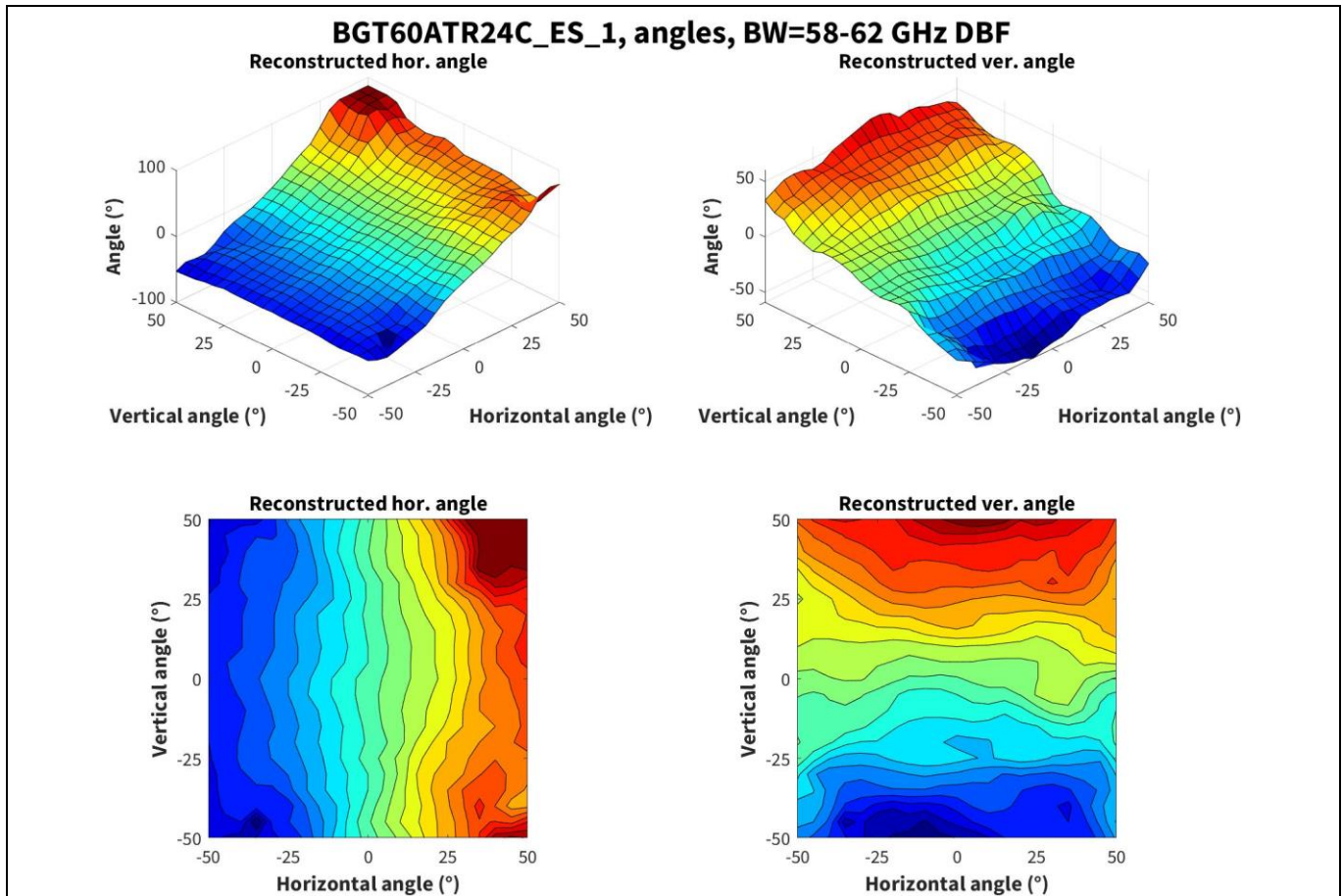
Figure 38 Reconstructed horizontal and vertical angles for 58 to 62 GHz measurements
