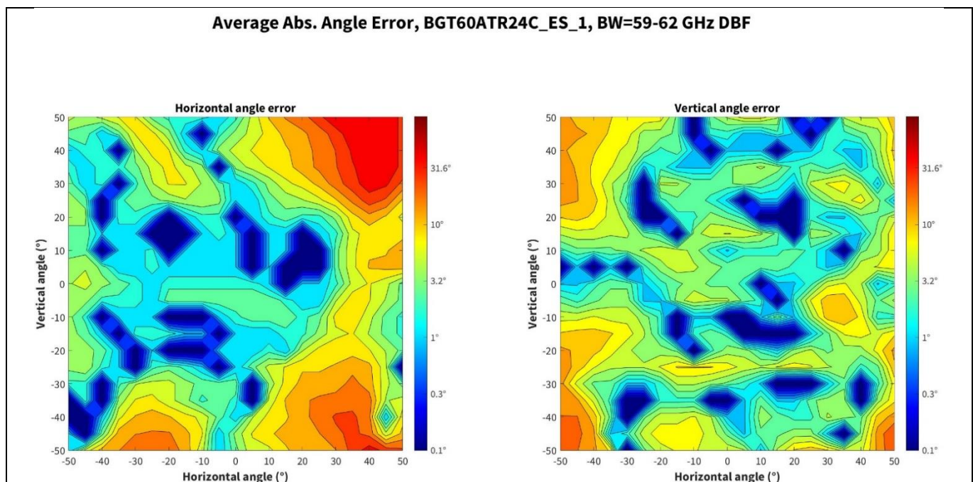
Figure 37 Angle reconstruction errors for 59 to 62 GHz measurements
