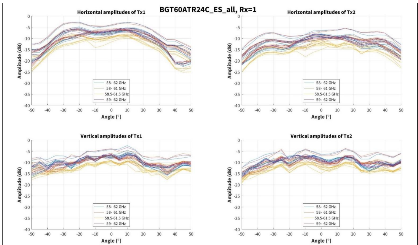
Figure 26 Amplitude characteristics on horizontal and vertical cross-sections with Rx1 channel for all frequency bands and 10 boards
