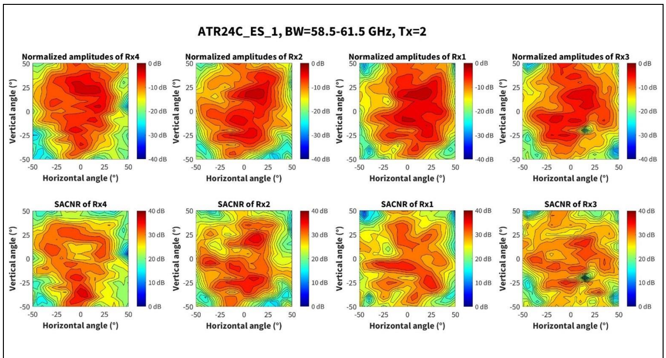
Figure 14 Amplitude and SACNR characteristics with Tx2 channel for 58.5 to 61.5 GHz band
