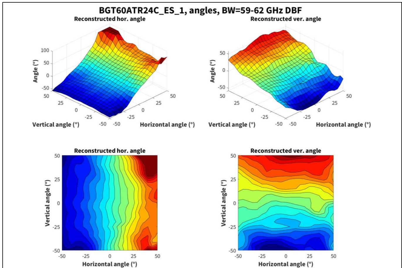
Figure 36 Reconstructed horizontal and vertical angles for 59 to 62 GHz measurements
