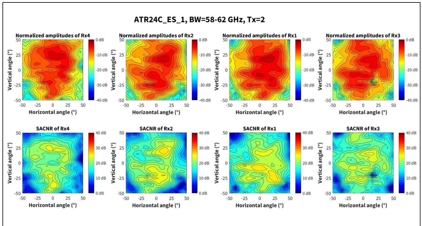
Figure 24 Amplitude and SACNR characteristics with Tx2 channel for 58 to 62 GHz band
