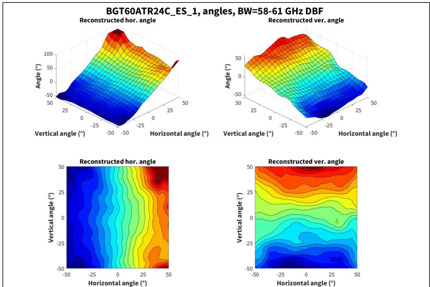
Figure 32 Reconstructed horizontal and vertical angles for 58 to 61 GHz measurements
