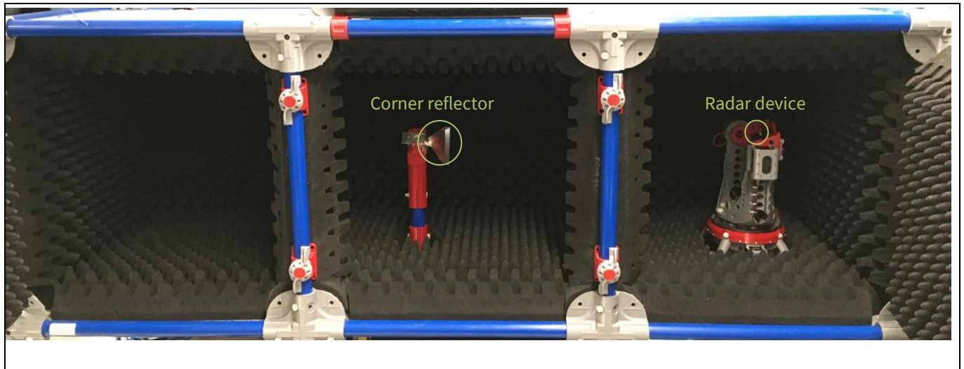
Figure 3 Anechoic antenna chamber used for the measurements
