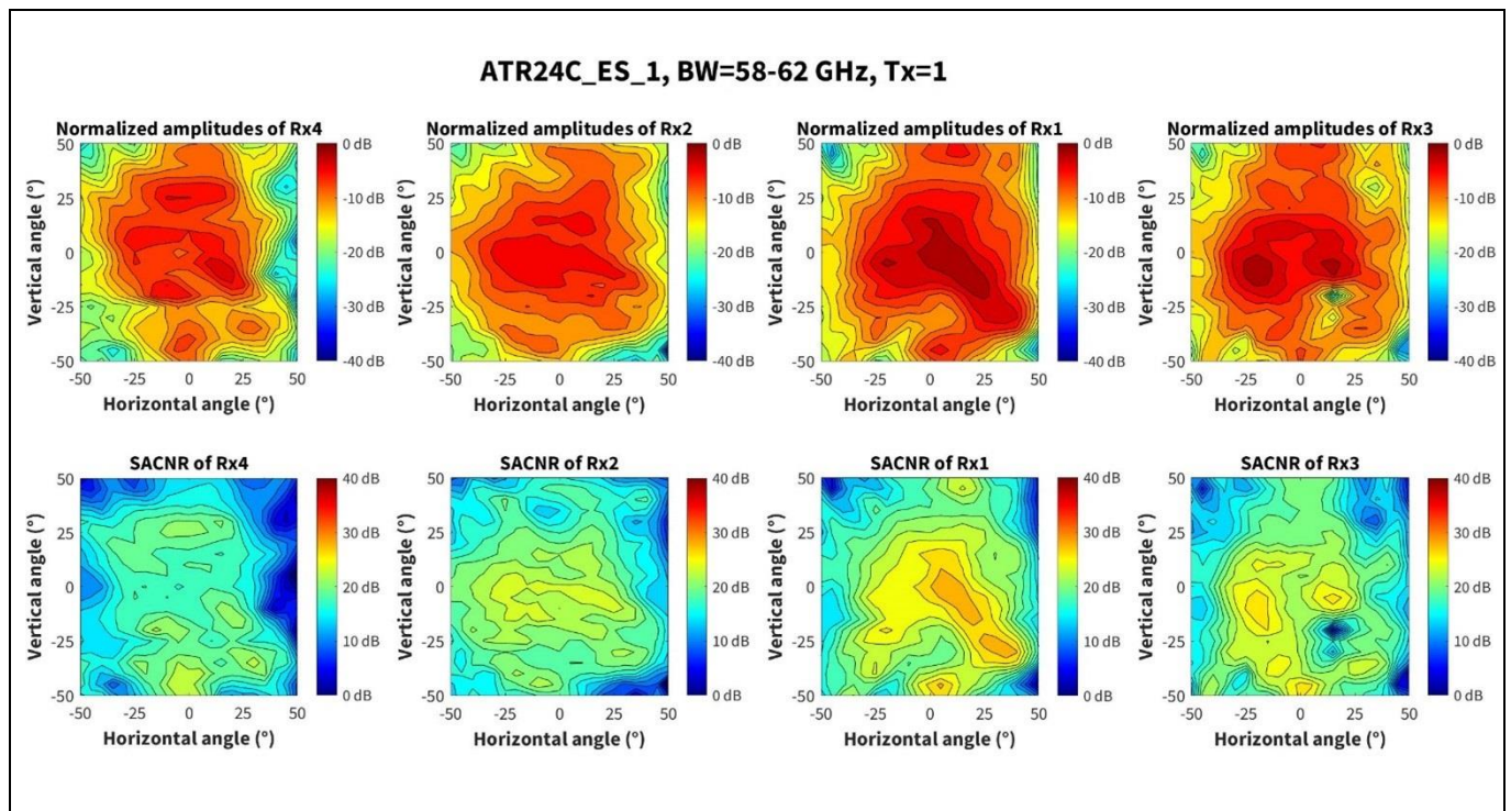
Figure 22 Amplitude and SACNR characteristics with Tx1 channel for 58 to 62 GHz band
