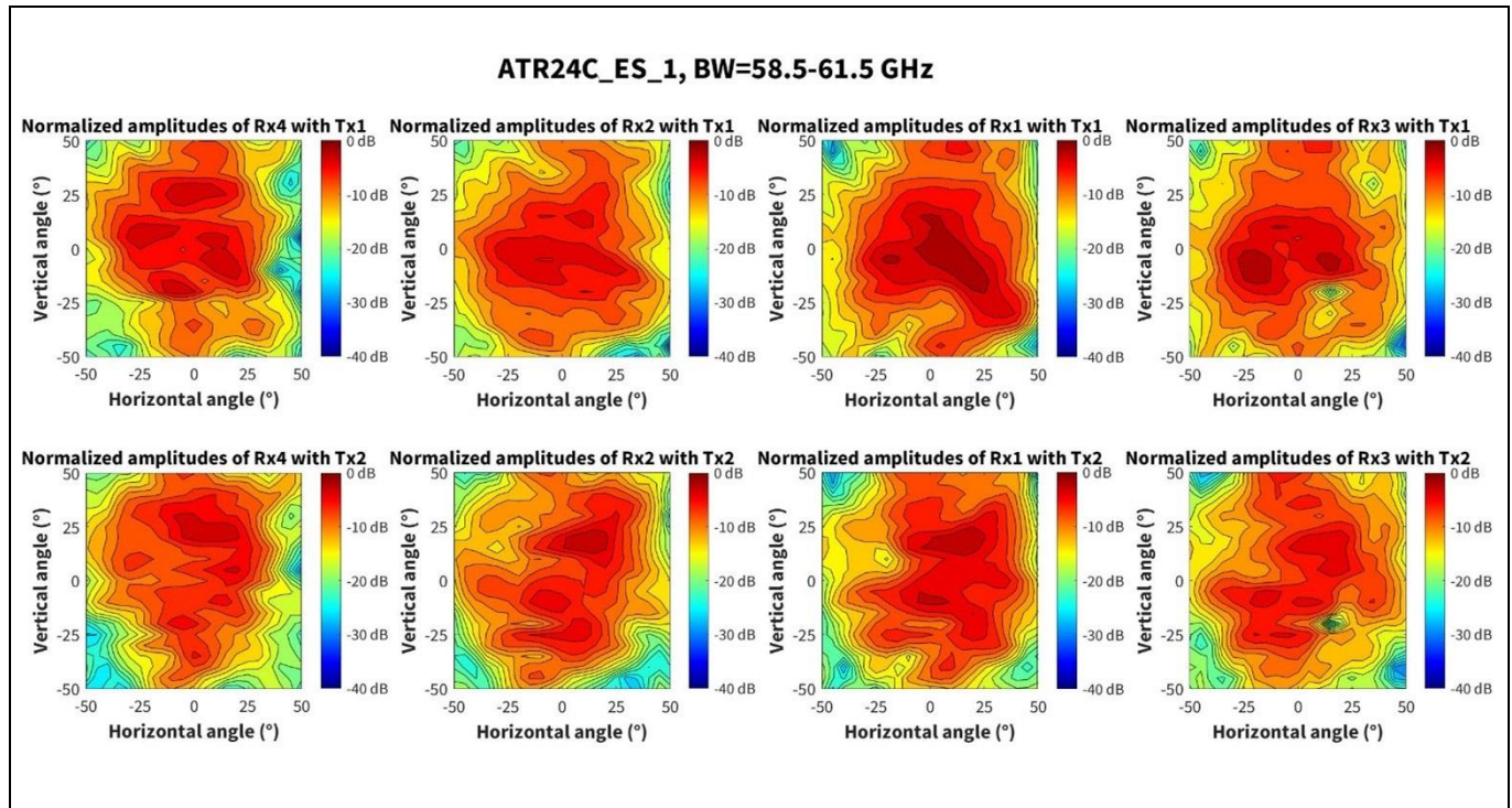
Figure 11 Amplitude characteristics of all virtual antennas for 58.5 to 61.5 GHz band
