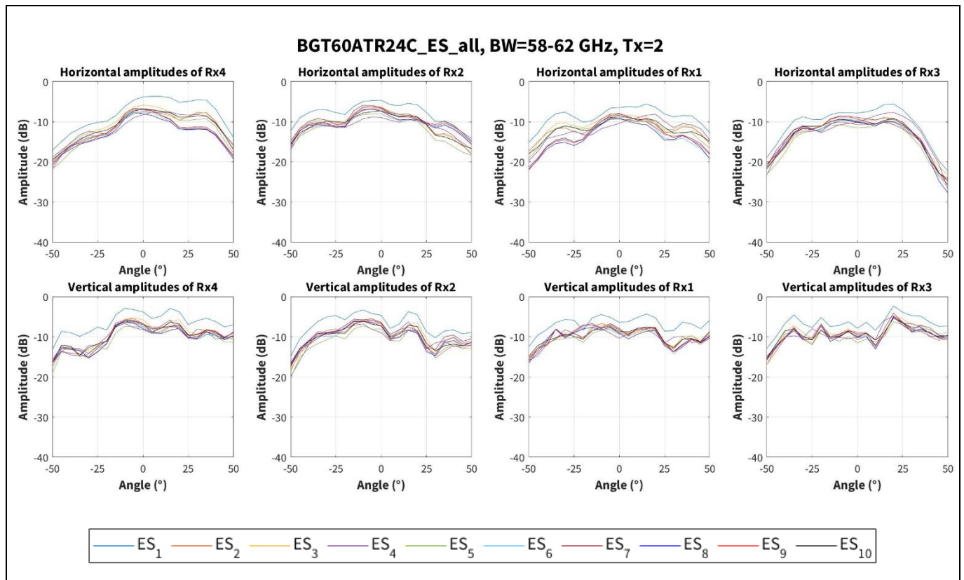
Figure 25 Amplitude characteristics on horizontal and vertical cross-sections with Tx2 channel for 58 to 62 GHz band for 10 boards
