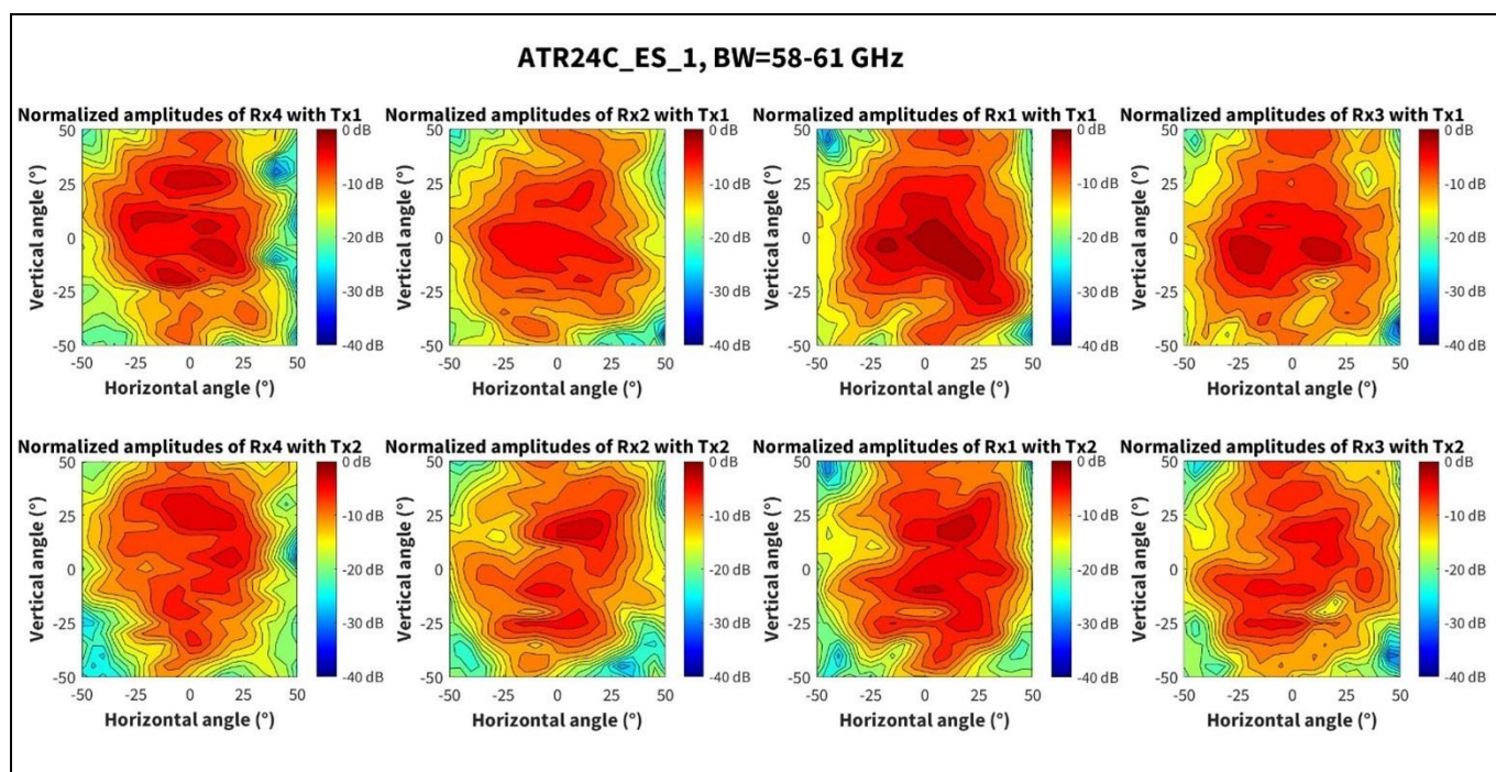
Figure 6 Amplitude characteristics of all virtual antennas for 58 to 61 GHz band
