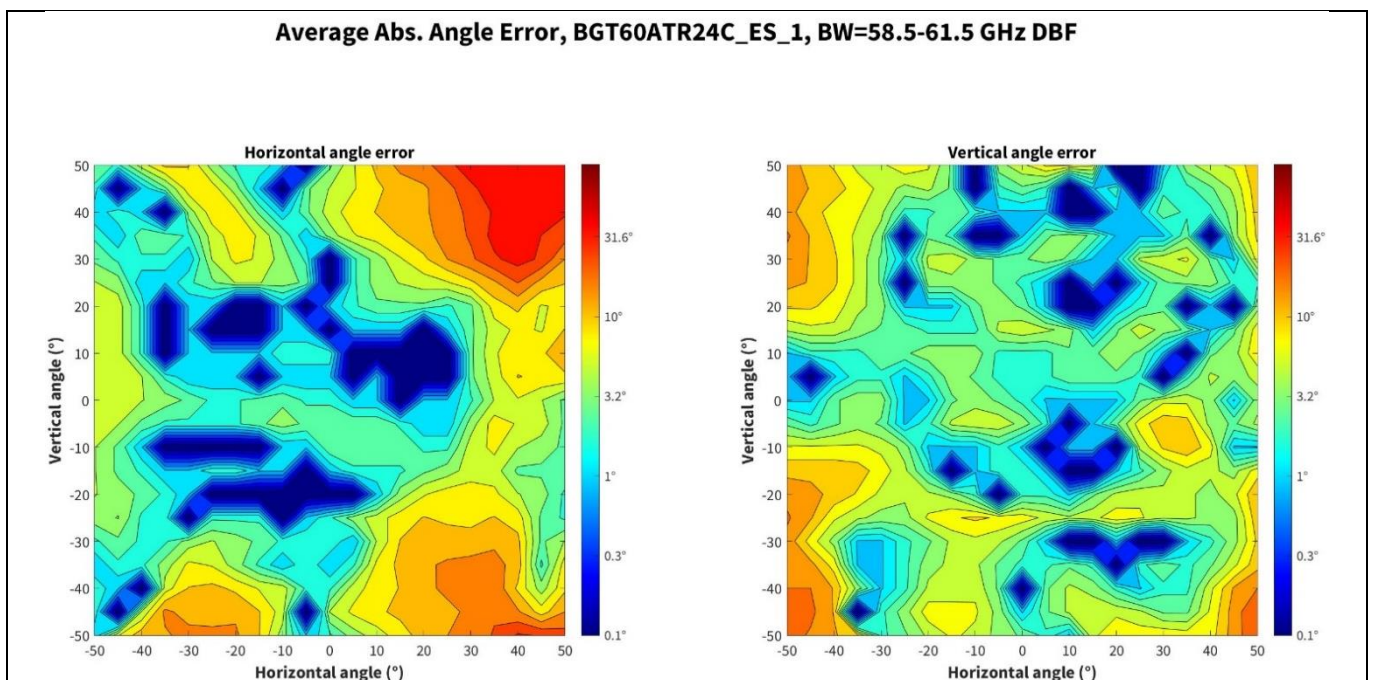
Figure 35 Angle reconstruction errors for 58.5 to 61.5 GHz measurements
