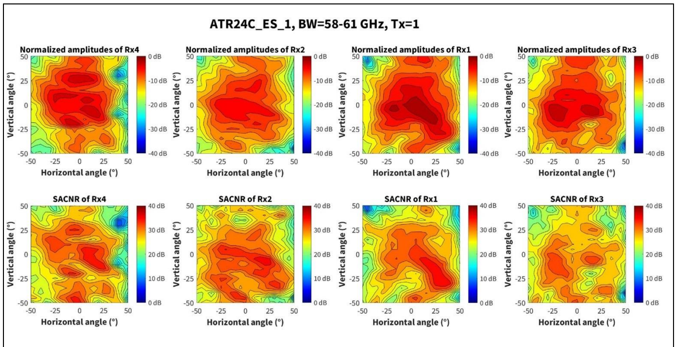
Figure 7 Amplitude and SACNR characteristics with Tx1 channel for 58 to 61 GHz band
