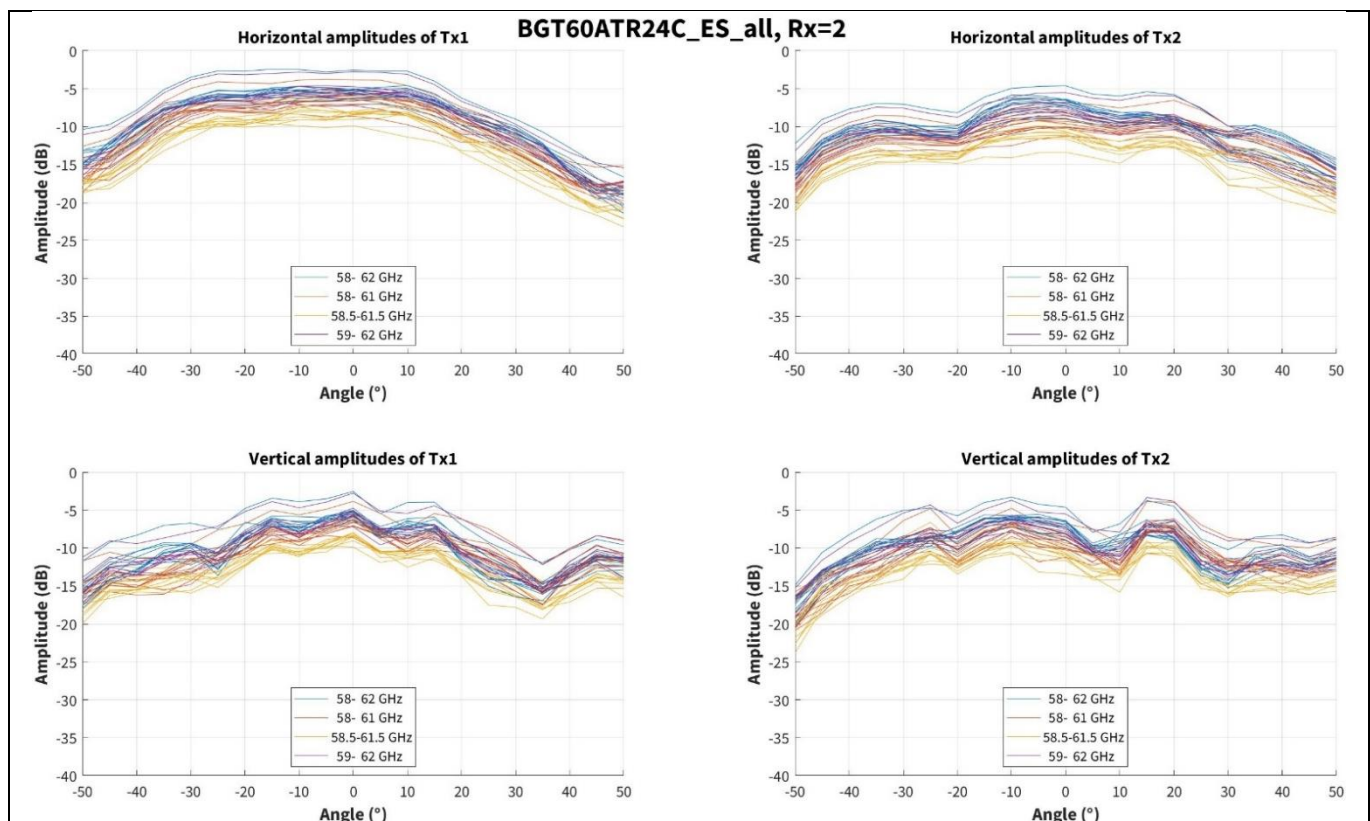
Figure 27 Amplitude characteristics on horizontal and vertical cross-sections with Rx2 channel for all frequency bands and 10 boards
