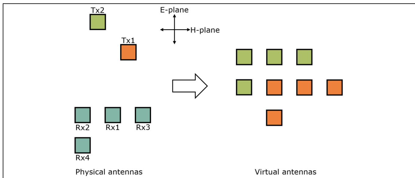
Figure 2 Orientation of the physical antennas and corresponding virtual antenna array
