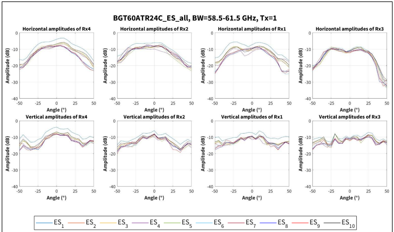
Figure 13 Amplitude characteristics on horizontal and vertical cross-sections with Tx1 channel for 58.5 to 61.5 GHz band for 10 boards
