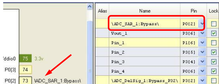
Figure 21. SAR ADC Reference Pin
