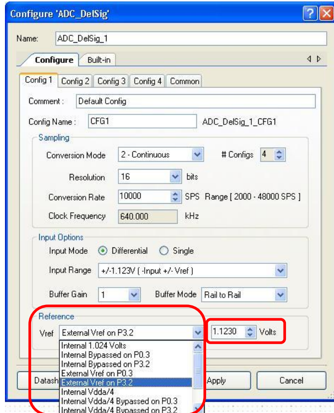
Figure 18. Delta-Sigma ADC Reference Selection
