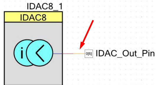
Figure 23. Schematic for Dedicated Iout
