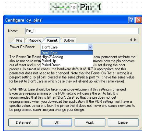
Figure 10. Pins Component Reset Setting
