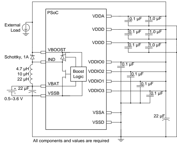
Figure 6. Boost Converter Typical Application
