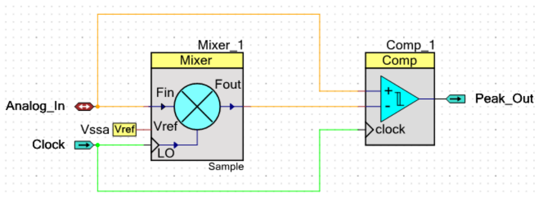
Figure 1. Peak Detector with Sample and Hold
