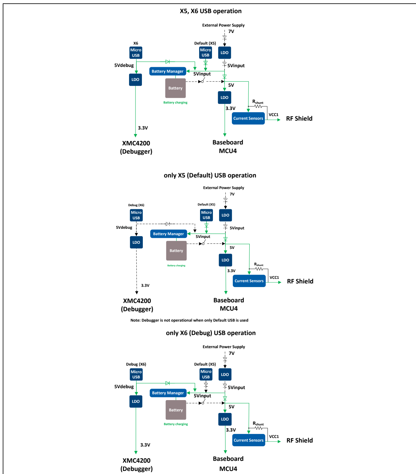
Figure 8 Operation with USB cables
