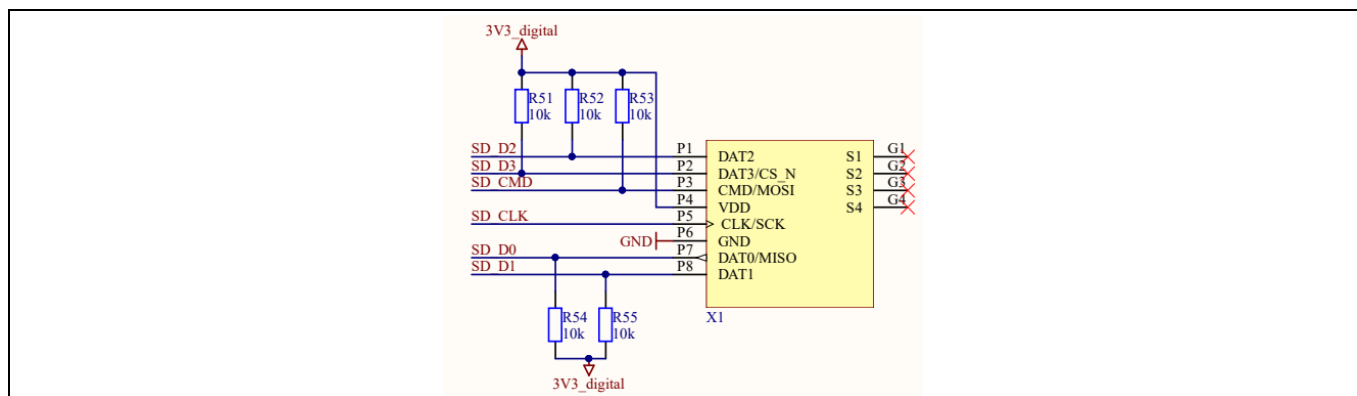
Figure 13 SD card reader connections
