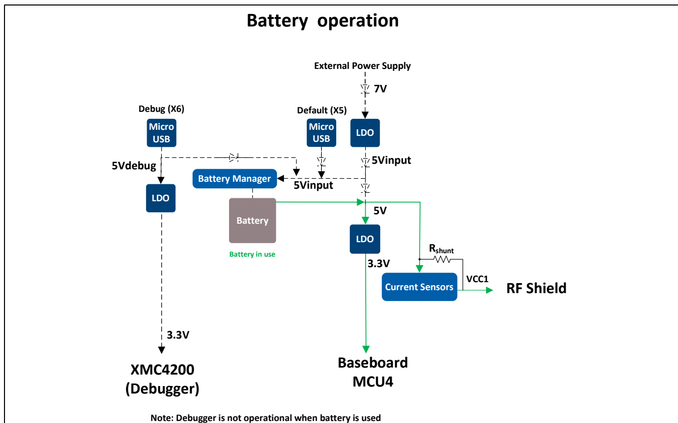
Figure 6 Battery operation block diagram
