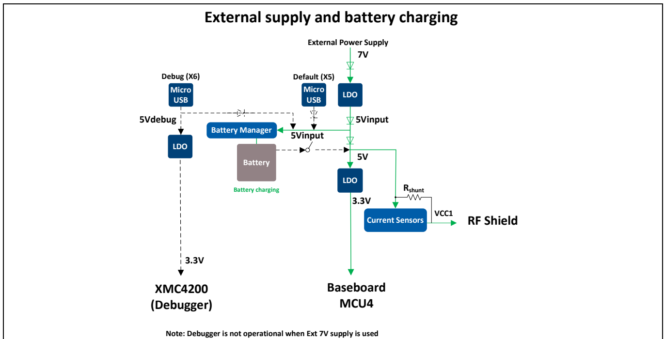
Figure 4 External power supply and battery charging block diagram
