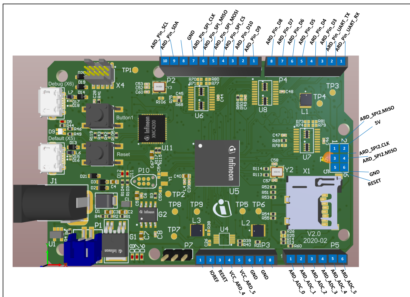
Figure 15 External headers (P2, P4, P5, and P6)
