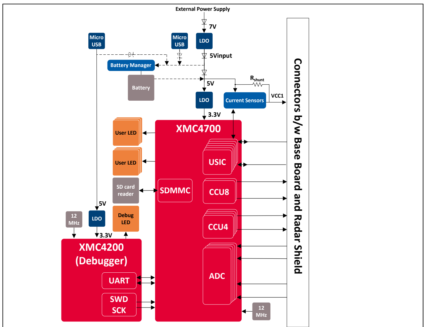
Figure 2 Radar Baseboard MCU4 block diagram
