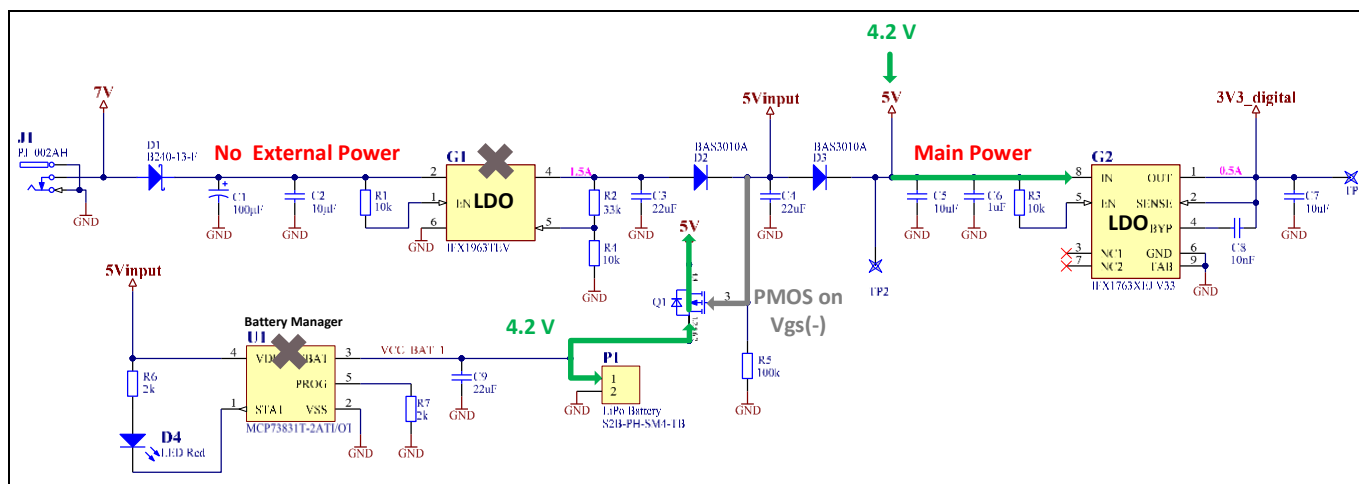
Figure 7 Battery operation schematic
