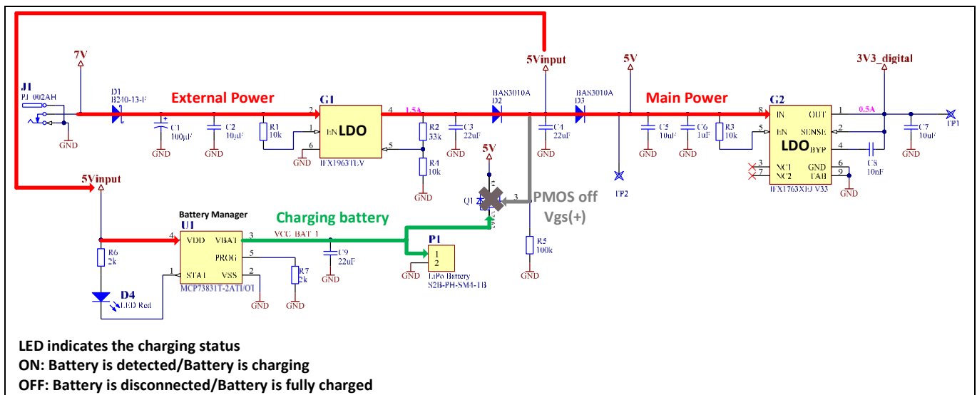
Figure 5 External power supply and battery charging schematic
