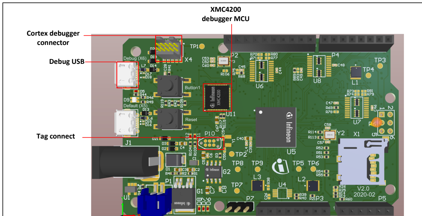
Figure 16 Debugger components
