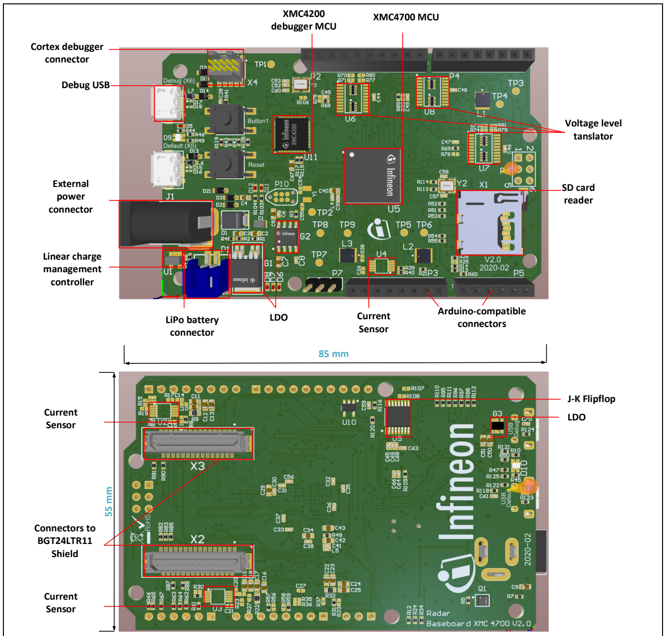
Figure 1 Radar Baseboard MCU4 with main component and dimensions
