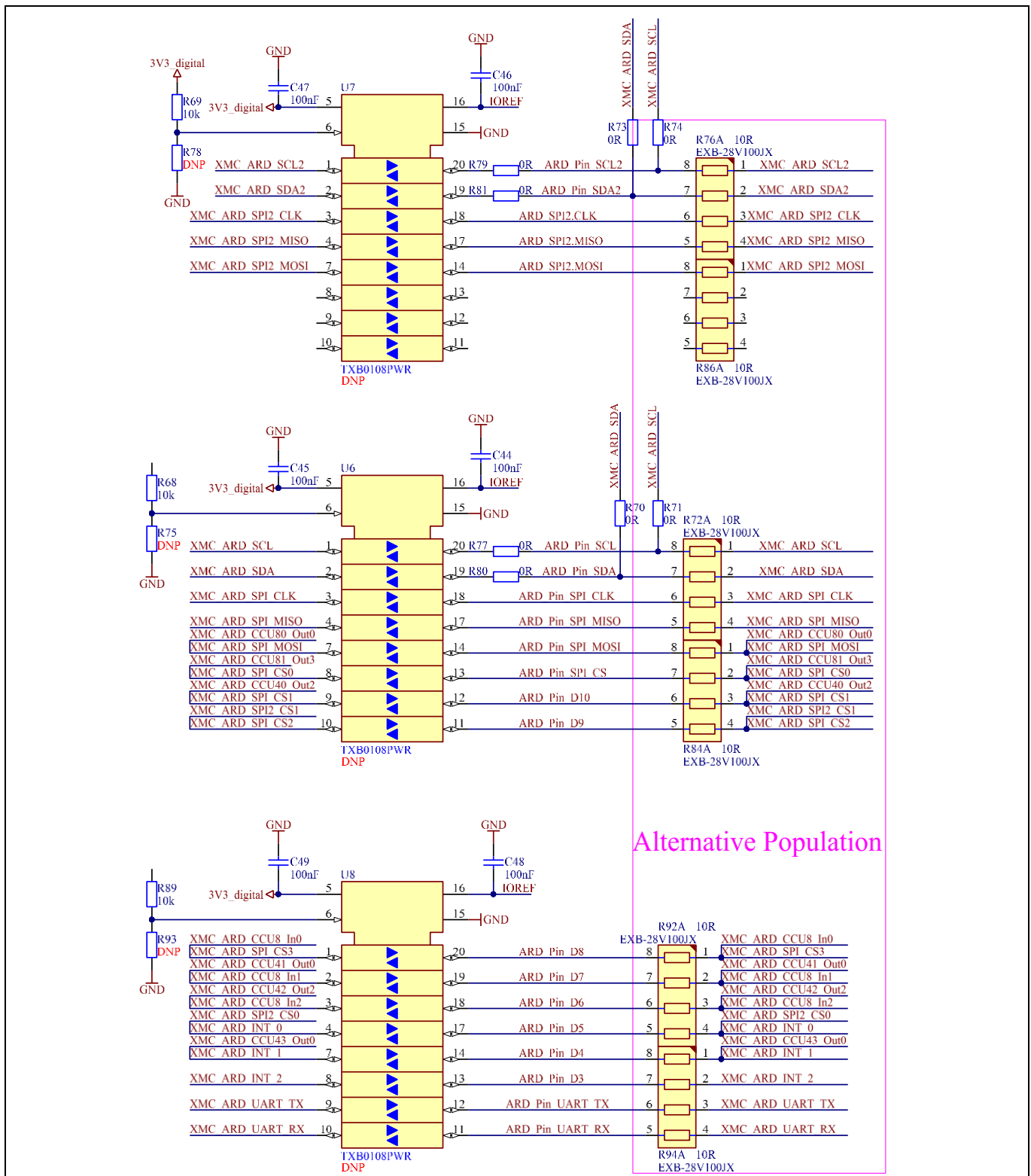
Figure 14 Level translator (U6, U7, and U8) connections
