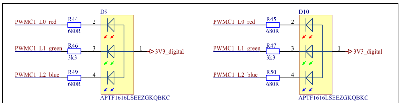
Figure 11 User-configurable LEDs
