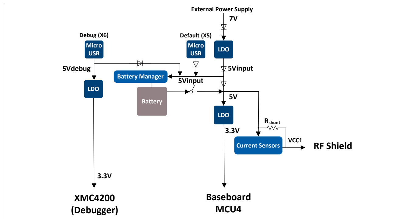
Figure 3 Power supply concept block diagram
