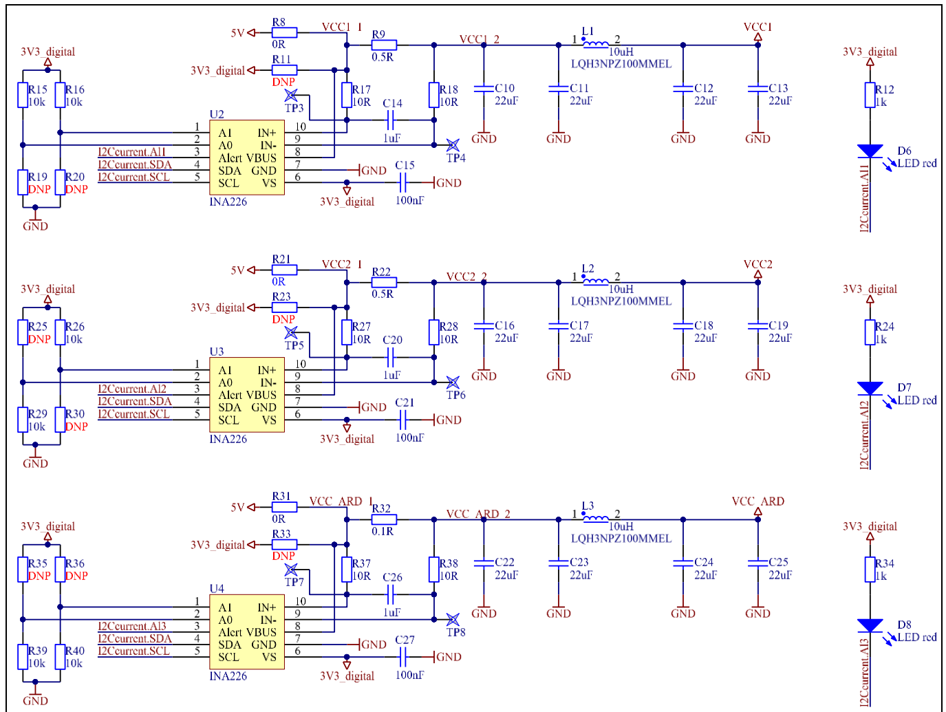
Figure 9 Current sensors connections
