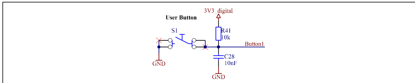
Figure 12 User-configurable button
