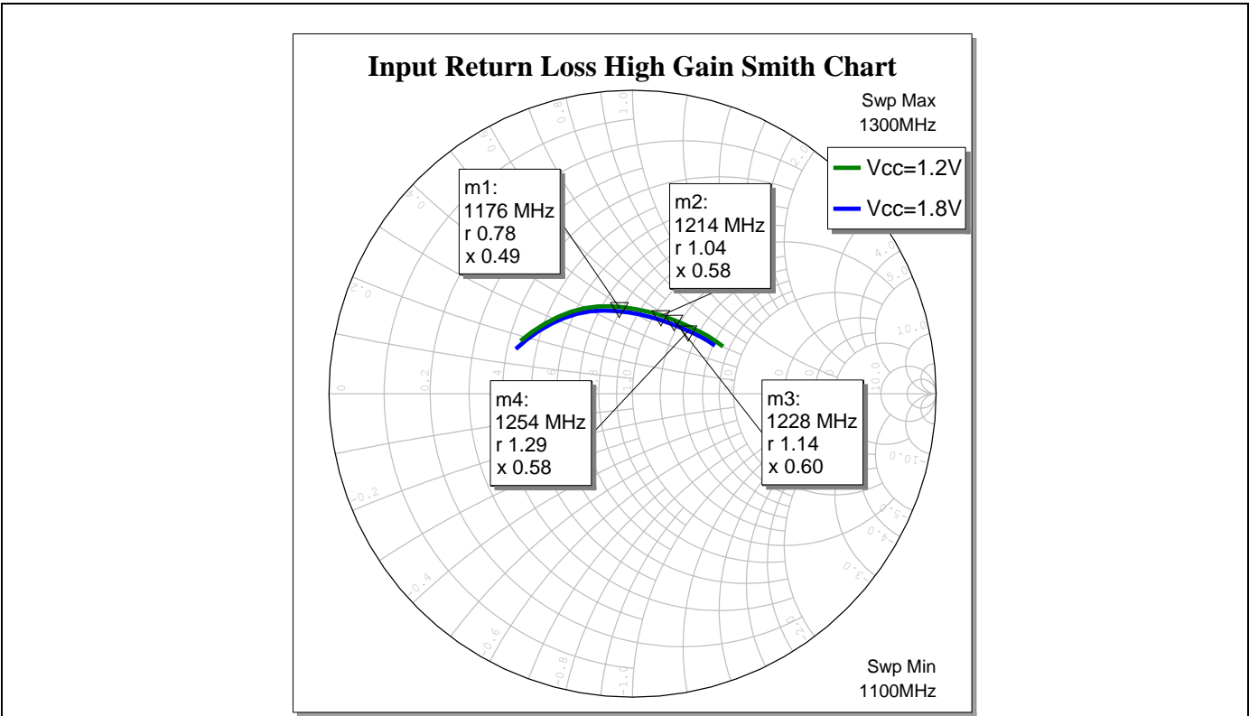
Figure 11 Input return loss (Smith chart) of BGA123L4 for GNSS applications (port de-embedded)
