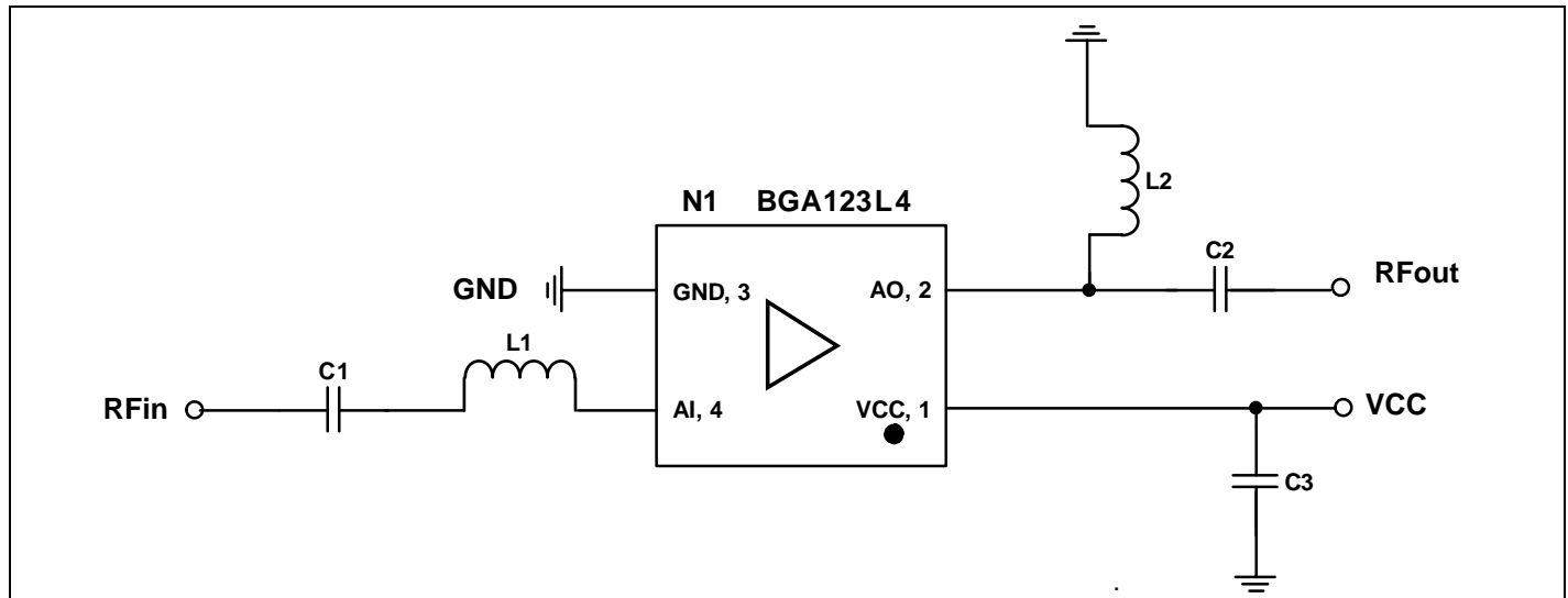
Figure 5 Schematic of the BGA123L4 application circuit
