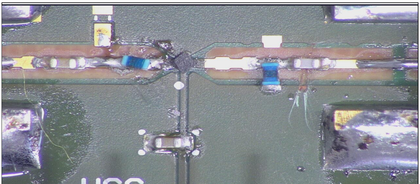
Figure 24 Photo of evaluation board (detailed view)
