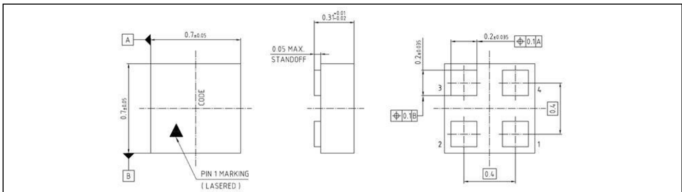
Figure 4 Package and pin connections of BGA123L4
