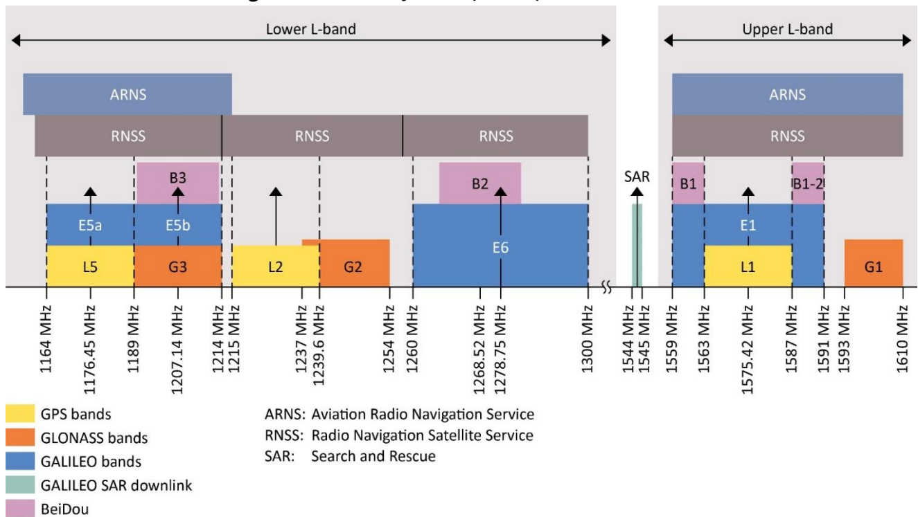
Figure 2 Frequency allocation: GNSS systems, upper L bands and lower L bands
