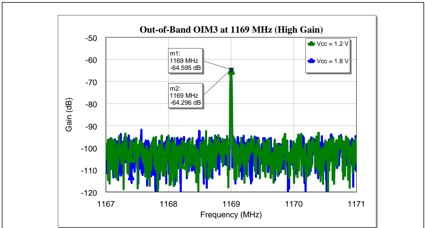
Figure 20 Out-of-band third-order intermodulation point of BGA123L4 for GNSS applications at 1169 MHz (output referred)
