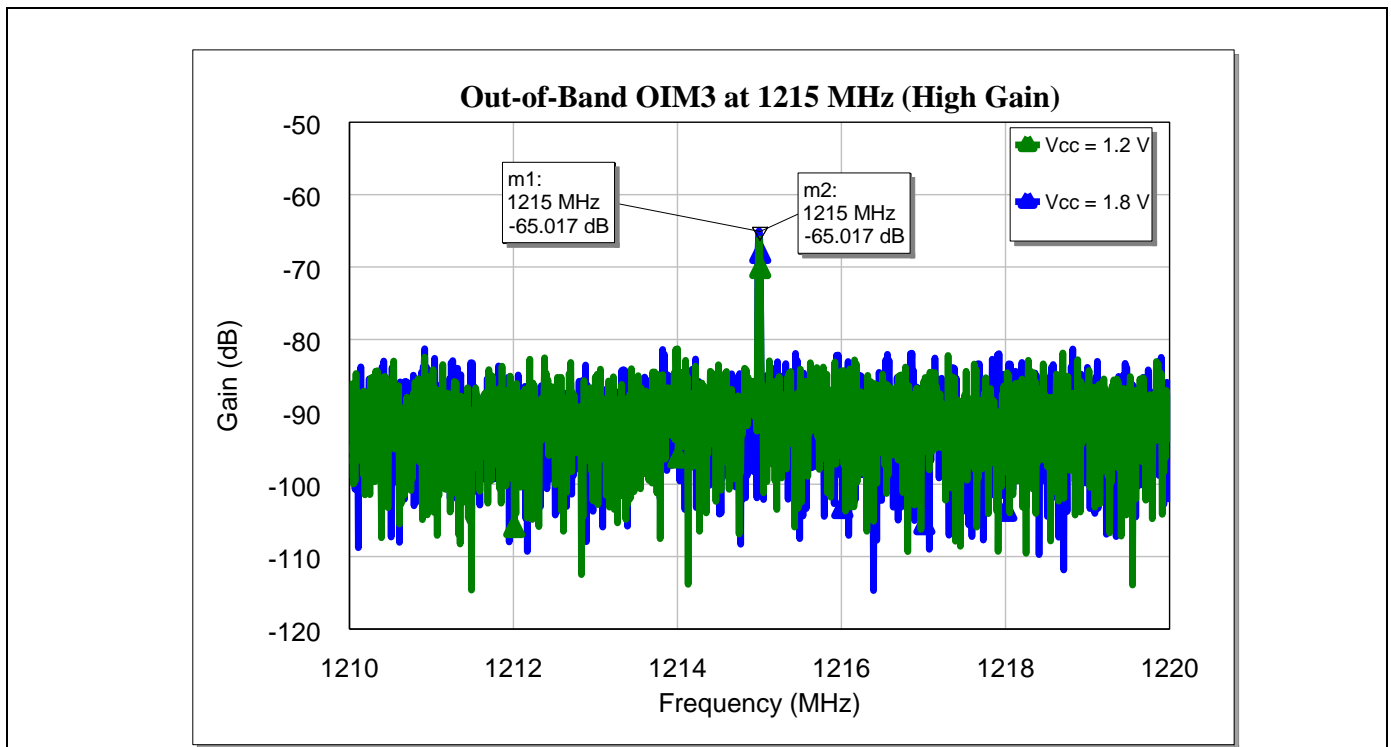
Figure 22 Out-of-band third-order intermodulation point of BGA123L4 for GNSS applications at 1215 MHz (output referred)
