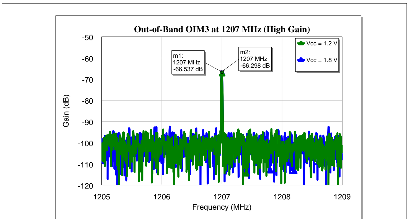
Figure 21 Out-of-band third-order intermodulation point of BGA123L4 for GNSS applications at 1207 MHz (output referred)
